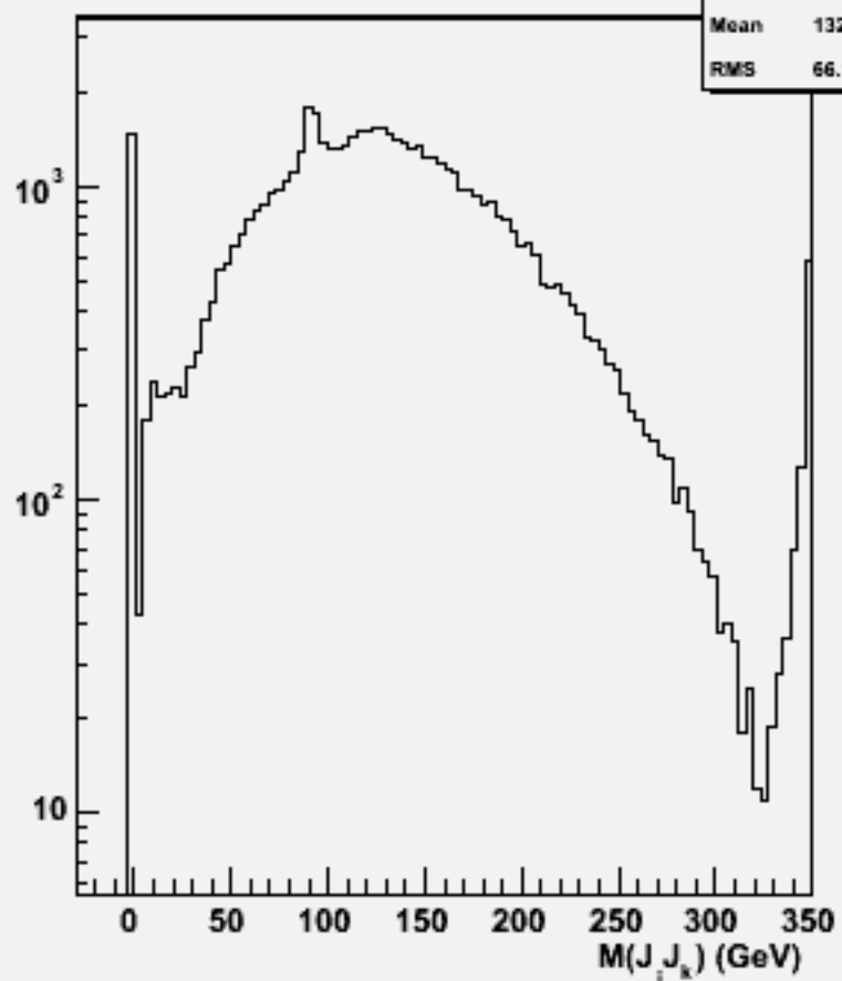
2jets mass(All comb)w102522 e1e1ddss_o
