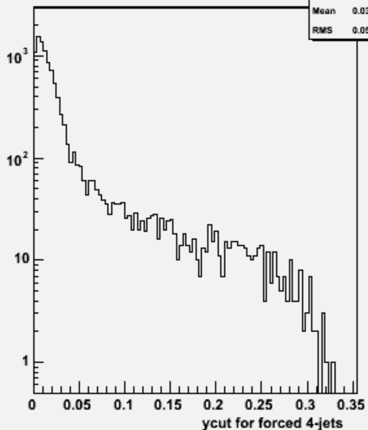
Ycut for 4-jets :w102522 e1e1ddss_o
