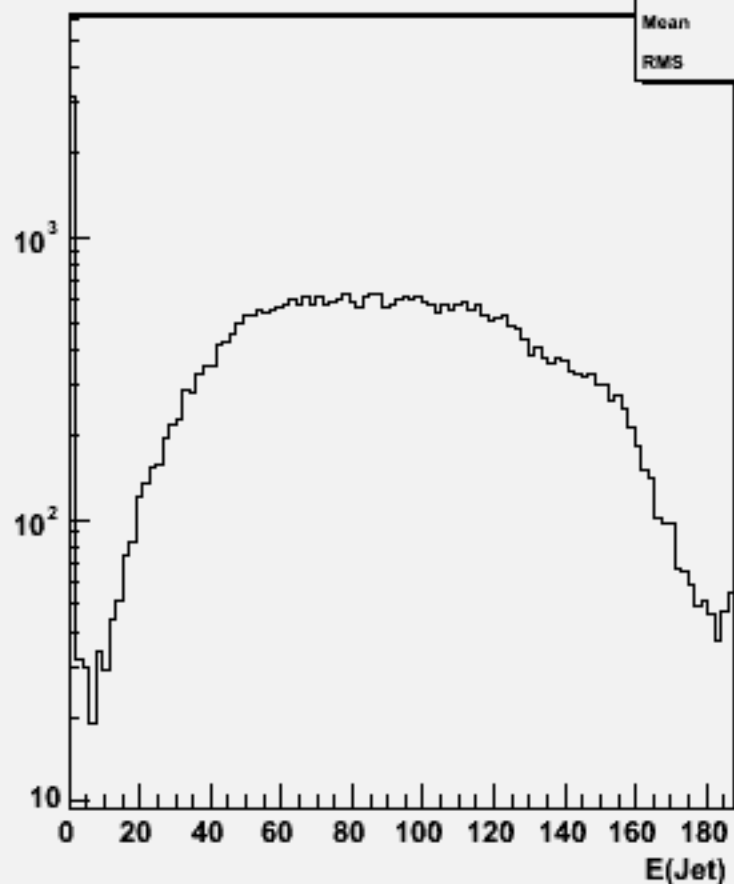
Jet energies(All jets)w102522 e1e1ddss_o
