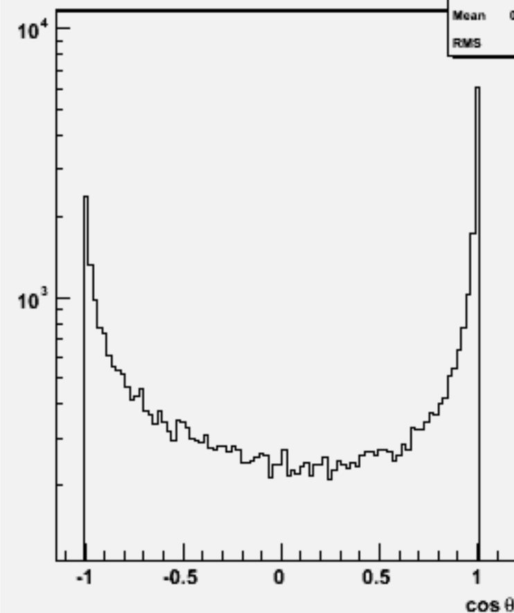
Jet cosθ (All jets)w102522 e1e1ddss_o
