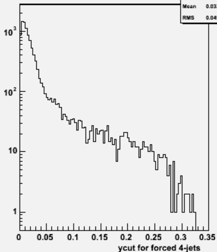
Ycut for 4-jets :w102521 e1e1ddss_o
