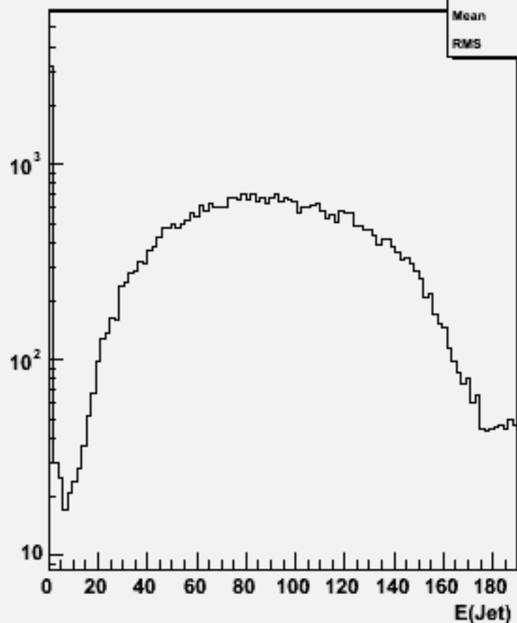
Jet energies(All jets)w102521 e1e1ddss_o
