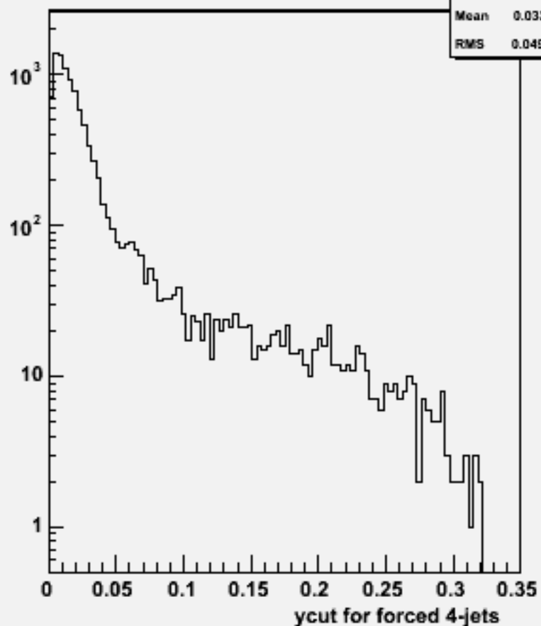
Ycut for 4-jets :w102520 e1e1ddss_o
