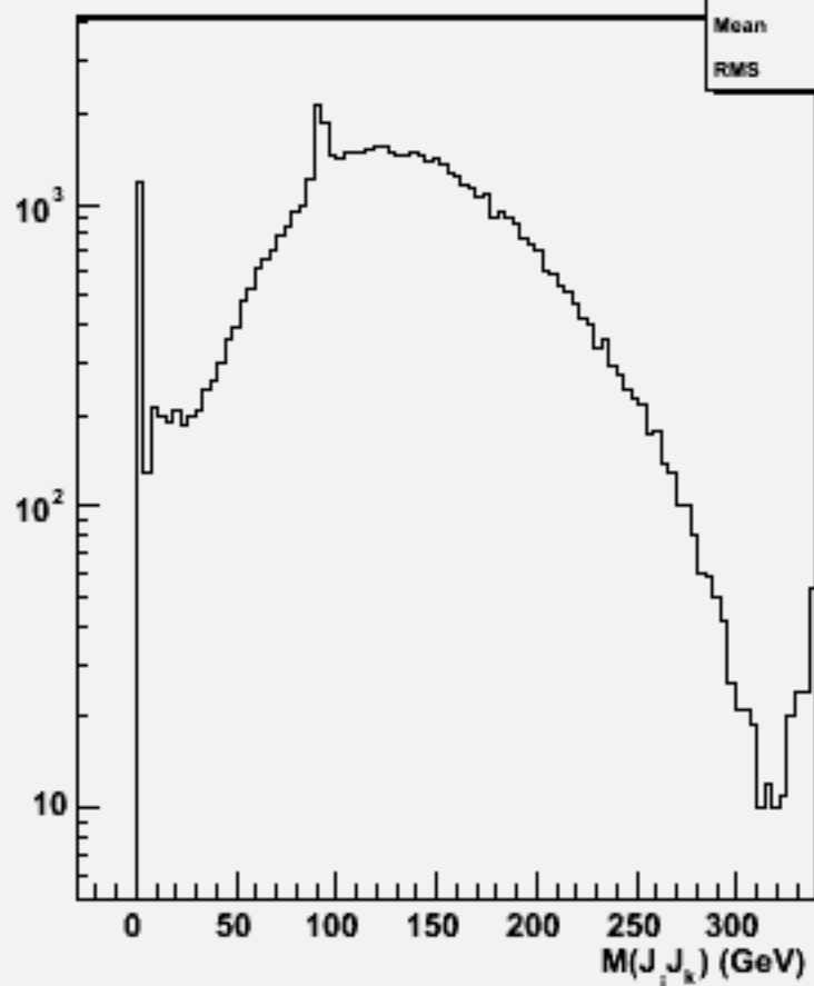
2jets mass(All comb)w102520 e1e1ddss_o
