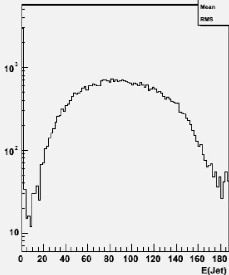
Jet energies(All jets)w102520 e1e1ddss_o
