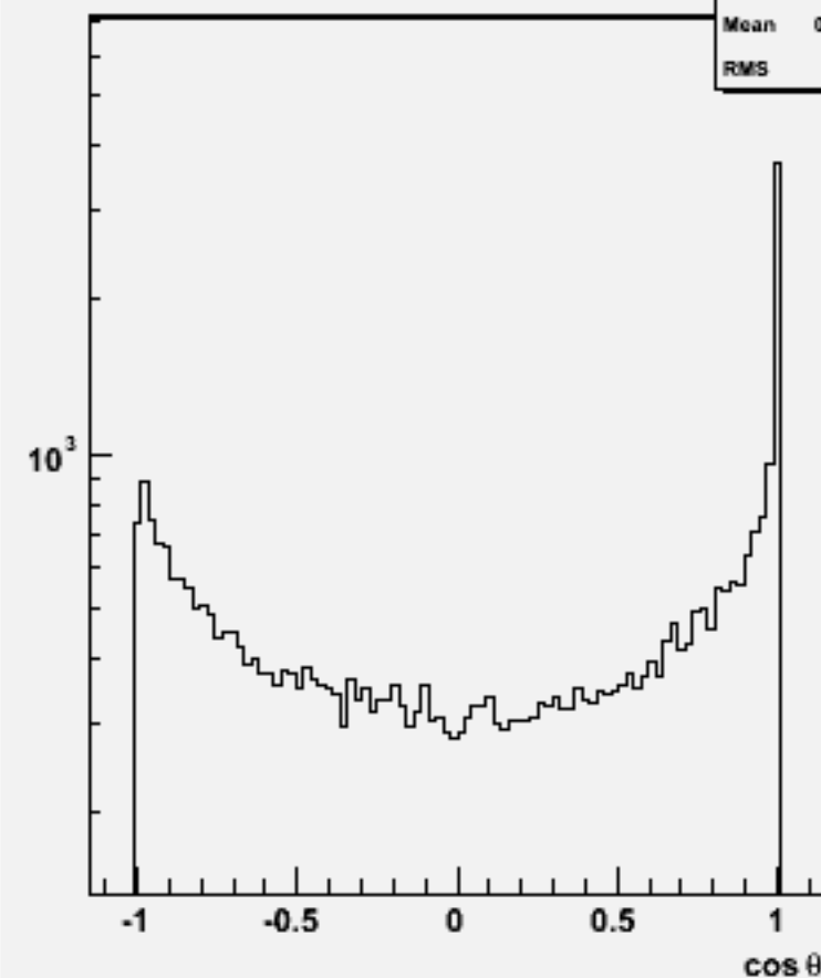
Jet cosθ (All jets)w102520 e1e1ddss_o
