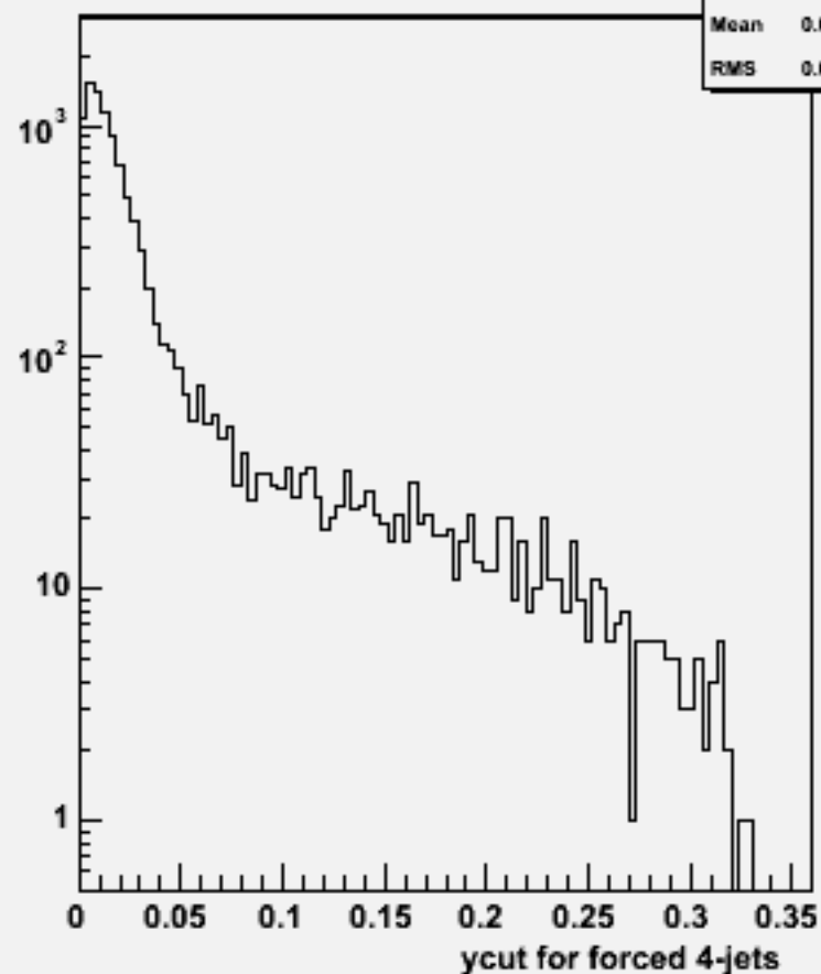
Ycut for 4-jets :w102519 e1e1ddss_o
