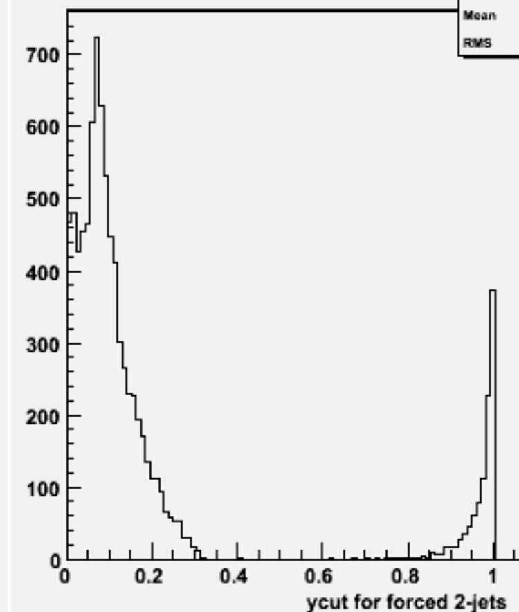
Ycut for 2-jets :w102511 e1e1e3e3bb_o
