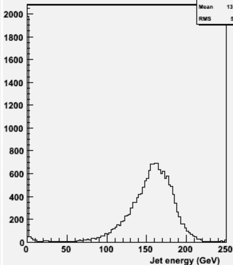
energy for 2-jets :w102511 e1e1e3e3bb_o
