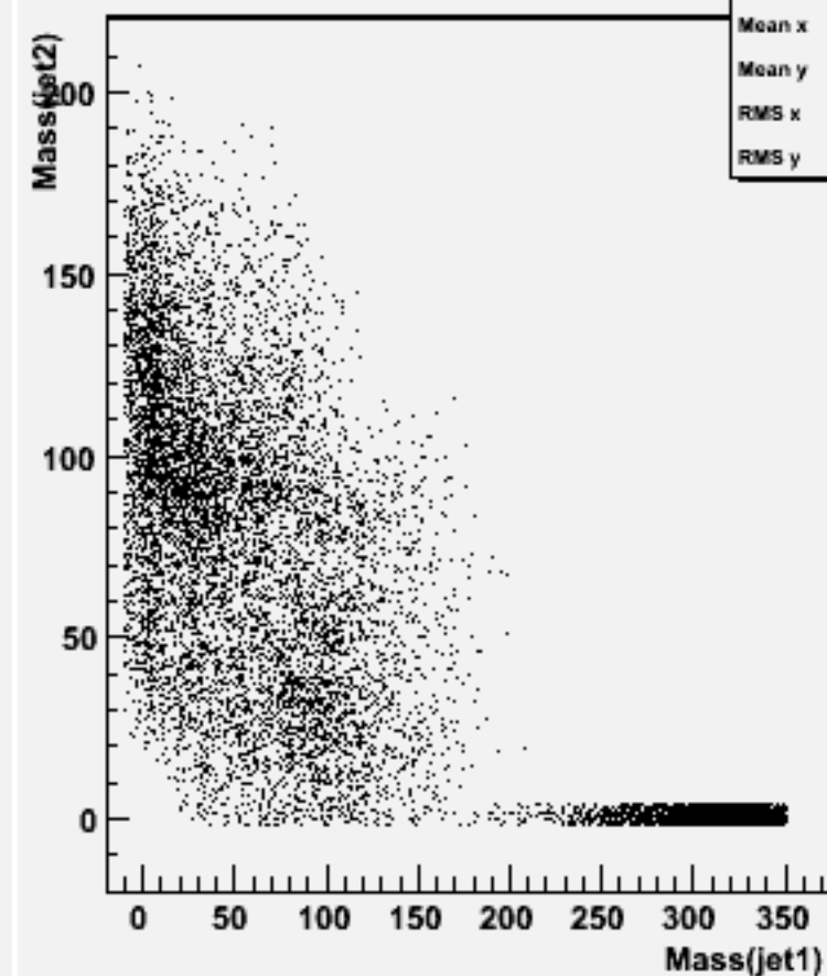
Jet mass for forced 2-jets : w102511 e1e1e3e3bb_o
