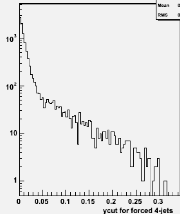
Ycut for 4-jets :w102509 e1e1e3e3ss_o
