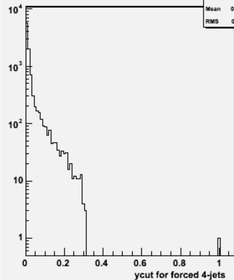
Ycut for 4-jets :w102508 e1e1e3e3ss_o
