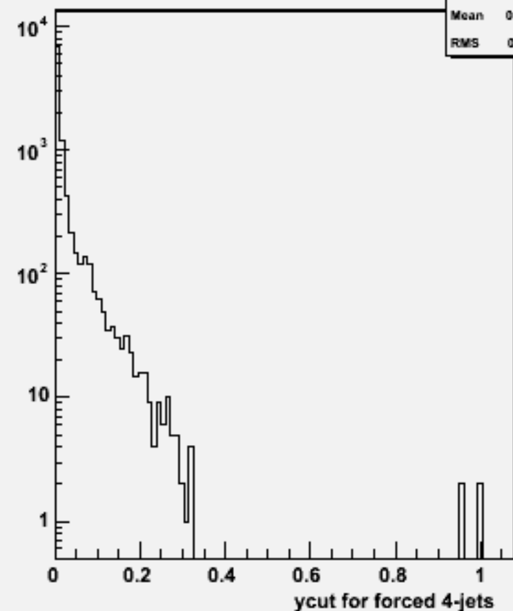
Ycut for 4-jets :w102507 e1e1e3e3ss_o
