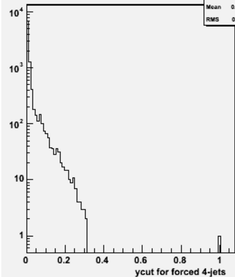
Ycut for 4-jets :w102506 e1e1e3e3dd_o
