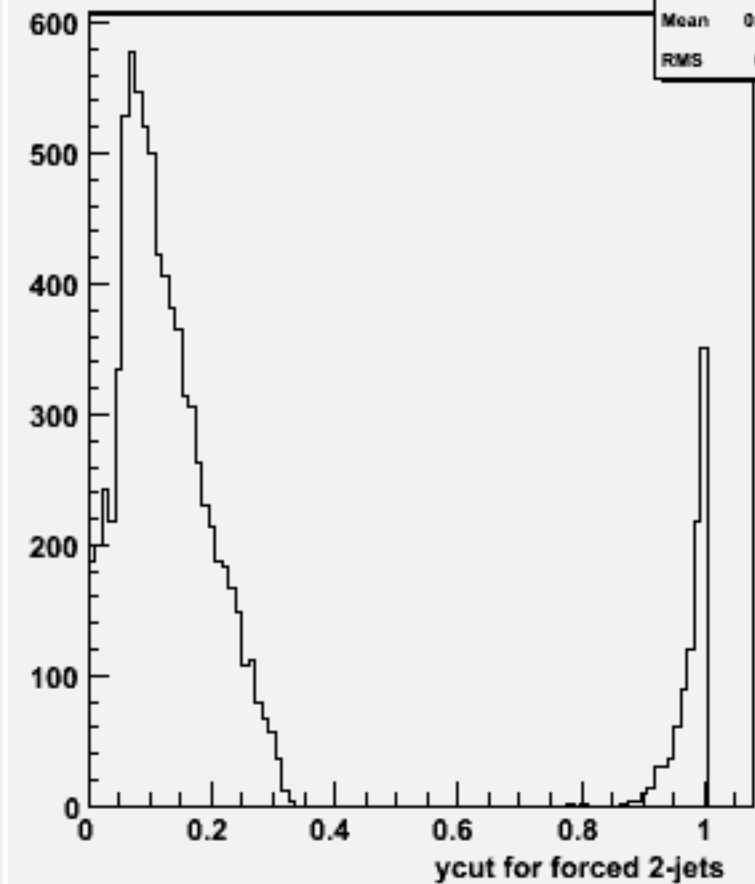
Ycut for 2-jets :w102476 e1e1e1e1bb_o
