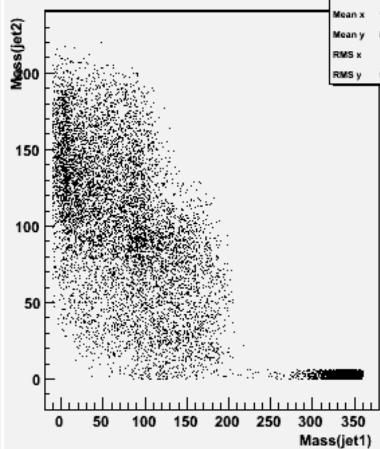
Jet mass for forced 2-jets : w102476 e1e1e1e1bb_o
