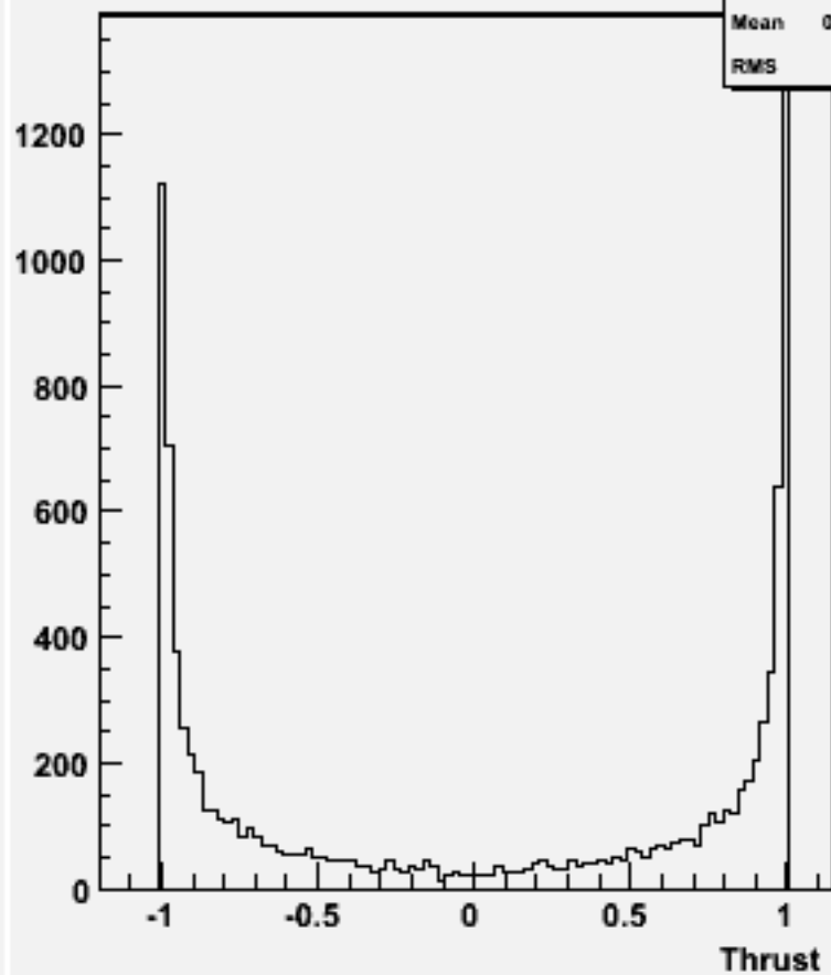
cos \Theta (thrust) w102476 e1e1e1e1bb_o
