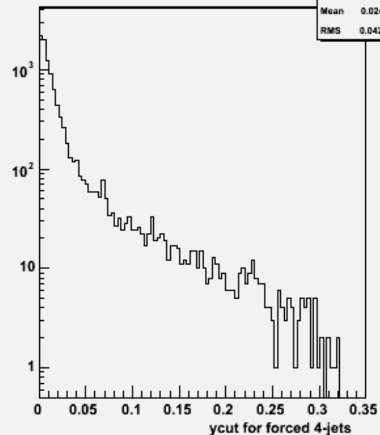
Ycut for 4-jets :w102476 e1e1e1e1bb_o
