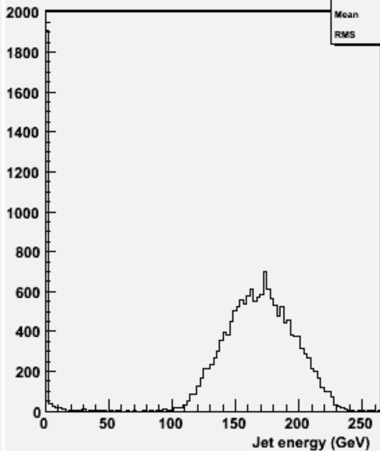
energy for 2-jets :w102476 e1e1e1e1bb_o
