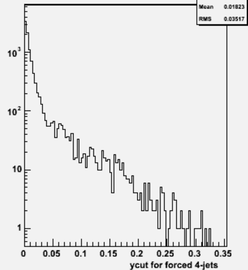
Ycut for 4-jets :w102474 e1e1e1e1ss_o
