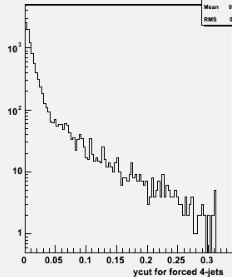
Ycut for 4-jets :w102473 e1e1e1e1ss_o
