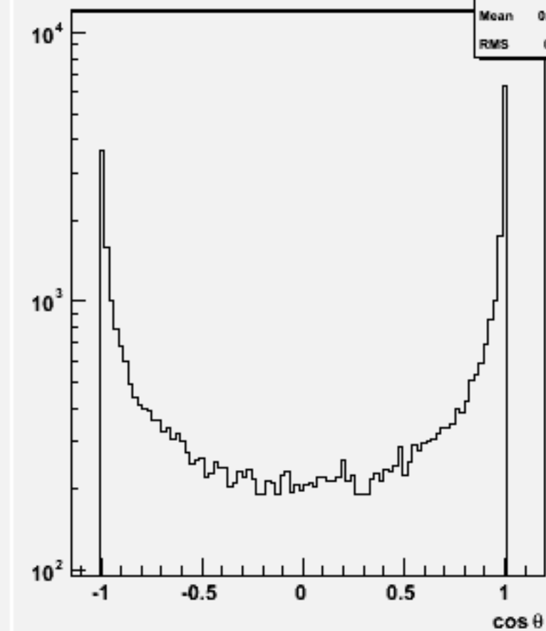
Jet cos \theta (All jets)w102473 e1e1e1e1ss_o
