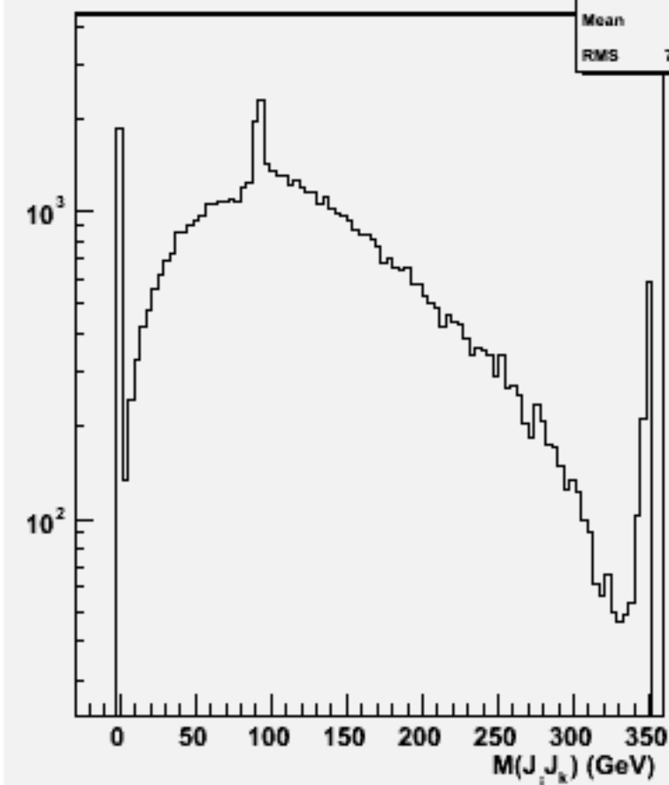
2jets mass(All comb)w102473 e1e1e1e1ss_o
