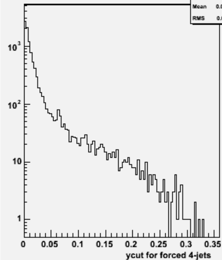
Ycut for 4-jets :w102469 e1e1e1e1dd_o
