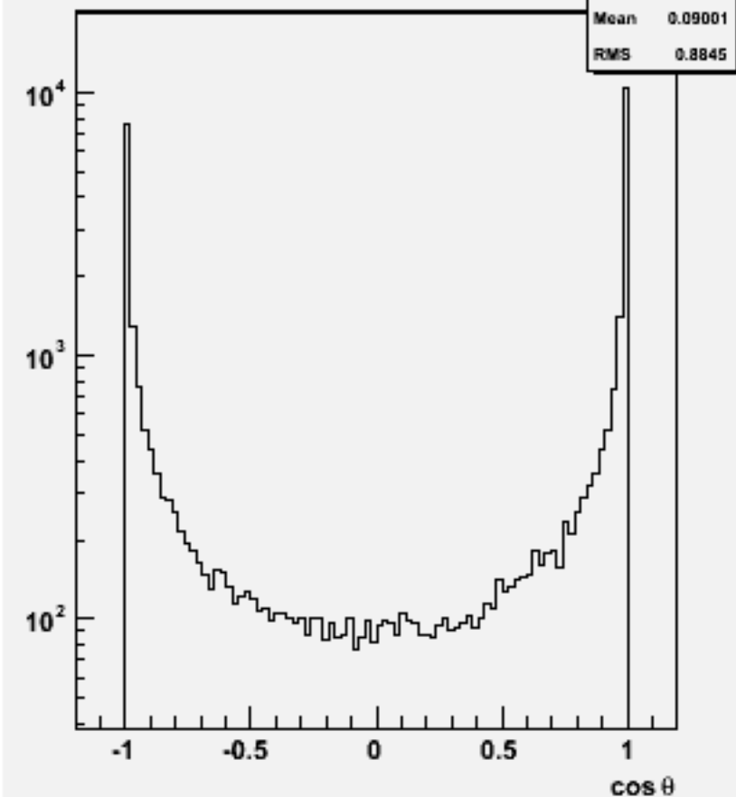
Jet cos theta (All jets)w102464 e1e1e1e1e3e3_o
