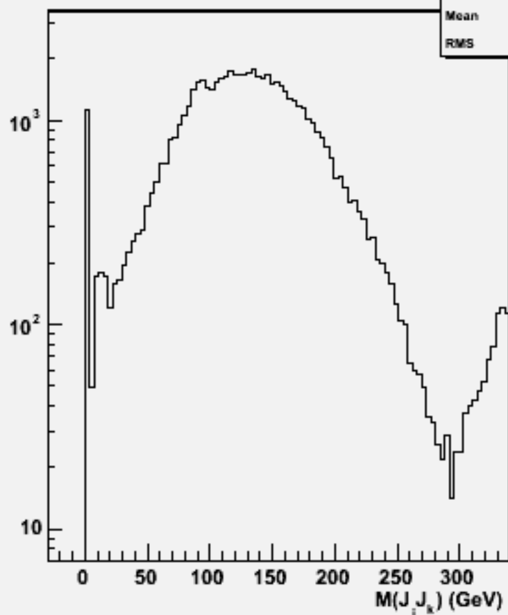
2jets mass(All comb)w102452 ccbbbb_o
