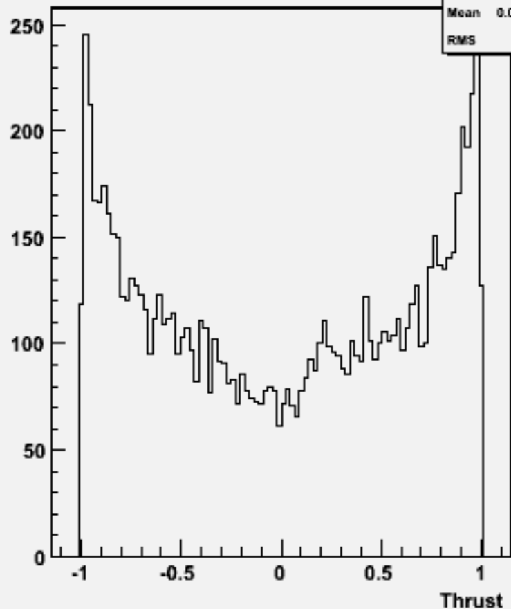
cos \Theta (thrust) w102452 ccbbbb_o
