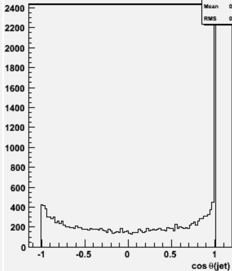
cos \theta for 2-jets :w102452 ccbbbb_o
