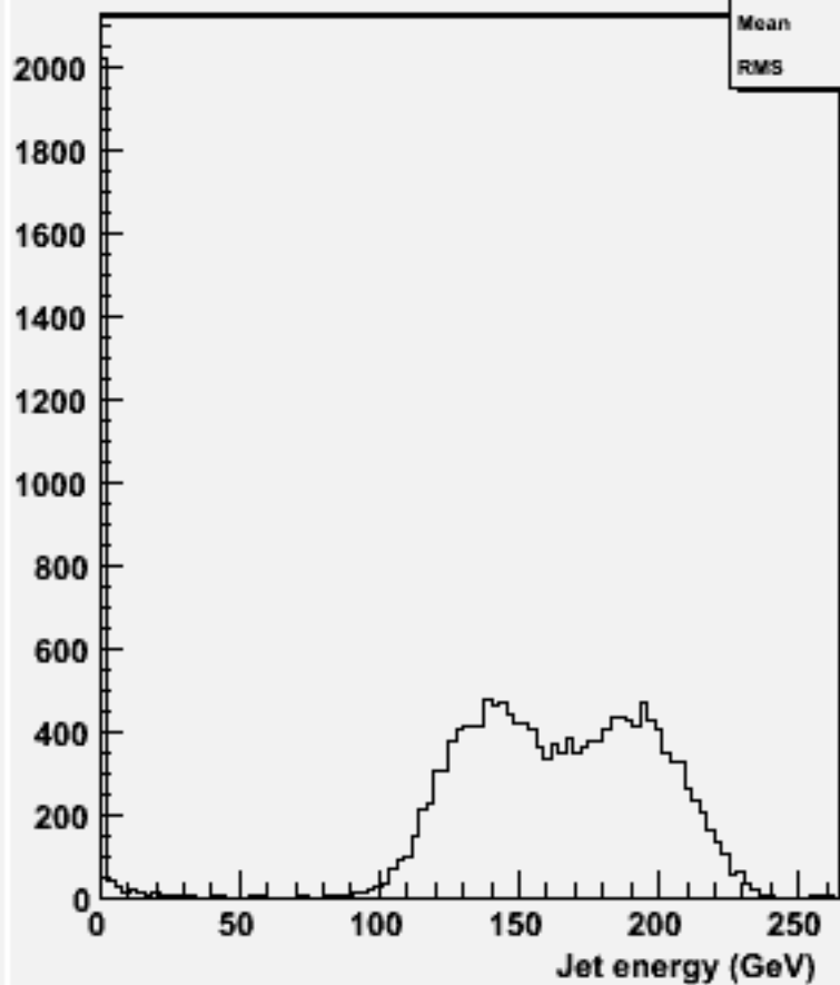
energy for 2-jets :w102452 ccbbbb_o
