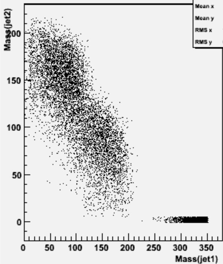
Jet mass for forced 2-jets : w102452 ccbbbb_o
