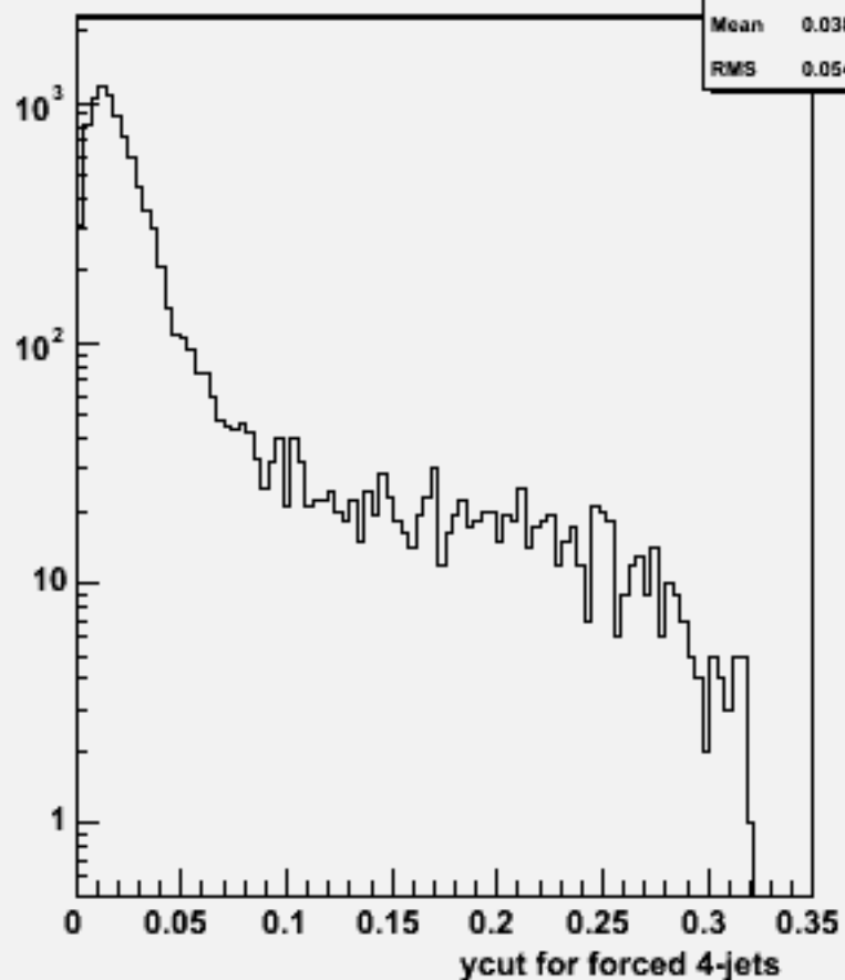
Ycut for 4-jets :w102452 ccbbbb_o
