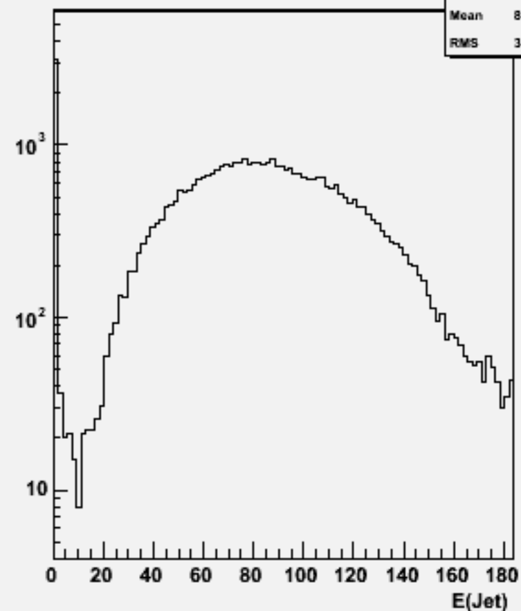
Jet energies(All jets)w102452 ccbbbb_o
