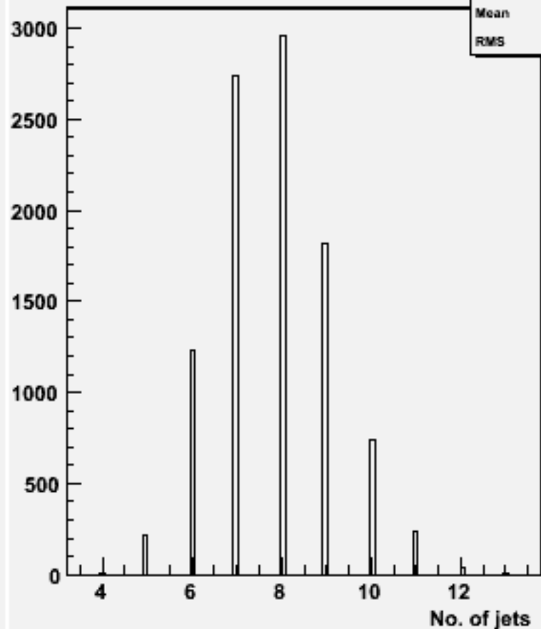
No. jets (ycut=0.001) : w102452 ccbbbb_o
