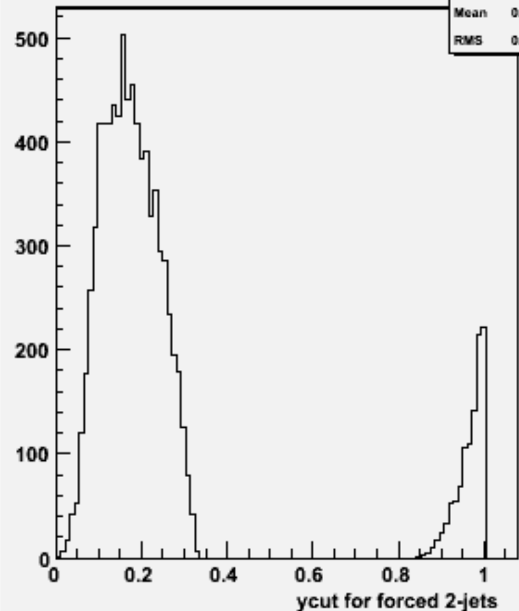
Ycut for 2-jets :w102452 ccbbbb_o
