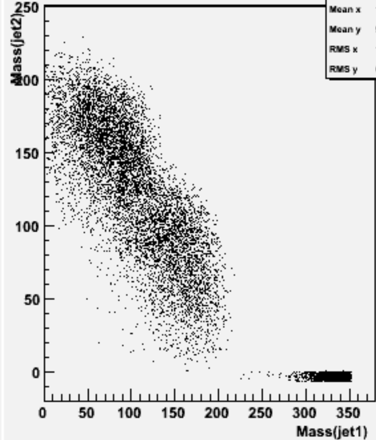
Jet mass for forced 2-jets : w102448 ccddb_o
