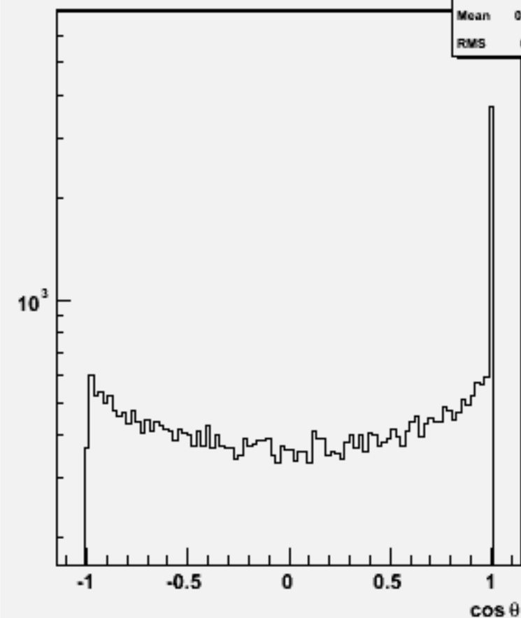
Jet cos \theta (All jets)w102448 ccddbb_o
