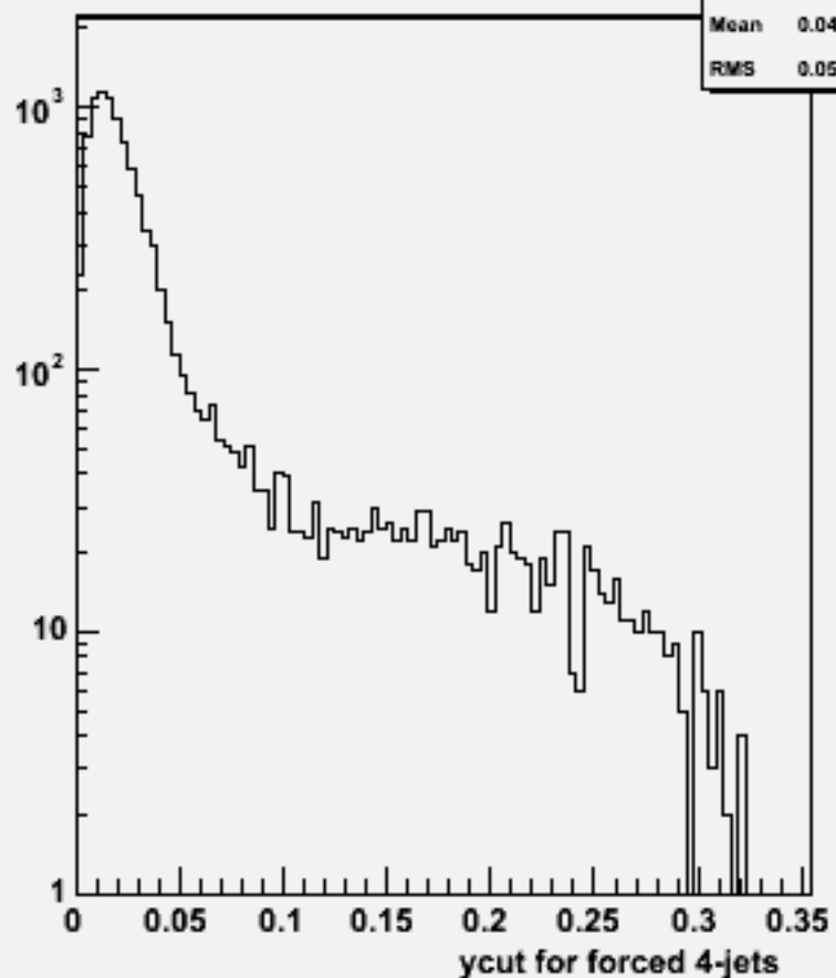
Ycut for 4-jets :w102448 ccddbb_o
