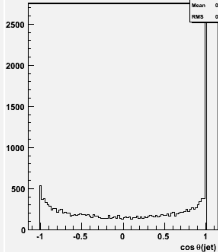
cos \Theta for 2-jets :w102448 ccddb_o
