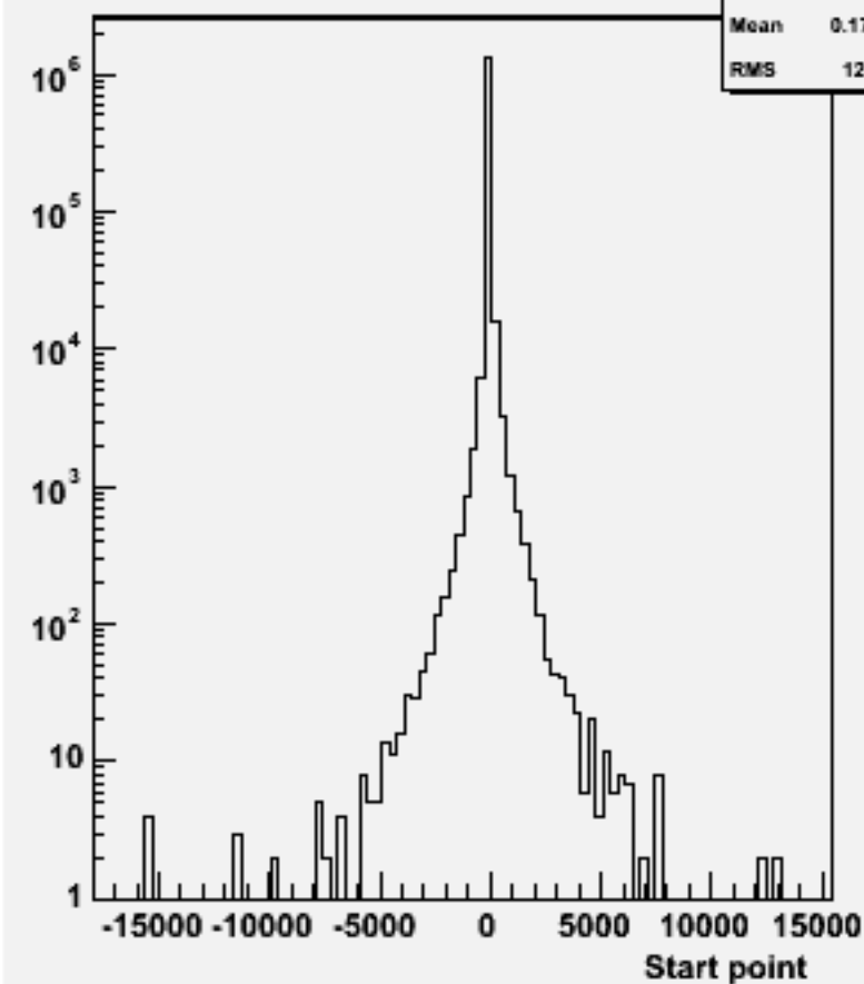
Start point Z : w102448 ccddbb_o
