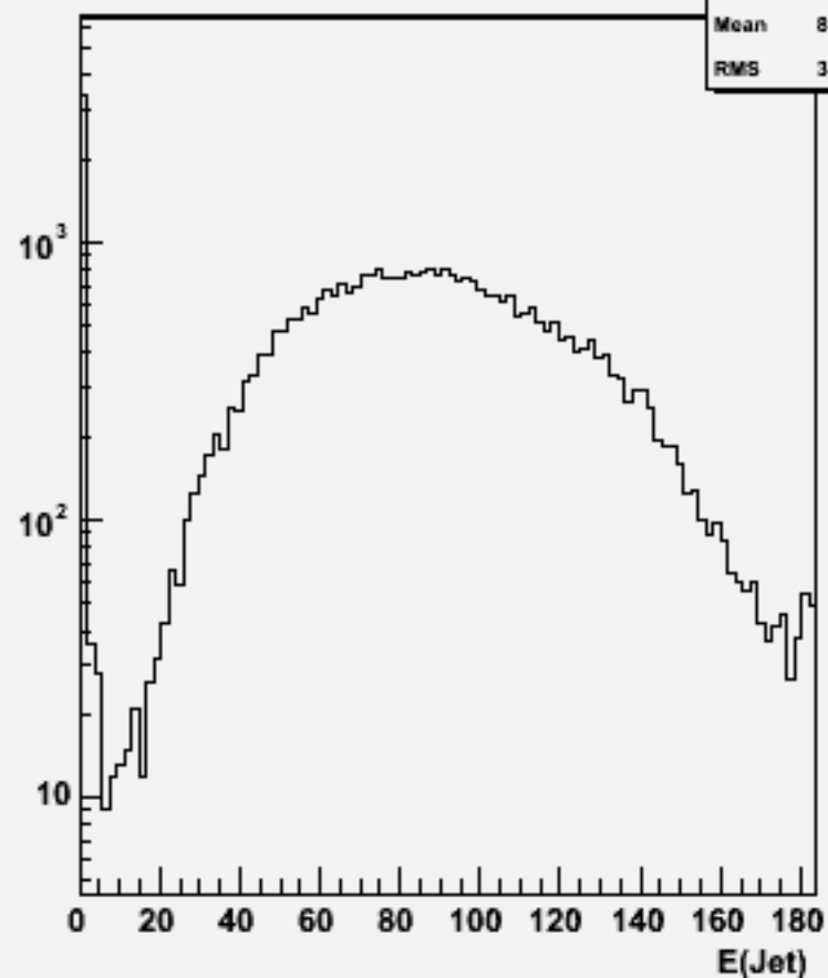
Jet energies(All jets)w102448 ccddbb_o
