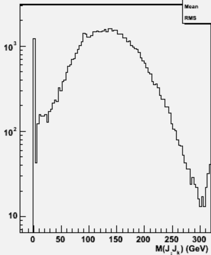
2jets mass(All comb)w102448 ccddbb_o
