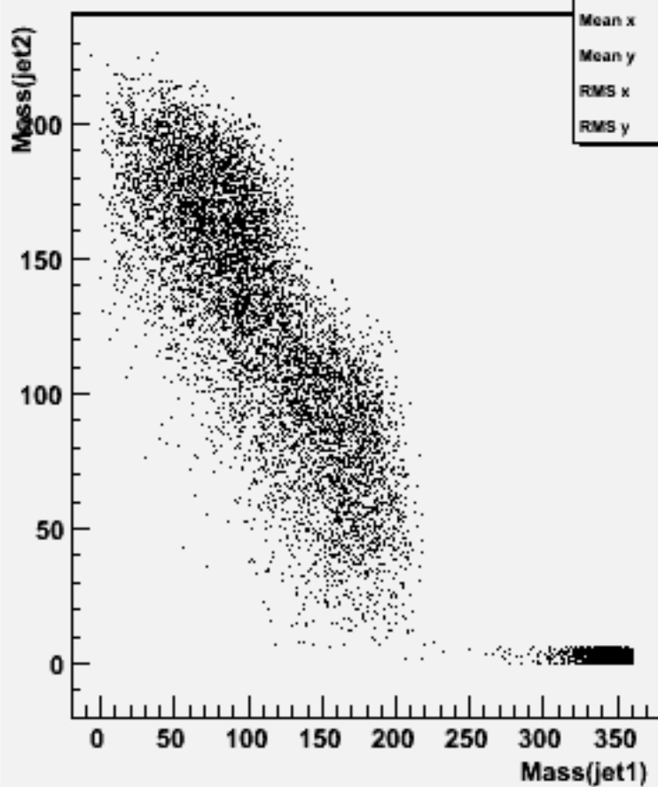
Jet mass for forced 2-jets : w102444 ccdddd_o
