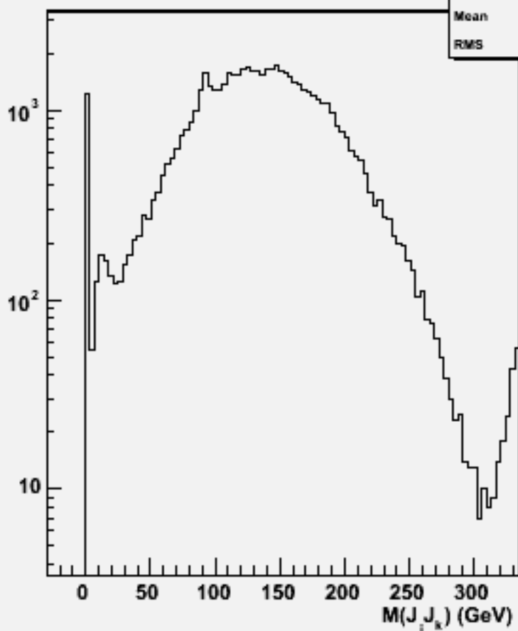
2jets mass(All comb)w102444 ccdddd_o
