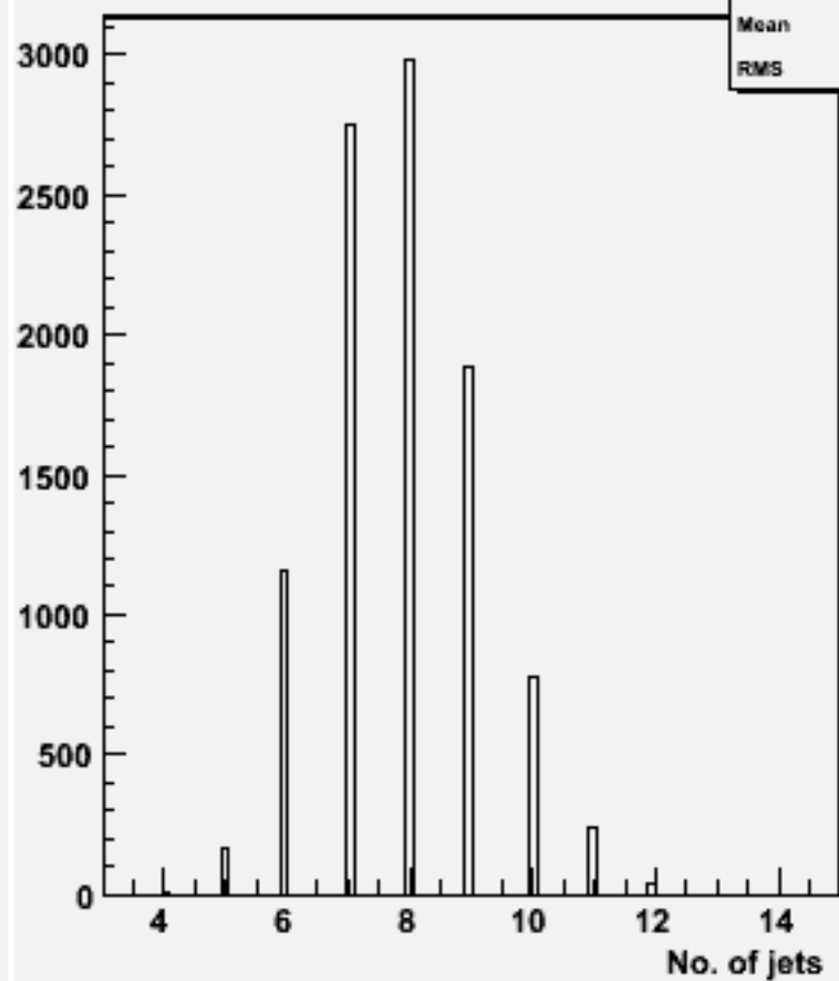
No. jets (ycut=0.001) : w102444 ccdddd_o
