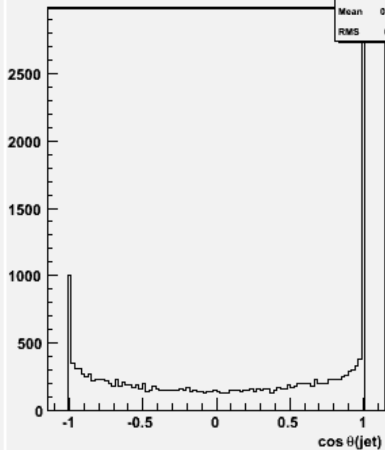
cos \Theta for 2-jets :w102444 ccdddd_o
