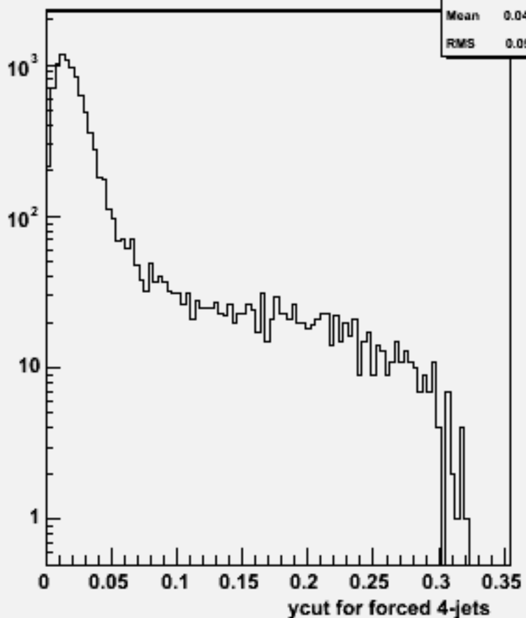
Ycut for 4-jets :w102444 ccdddd_o
