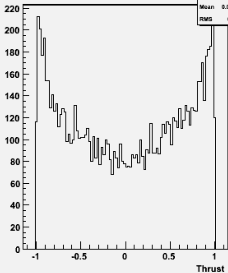
cos \Theta (thrust) w102444 ccdddd_o
