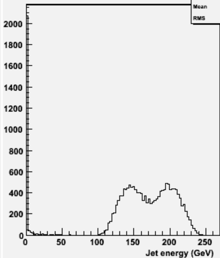
energy for 2-jets :w102444 ccdddd_o
