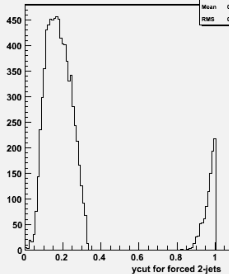
Ycut for 2-jets :w102444 ccdddd_o
