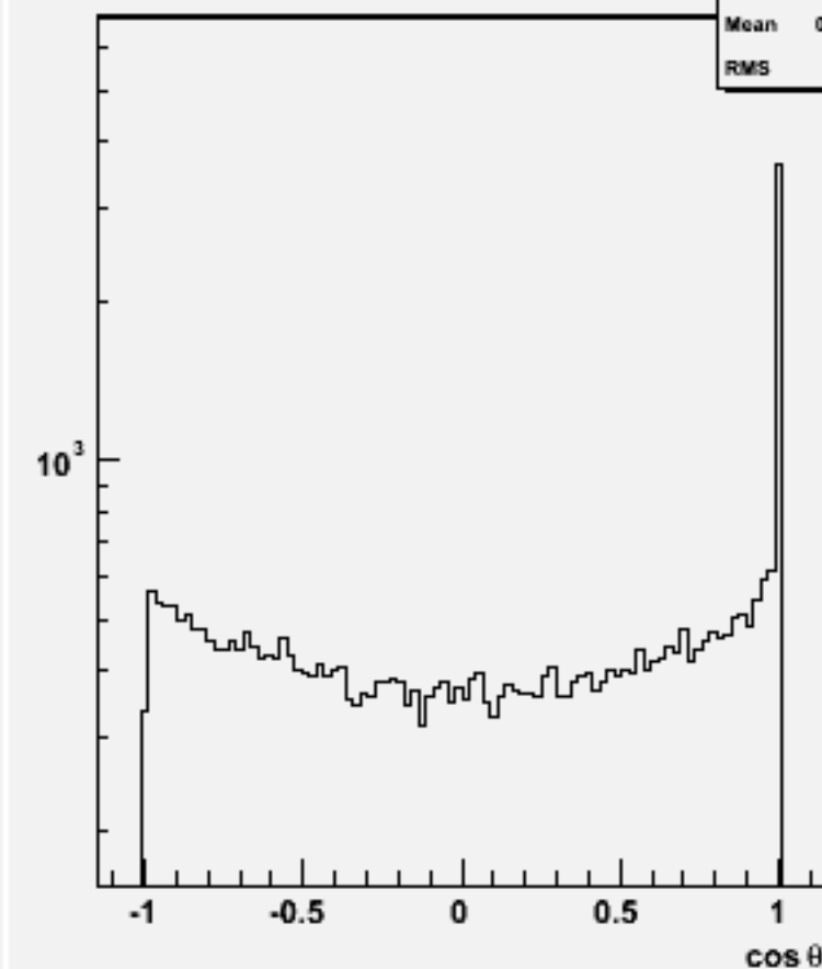
Jet cos \theta (All jets)w102444 ccdddd_o
