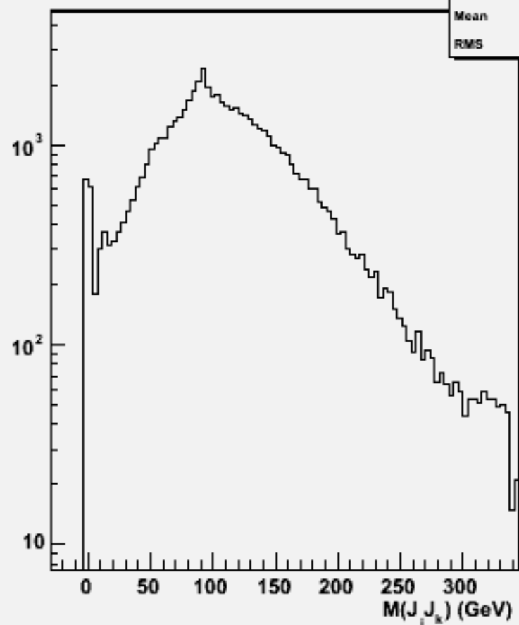
2jets mass(All comb)w102441 cce3e3bb_o
