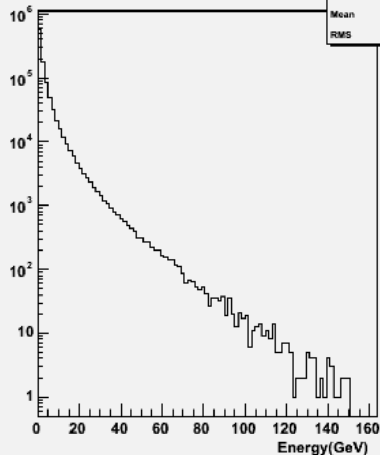
Particle Energy : w102441 cce3e3bb_o
