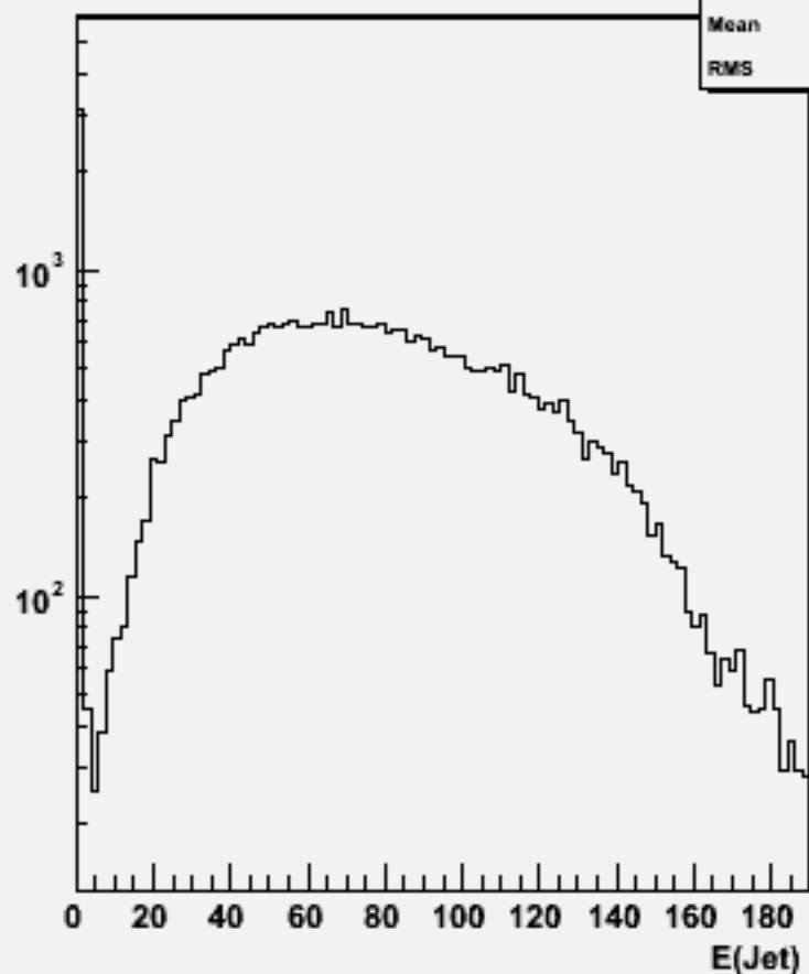
Jet energies(All jets)w102441 cce3e3bb_o
