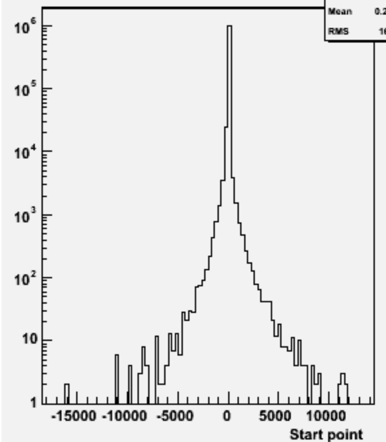
Start point Z : w102441 cce3e3bb_o
