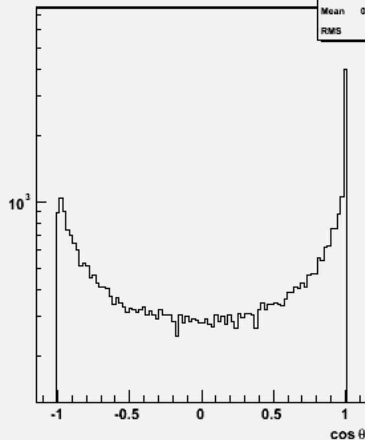
Jet cosθ (All jets)w102441 cce3e3bb_o
