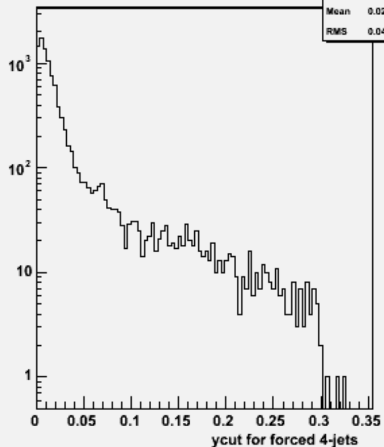
Ycut for 4-jets :w102441 cce3e3bb_o
