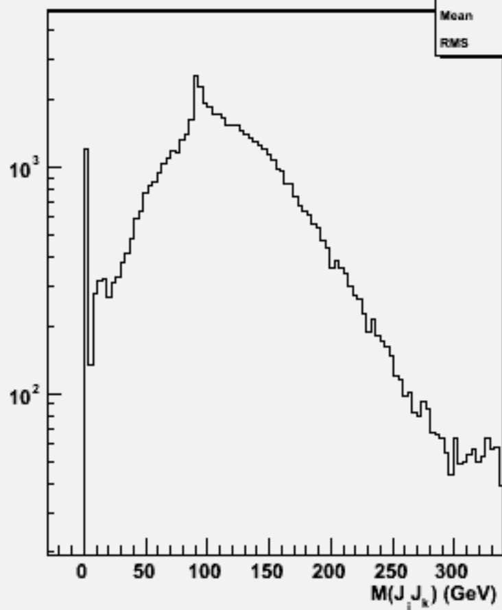
2jets mass(All comb)w102436 cce3e3dd_o
