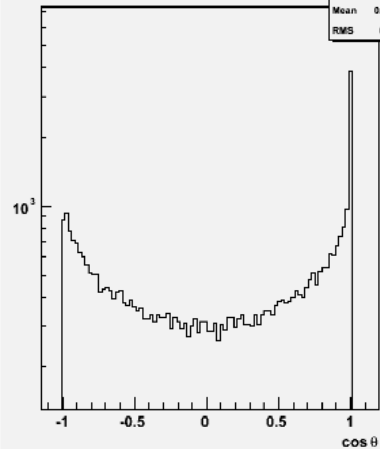
Jet cosθ (All jets)w102436 cce3e3dd_o
