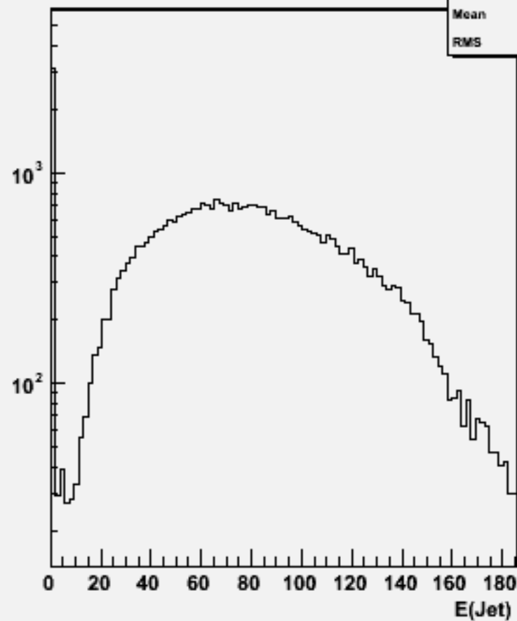
Jet energies(All jets)w102436 cce3e3dd_o
