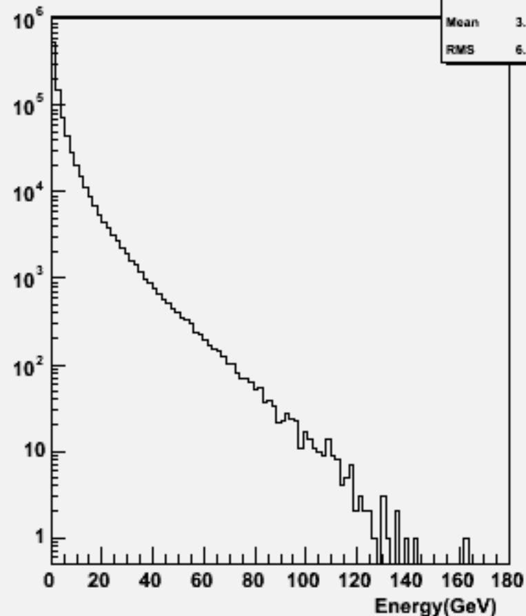
Particle Energy : w102436 cce3e3dd_o
