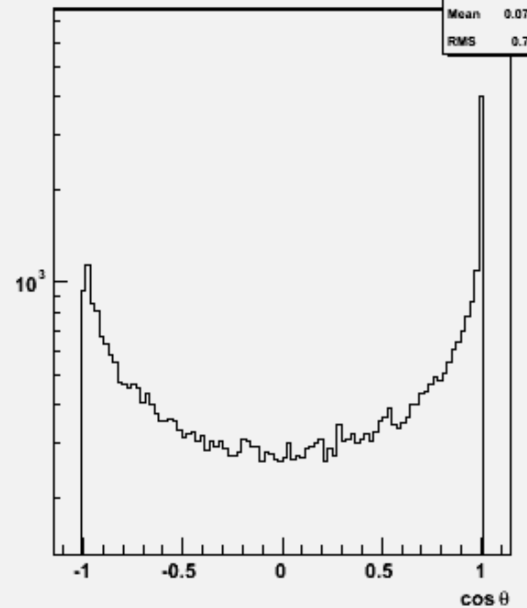
Jet cosθ (All jets)w102429 cce2e2bb_o
