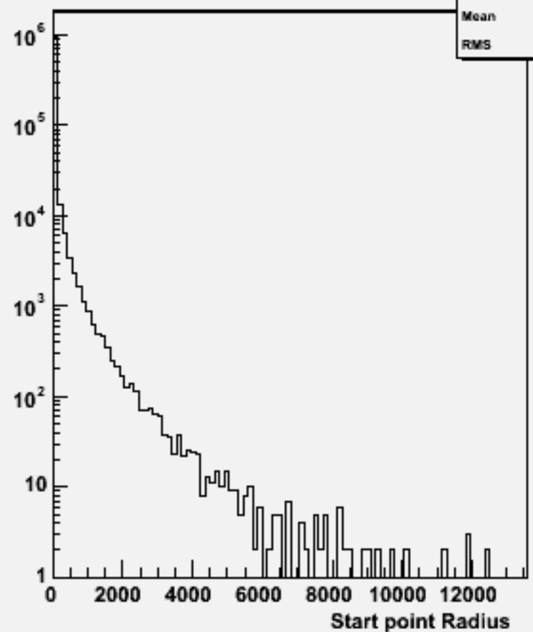
Start point R : w102429 cce2e2bb_o
