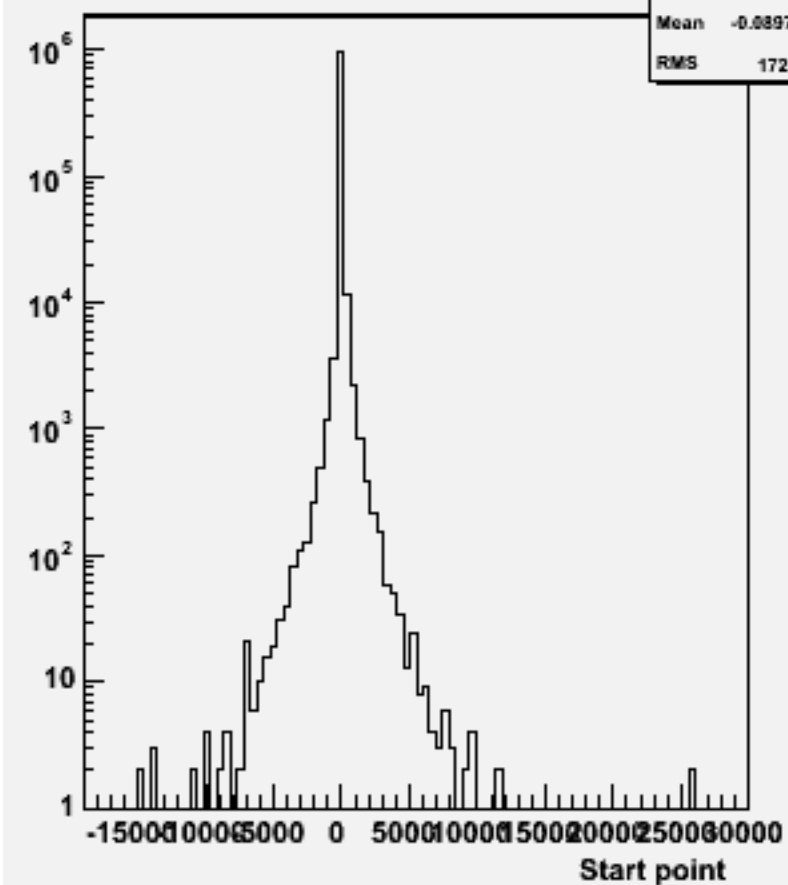
Start point Z : w102429 cce2e2bb_o
