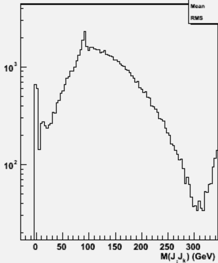
2jets mass(All comb)w102429 cce2e2bb_o
