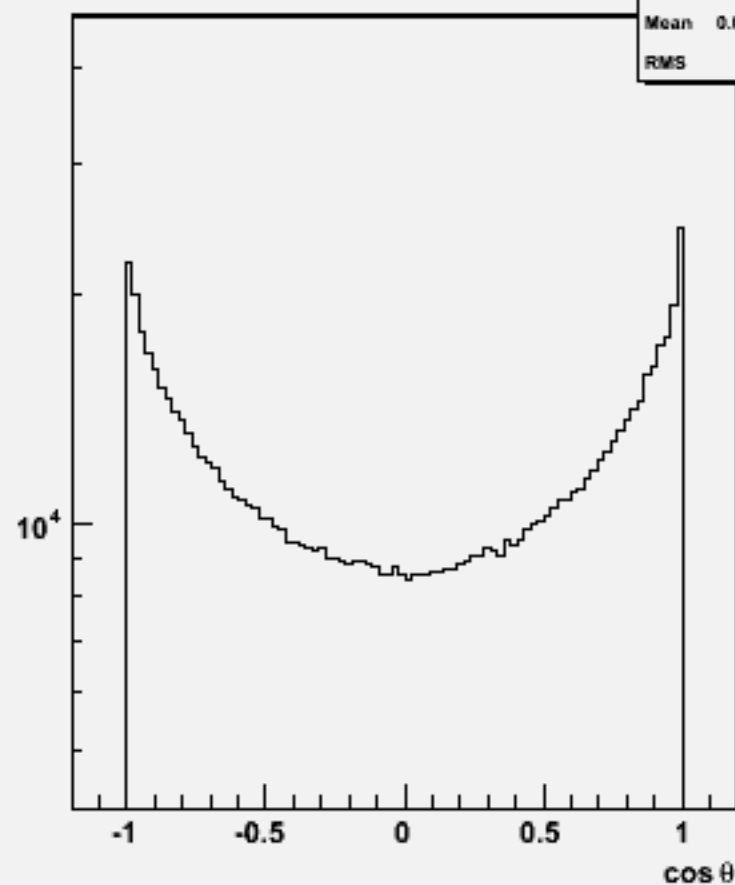
Particle cos \theta : w102429 cce2e2bb_o
