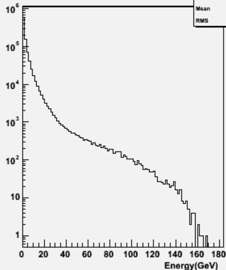
Particle Energy : w102429 cce2e2bb_o
