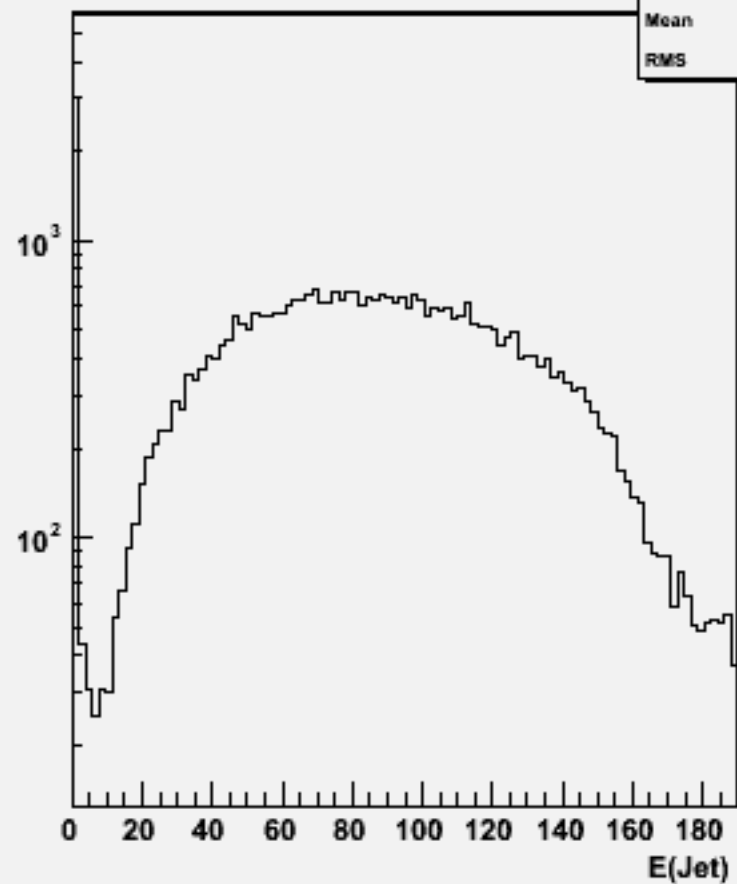
Jet energies(All jets)w102429 cce2e2bb_o
