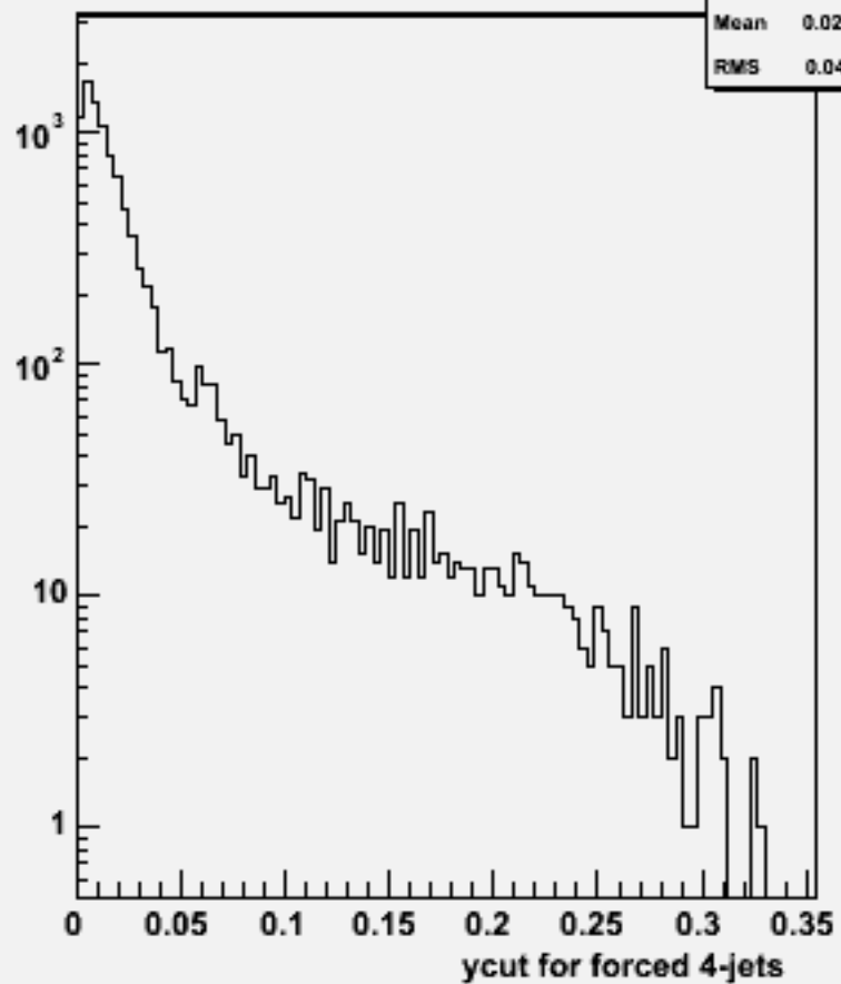
Ycut for 4-jets :w102429 cce2e2bb_o
