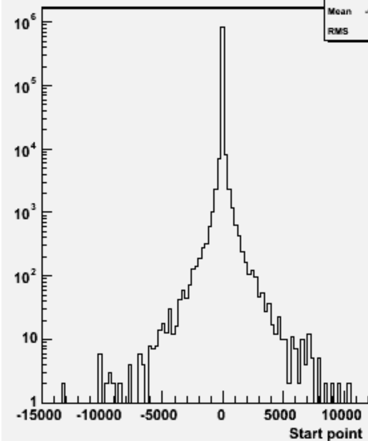
Start point Z : w102424 cce2e2dd_o
