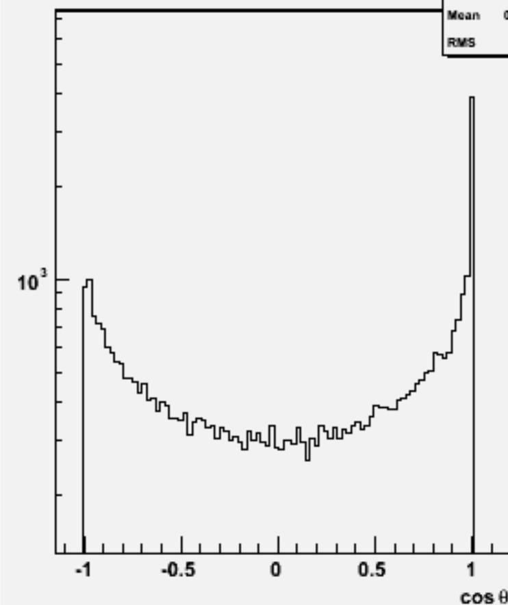
Jet cosθ (All jets)w102424 cce2e2dd_o
