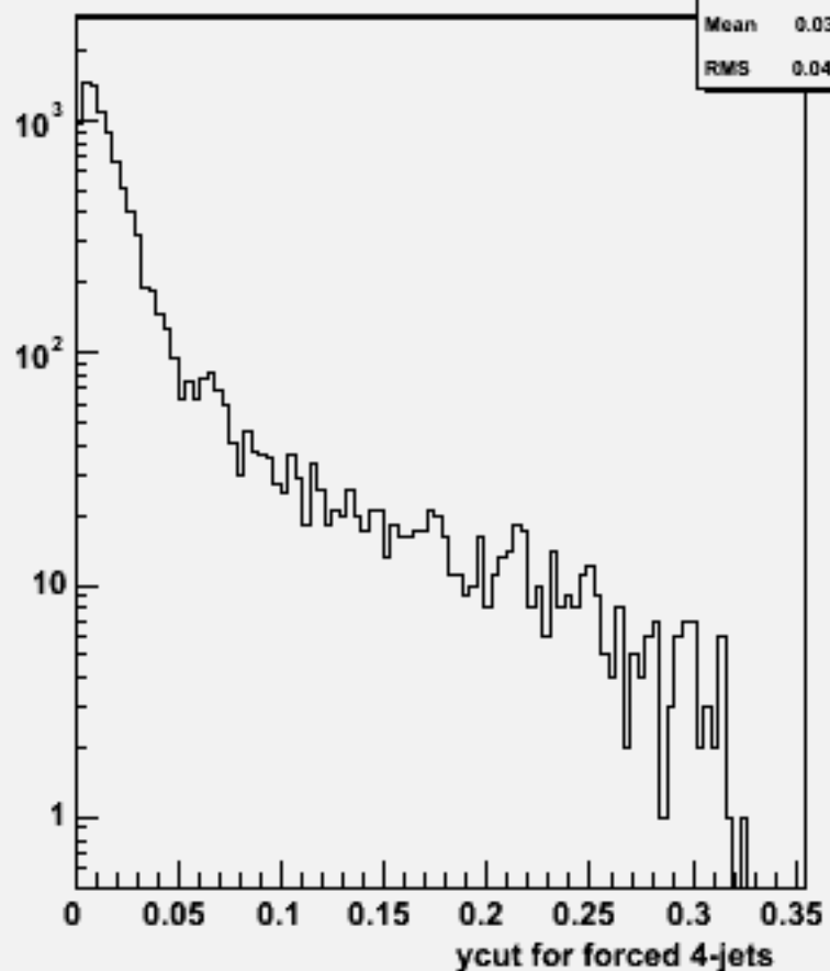
Ycut for 4-jets :w102424 cce2e2dd_o
