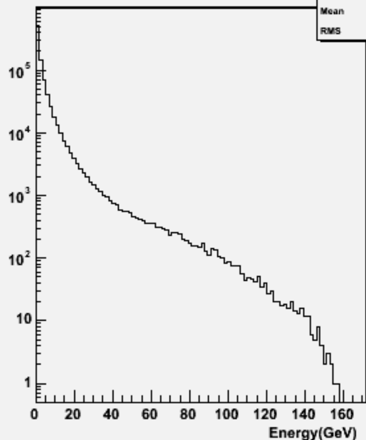
Particle Energy : w102424 cce2e2dd_o
