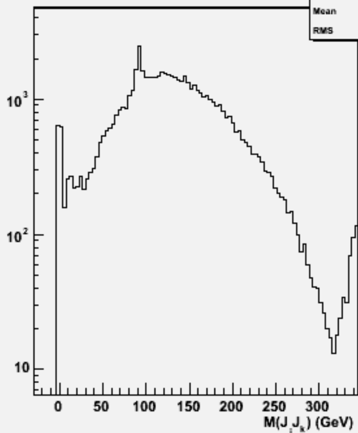
2jets mass(All comb)w102424 cce2e2dd_o
