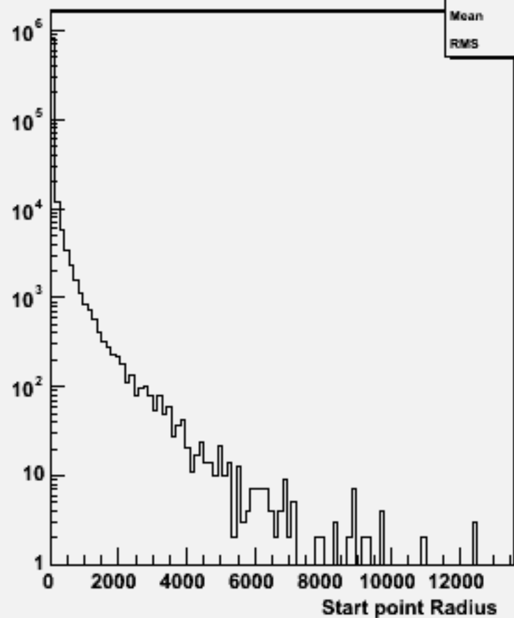
Start point R : w102424 cce2e2dd_o
