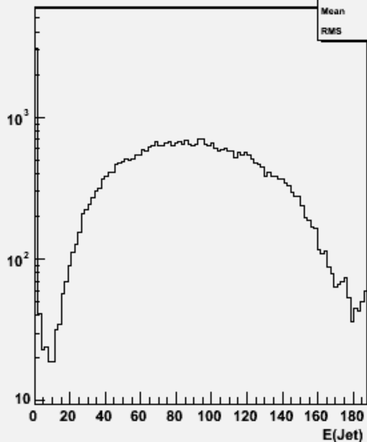
Jet energies(All jets)w102424 cce2e2dd_o
