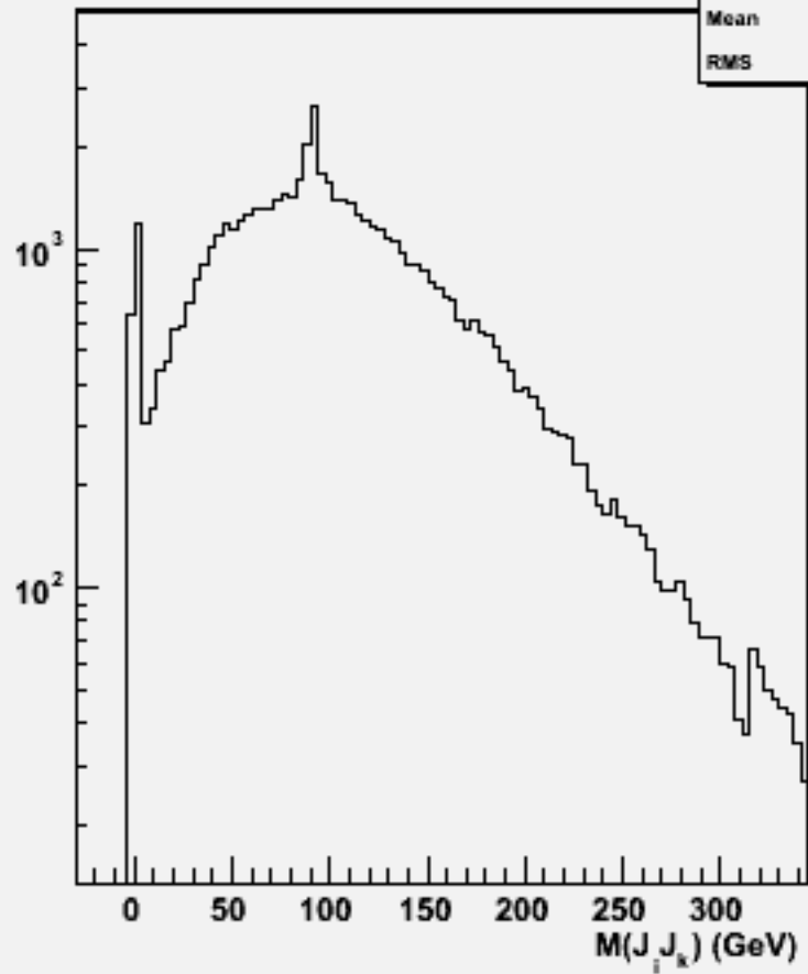
2jets mass(All comb)w102421 cce2e2e3e3_o
