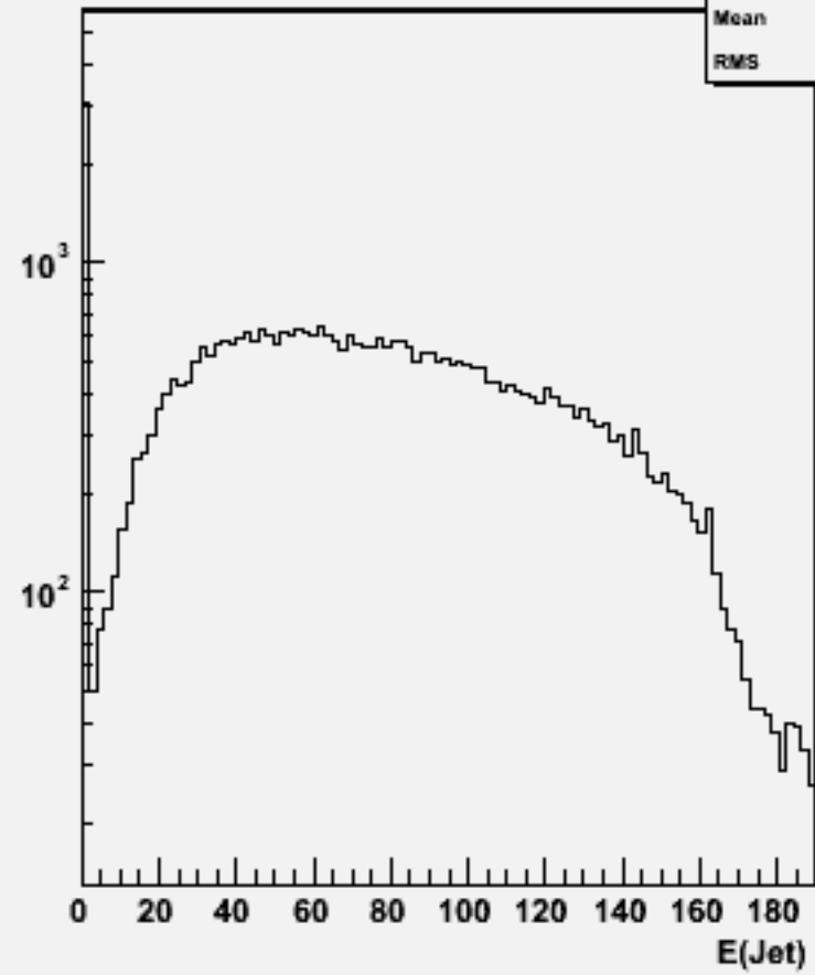
Jet energies(All jets)w102421 cce2e2e3e3_o
