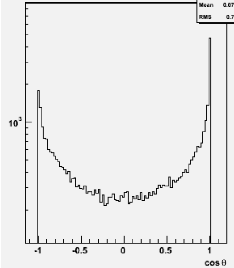
Jet cos \theta (All jets)w102421 cce2e2e3e3_o
