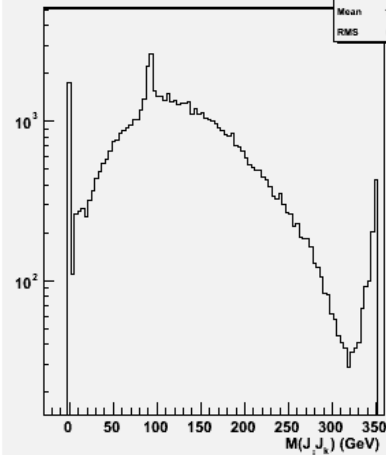
2jets mass(All comb)w102416 cce2e2e2e2_o
