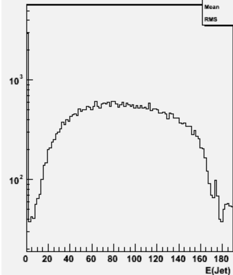
Jet energies(All jets)w102416 cce2e2e2e2_o
