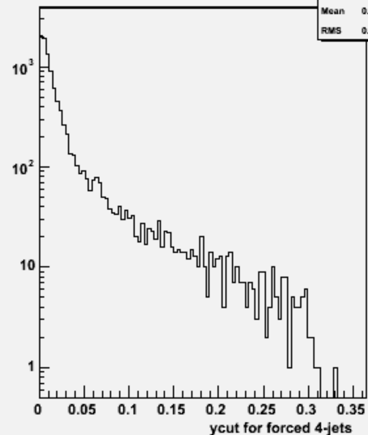
Ycut for 4-jets :w102416 cce2e2e2e2_o
