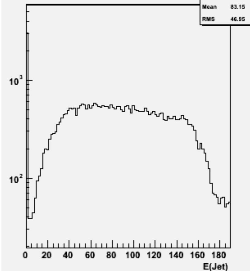
Jet energies(All jets)w102414 cce1e1bb_o
