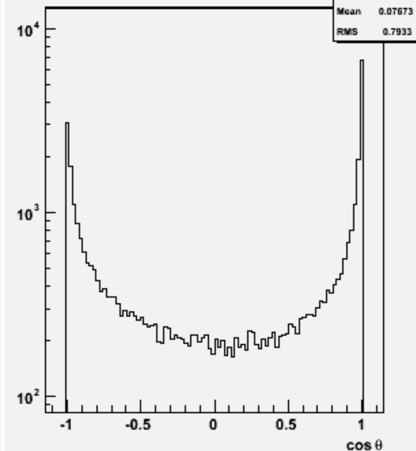
Jet cosθ (All jets)w102414 cce1e1bb_o
