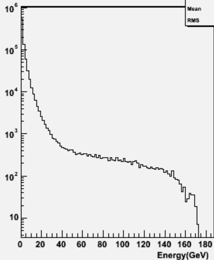
Particle Energy : w102414 cce1e1bb_o
