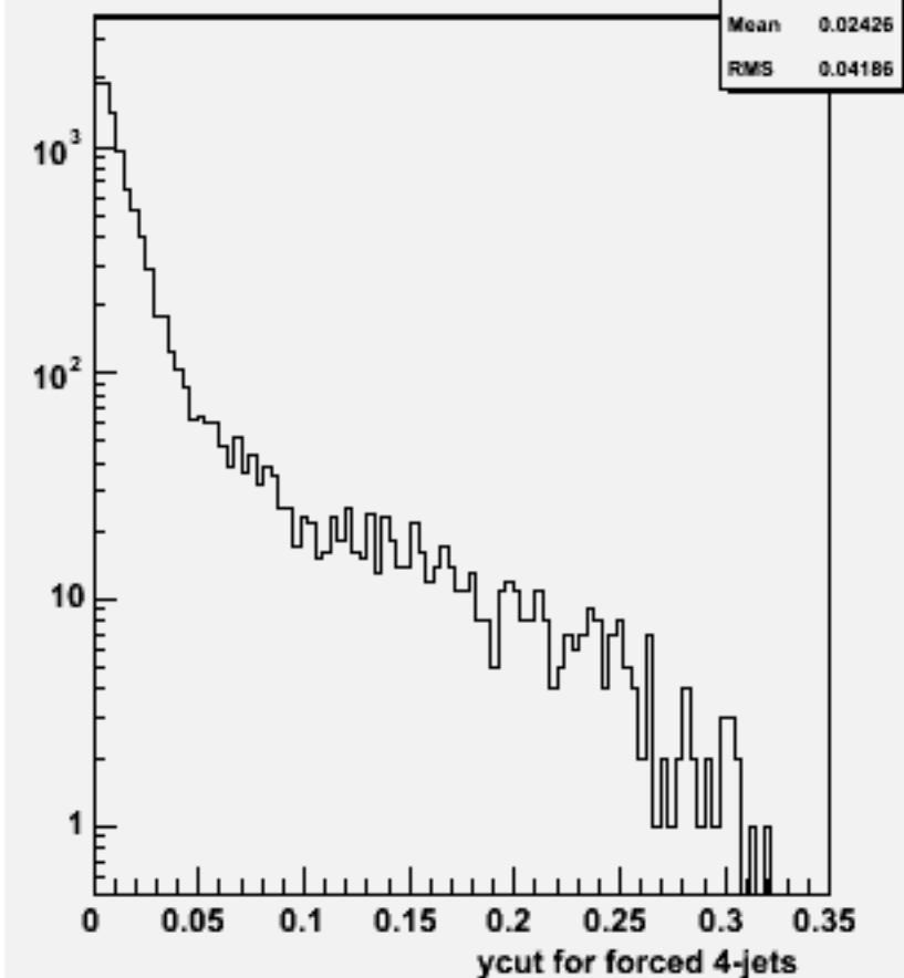
Ycut for 4-jets :w102414 cce1e1bb_o
