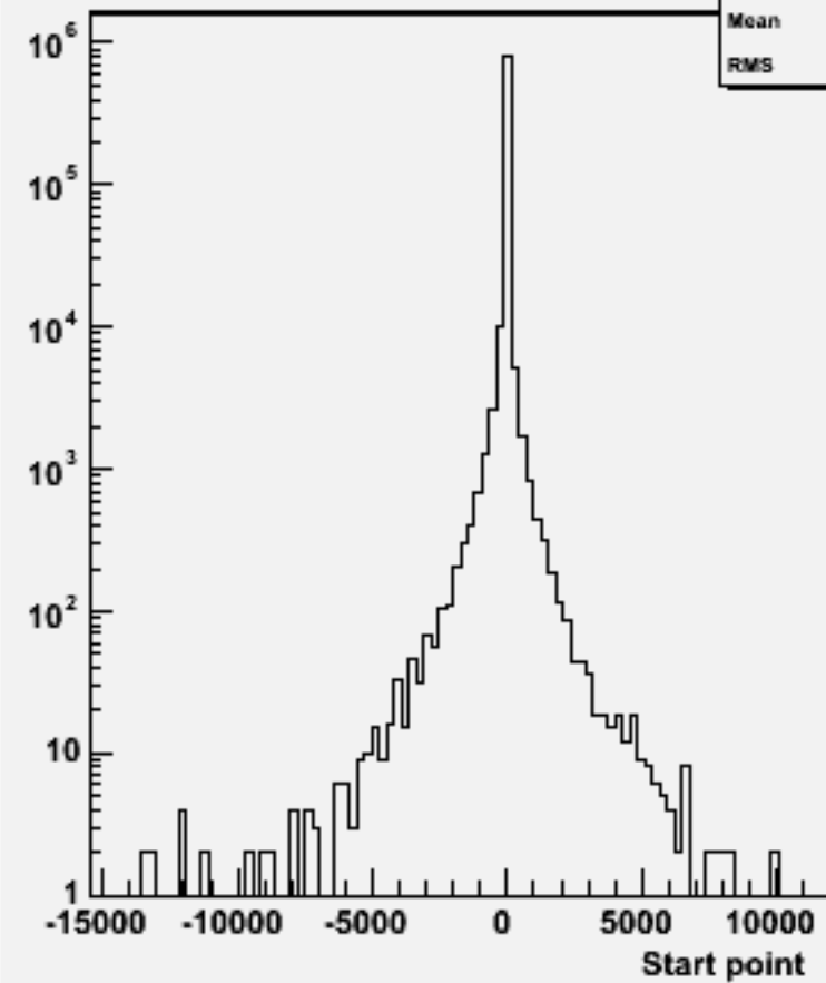
Start point Z : w102414 cce1e1bb_o
