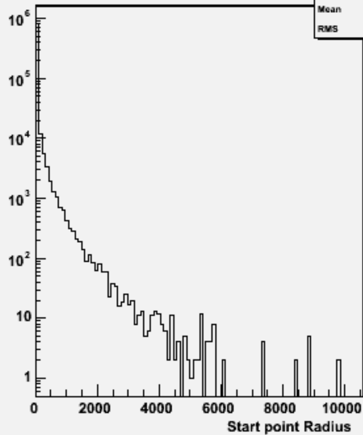
Start point R : w102414 cce1e1bb_o
