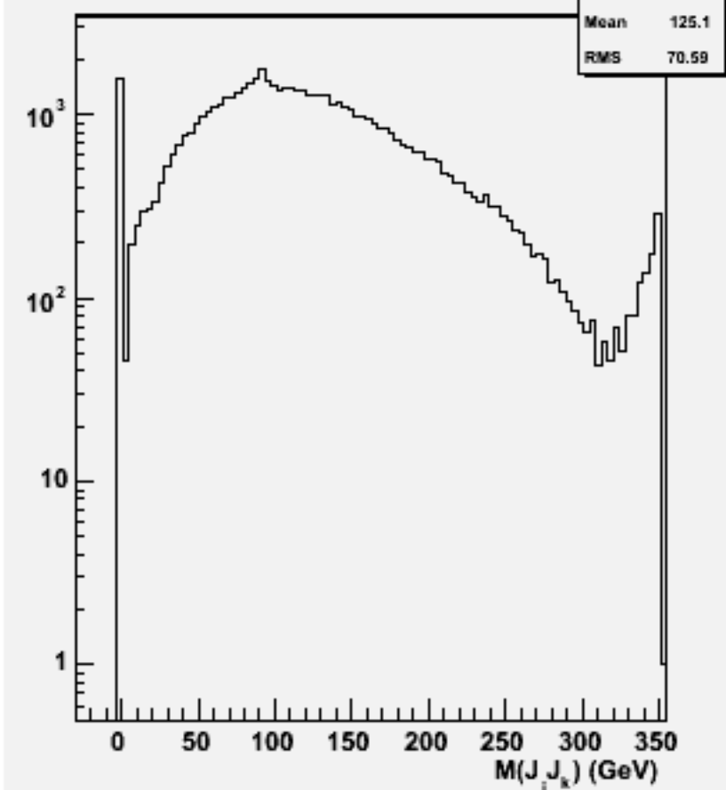
2jets mass(All comb)w102414 cce1e1bb_o
