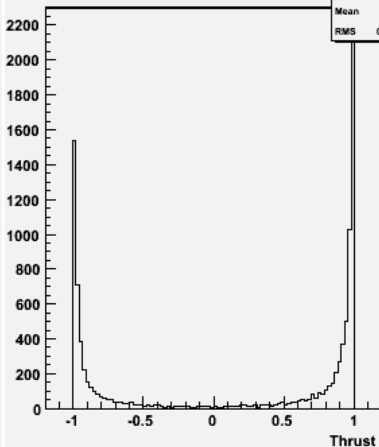
cos \Theta (thrust) w102411 cce1e1bb_o
