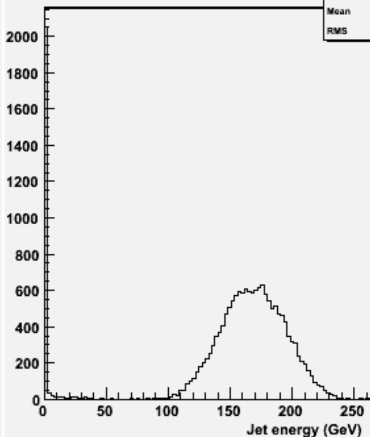
energy for 2-jets :w102411 cce1e1bb_o
