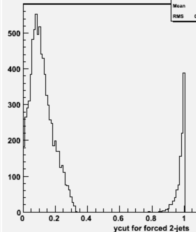
Ycut for 2-jets :w102411 cce1e1bb_o
