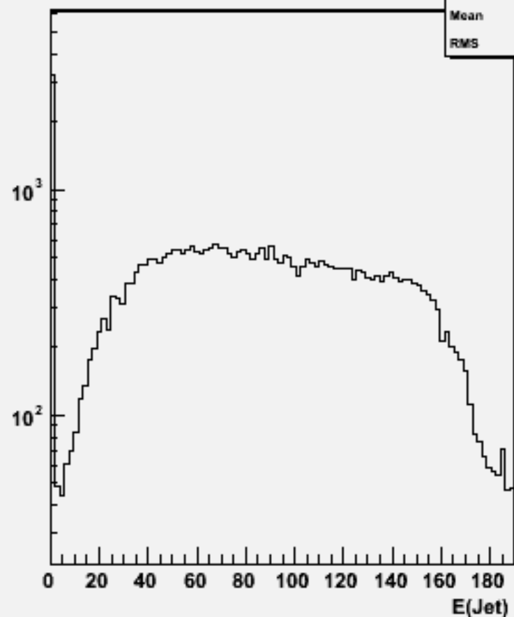
Jet energies(All jets)w102411 cce1e1bb_o
