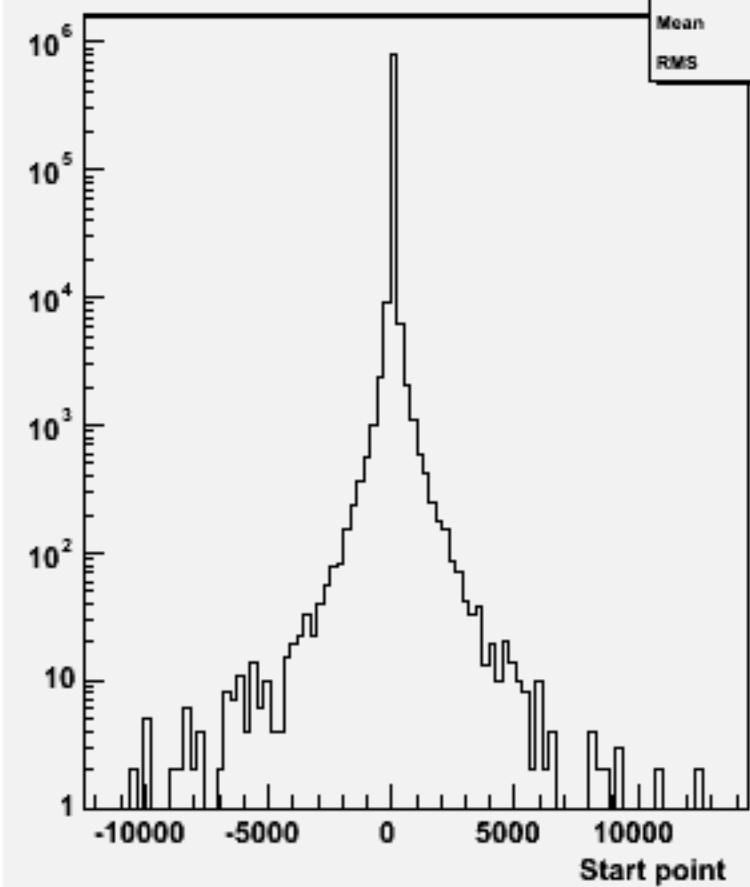
Start point Z : w102411 cce1e1bb_o
