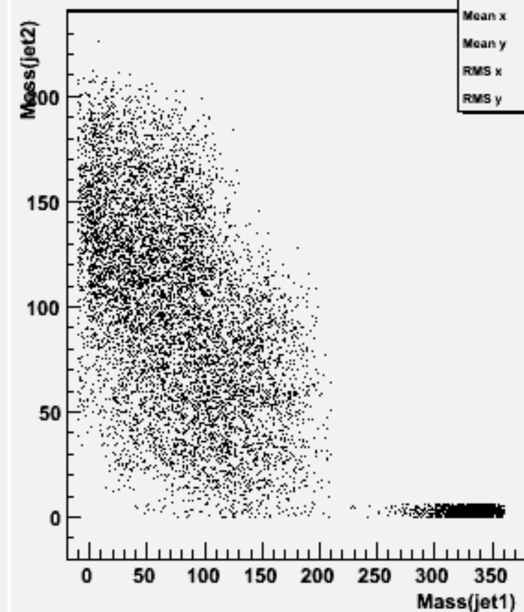
Jet mass for forced 2-jets : w102411 cce1e1bb_o
