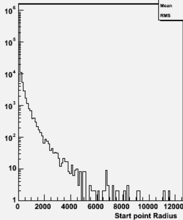
Start point R : w102411 cce1e1bb_o
