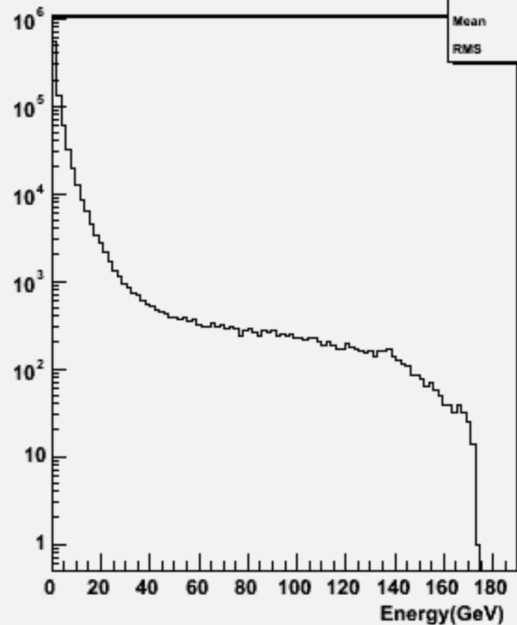
Particle Energy : w102411 cce1e1bb_o
