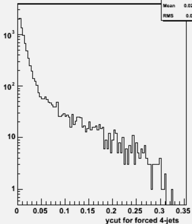
Ycut for 4-jets :w102411 cce1e1bb_o
