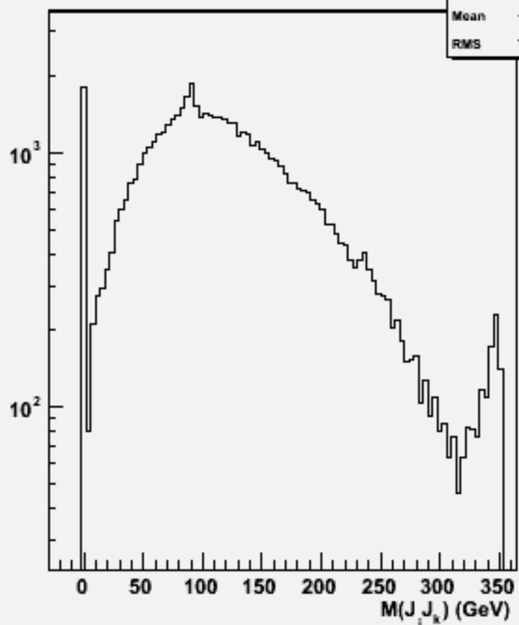
2jets mass(All comb)w102411 cce1e1bb_o
