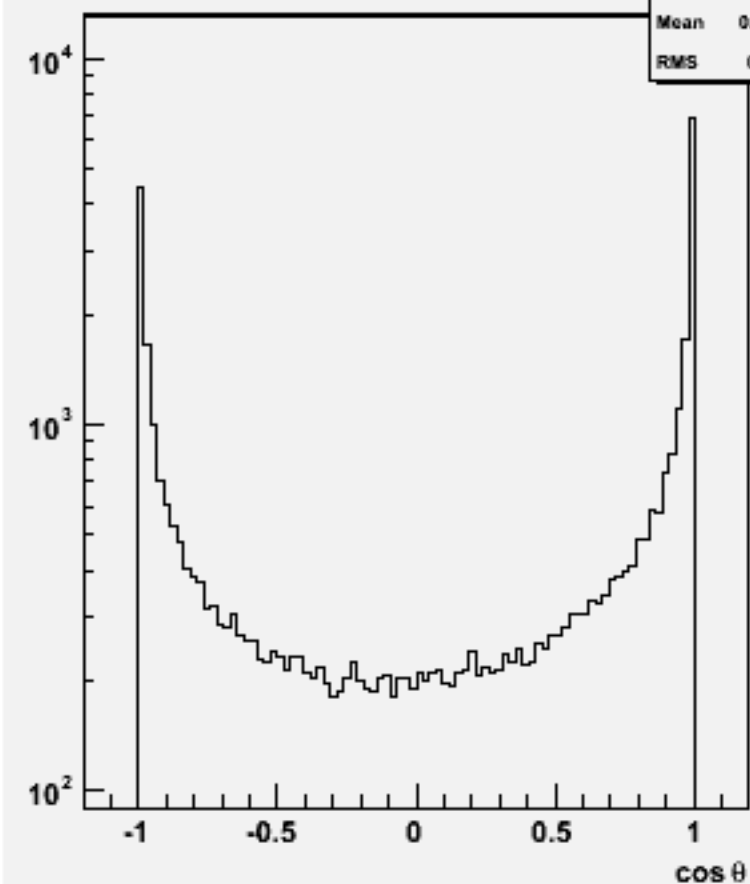
Jet cosθ (All jets)w102411 cce1e1bb_o
