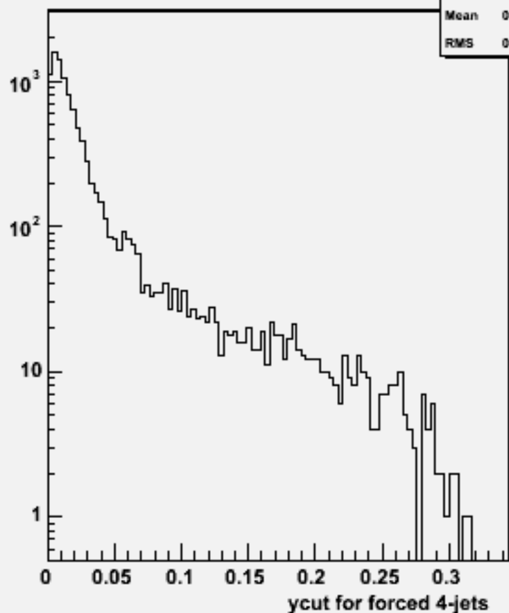
Ycut for 4-jets :w102409 cce1e1dd_o
