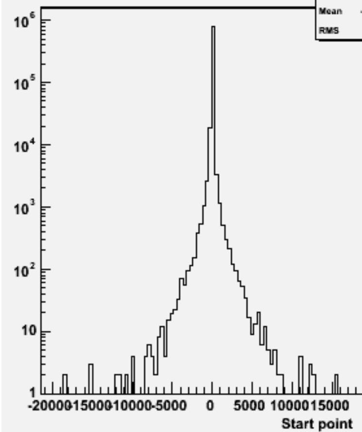
Start point Z : w102409 cce1e1dd_o
