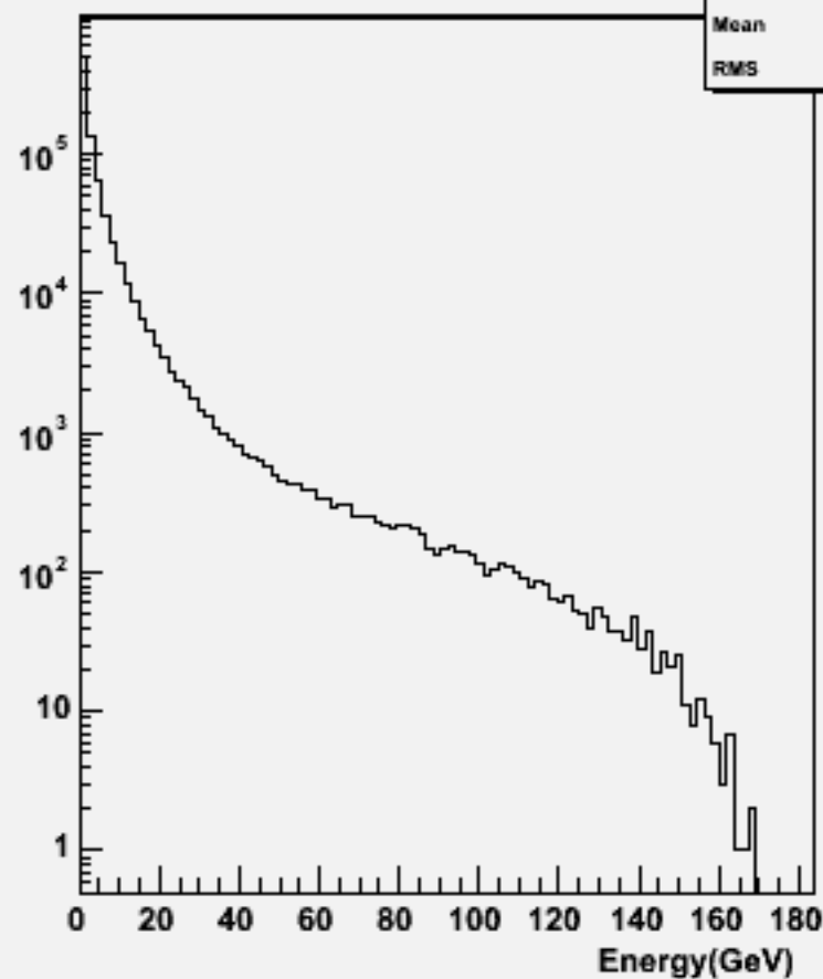
Particle Energy : w102409 cce1e1dd_o
