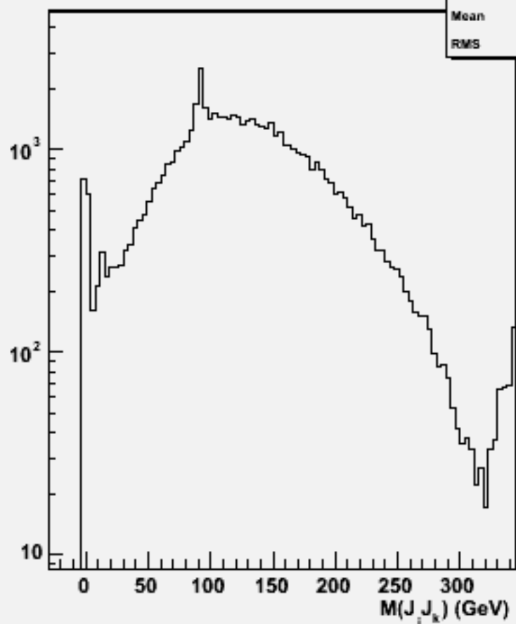
2jets mass(All comb)w102409 cce1e1dd_o
