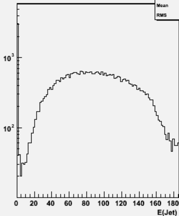
Jet energies(All jets)w102409 cce1e1dd_o
