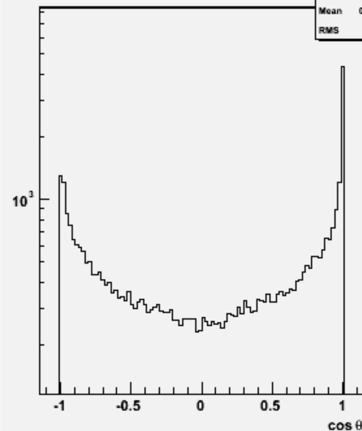
Jet cosθ (All jets)w102409 cce1e1dd_o
