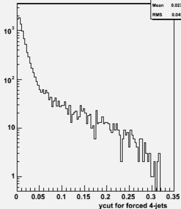
Ycut for 4-jets :w102407 cce1e1dd_o
