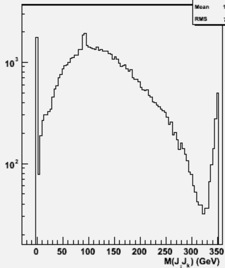
2jets mass(All comb)w102407 cce1e1dd_o
