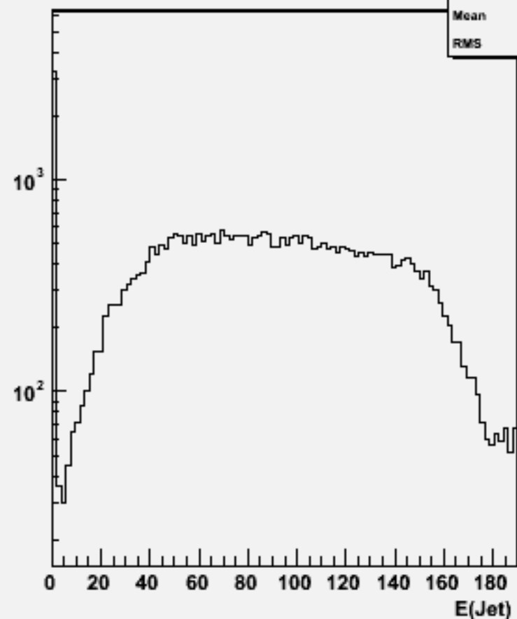
Jet energies(All jets)w102407 cce1e1dd_o
