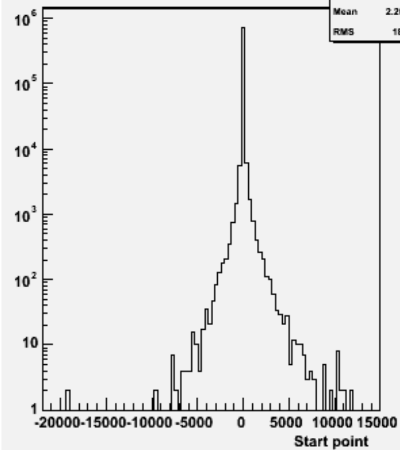
Start point Z : w102407 cce1e1dd_o
