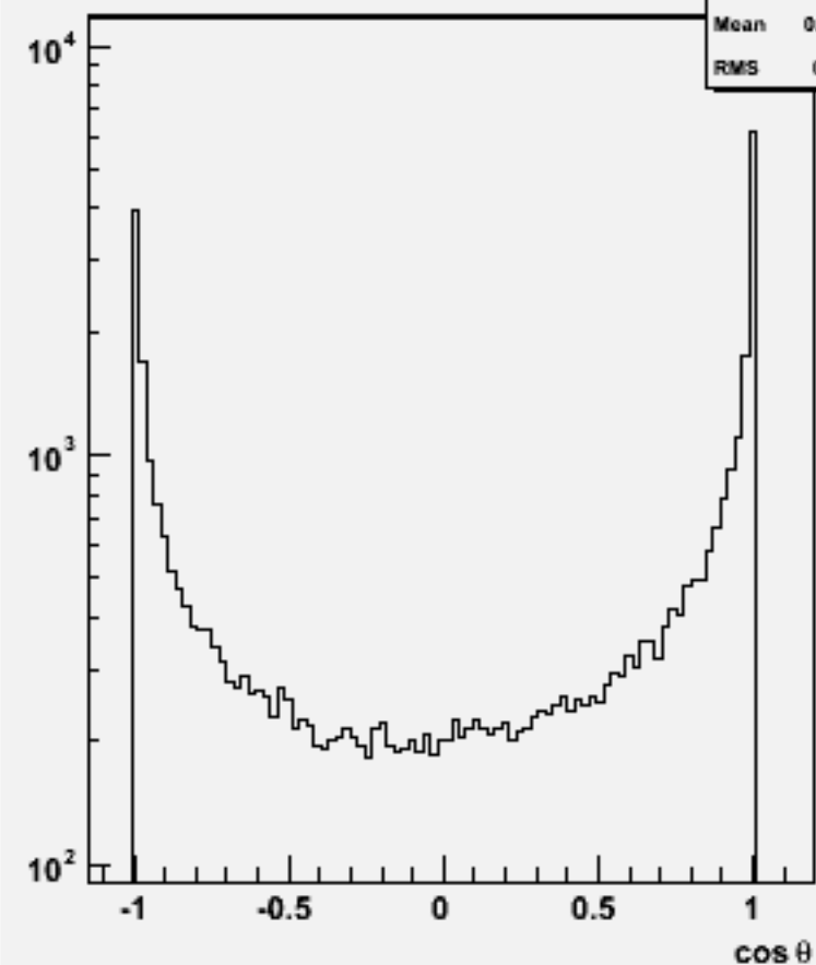
Jet cosθ (All jets)w102407 cce1e1dd_o
