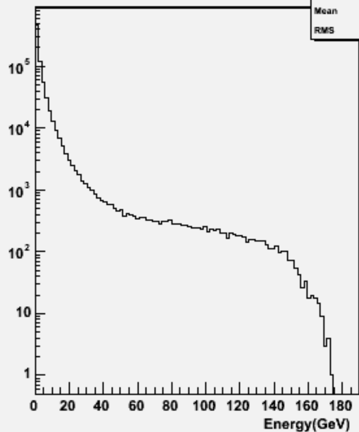
Particle Energy : w102407 cce1e1dd_o
