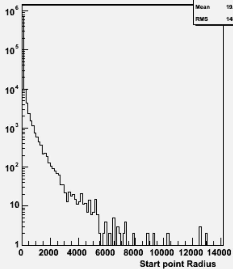
Start point R : w102407 cce1e1dd_o
