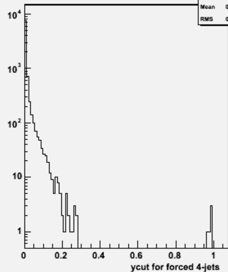
Ycut for 4-jets :w102406 cce1e1e3e3_o
