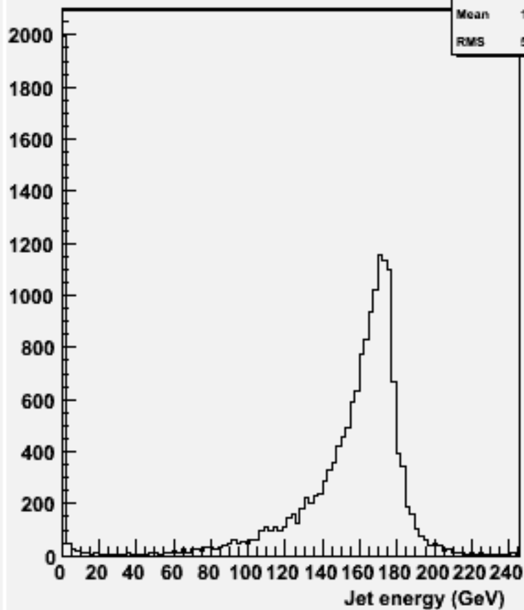
energy for 2-jets :w102406 cce1e1e3e3_o
