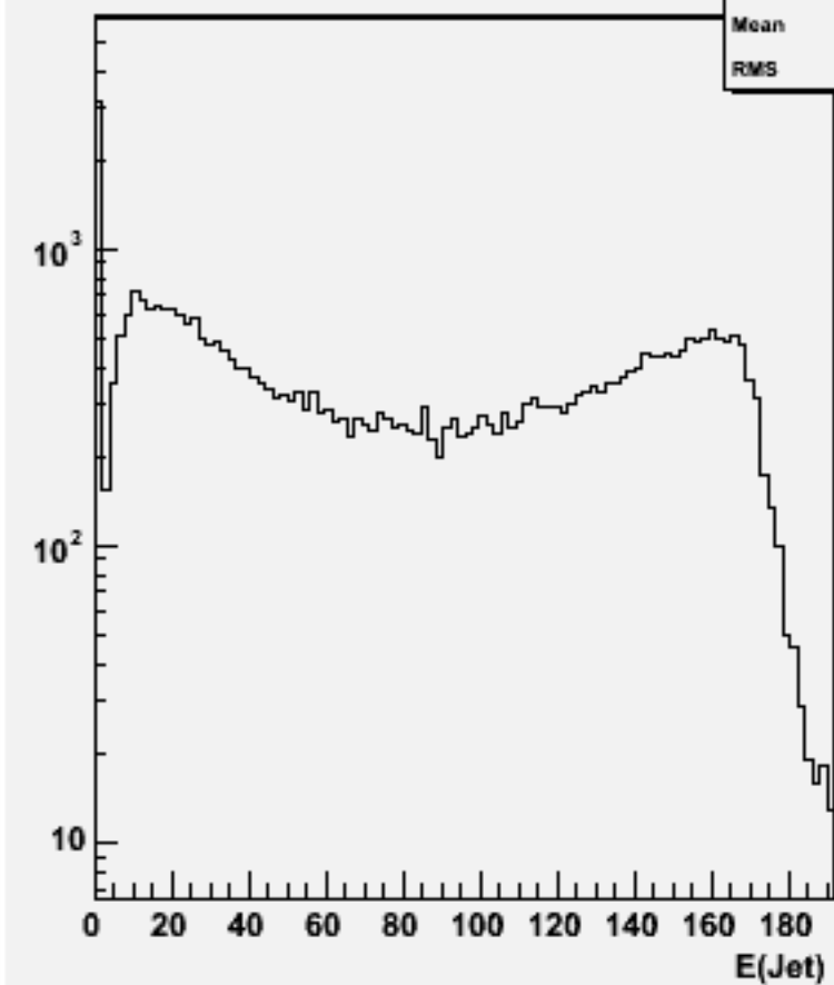
Jet energies(All jets)w102406 cce1e1e3e3_o
