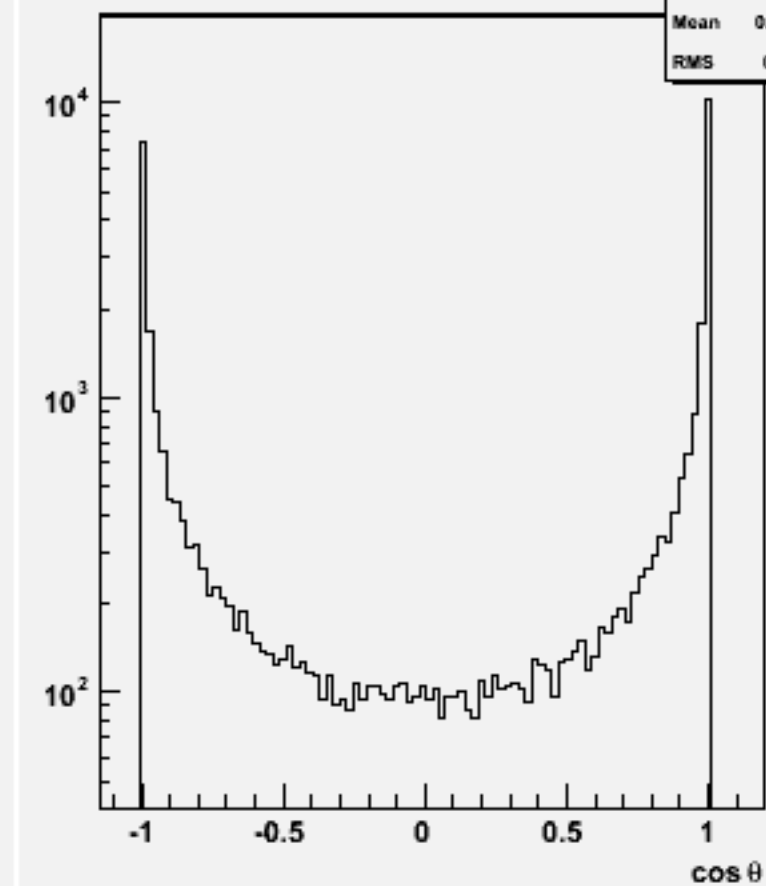
Jet cos \theta (All jets)w102406 cce1e1e3e3_o
