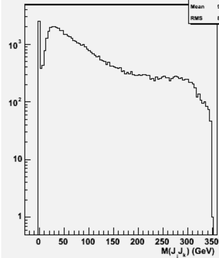
2jets mass(All comb)w102406 cce1e1e3e3_o
