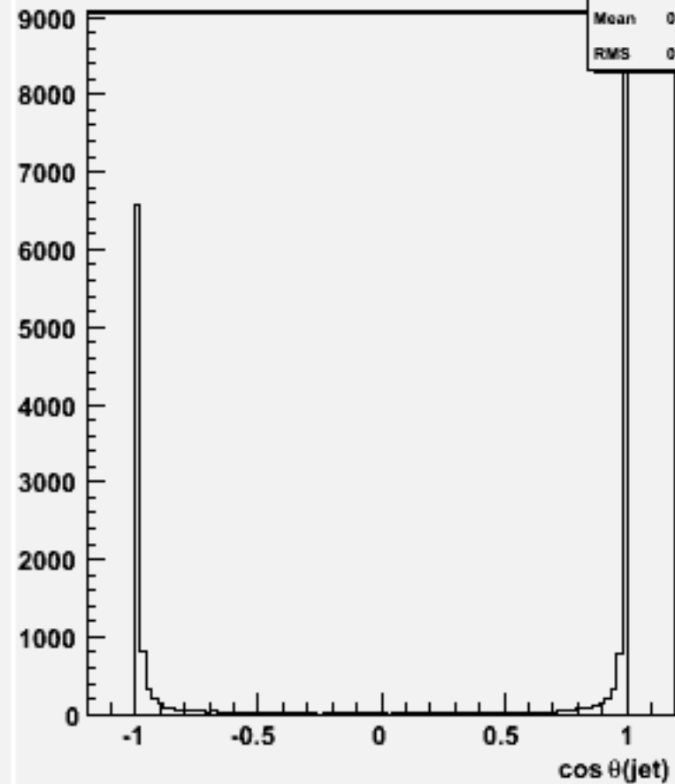
cos \theta for 2-jets :w102406 cce1e1e3e3_o
