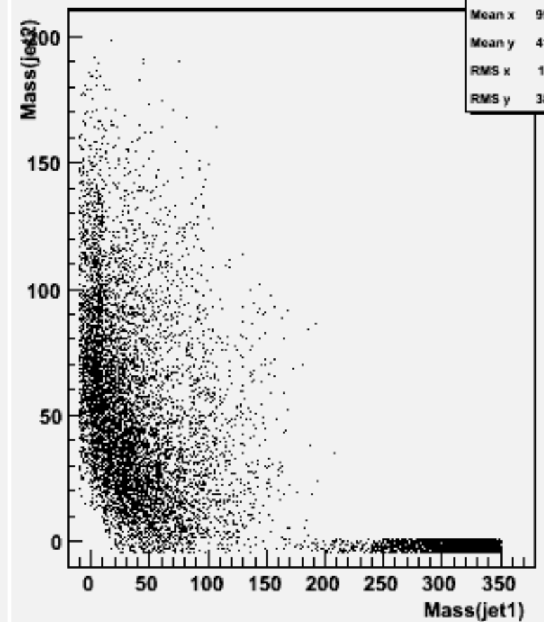
Jet mass for forced 2-jets : w102406 cce1e1e3e3_o
