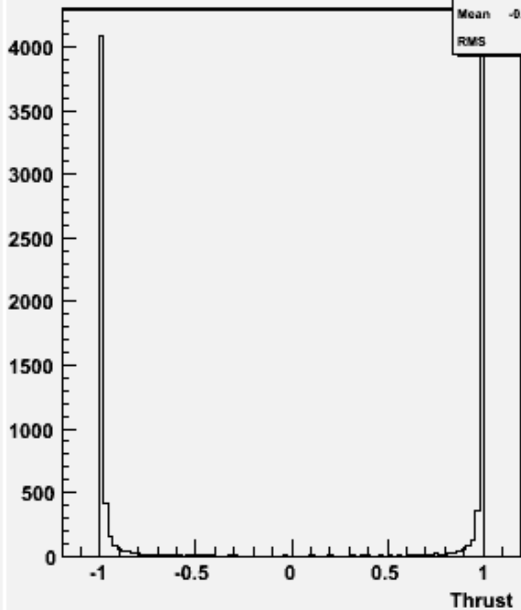
cos \Theta (thrust) w102406 cce1e1e3e3_o
