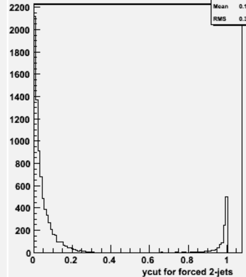
Ycut for 2-jets :w102406 cce1e1e3e3_o
