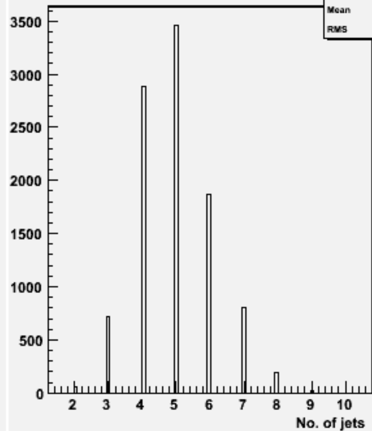
No. jets (ycut=0.001) : w102406 cce1e1e3e3_o
