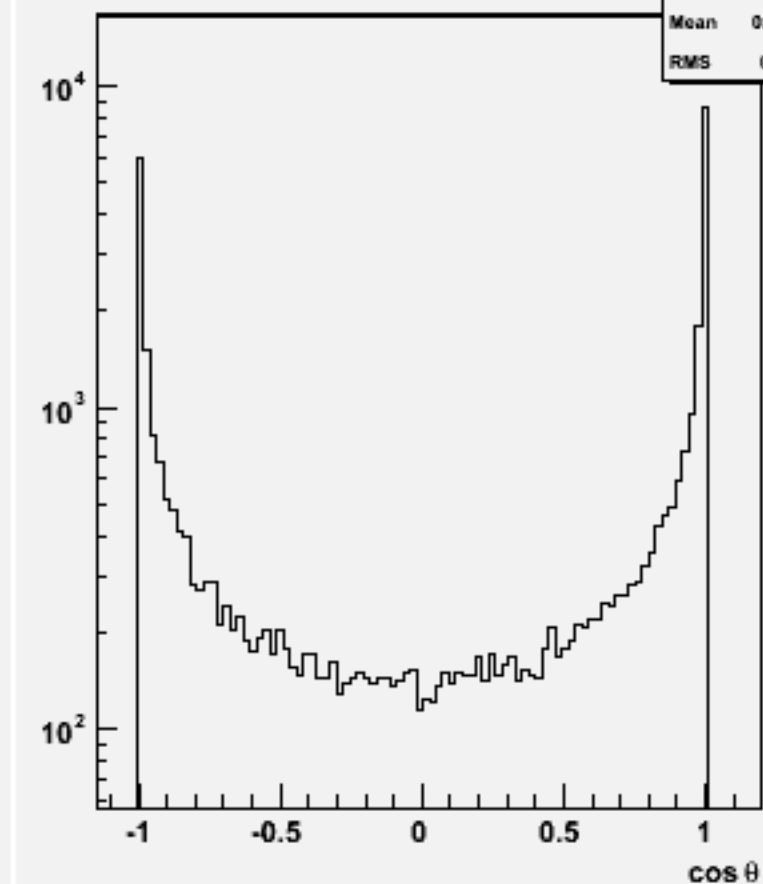
Jet cos \theta (All jets)w102405 cce1e1e3e3_o
