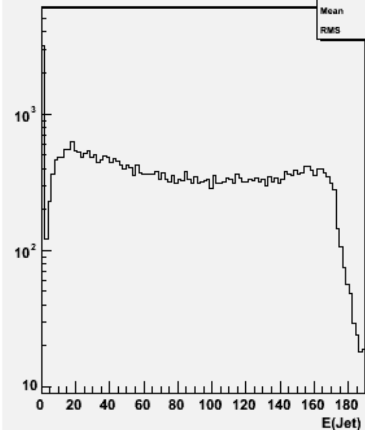
Jet energies(All jets)w102405 cce1e1e3e3_o
