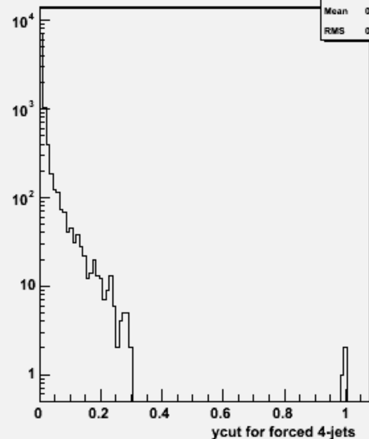
Ycut for 4-jets :w102405 cce1e1e3e3_o
