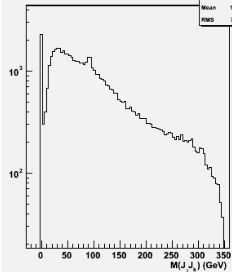
2jets mass(All comb)w102405 cce1e1e3e3_o
