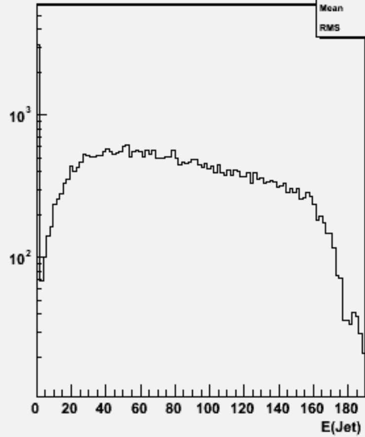
Jet energies(All jets)w102404 cce1e1e3e3_o
