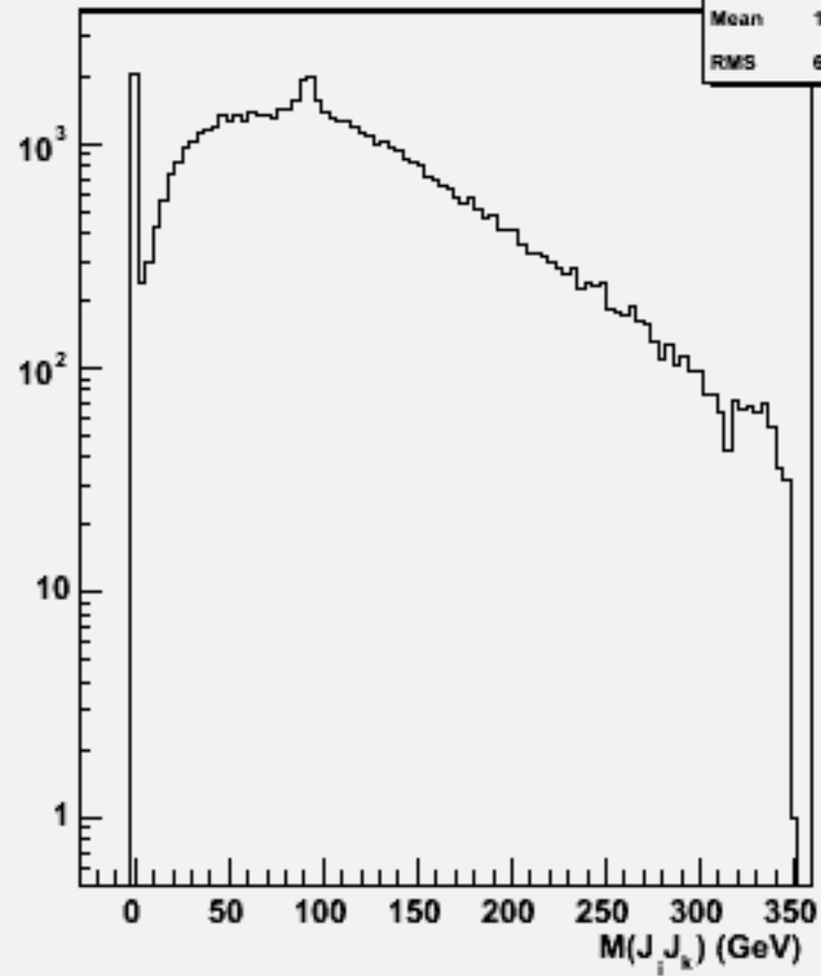
2jets mass(All comb)w102404 cce1e1e3e3_o
