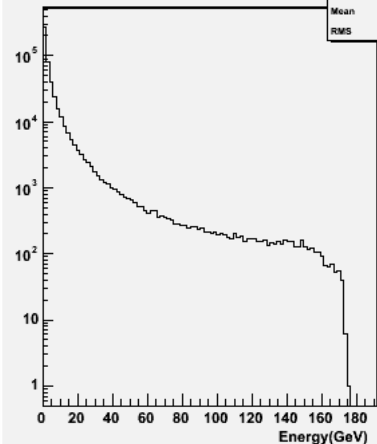
Particle Energy : w102404 cce1e1e3e3_o
