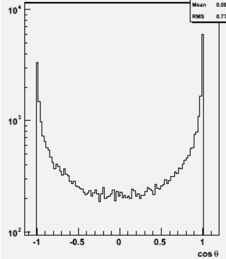
Jet cos \theta (All jets)w102404 cce1e1e3e3_o
