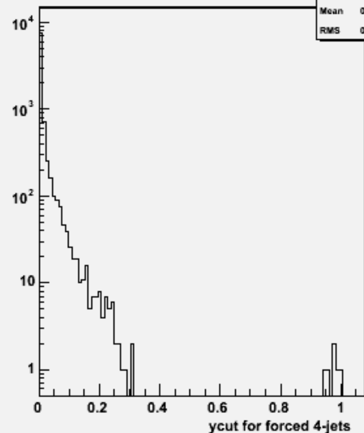
Ycut for 4-jets :w102403 cce1e1e3e3_o
