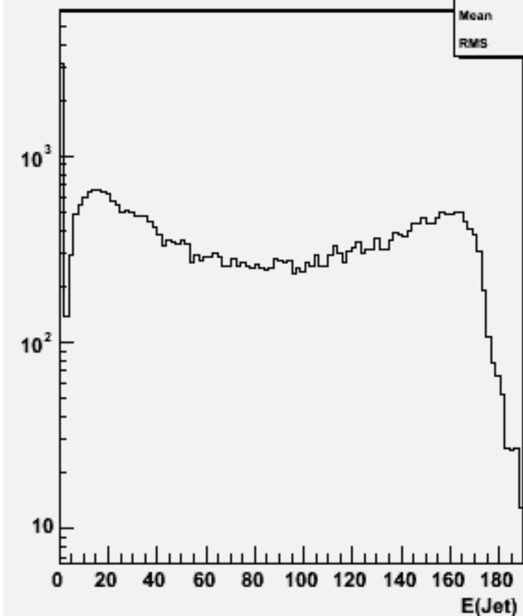
Jet energies(All jets)w102403 cce1e1e3e3_o
