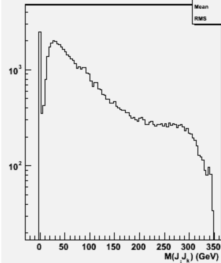
2jets mass(All comb)w102403 cce1e1e3e3_o
