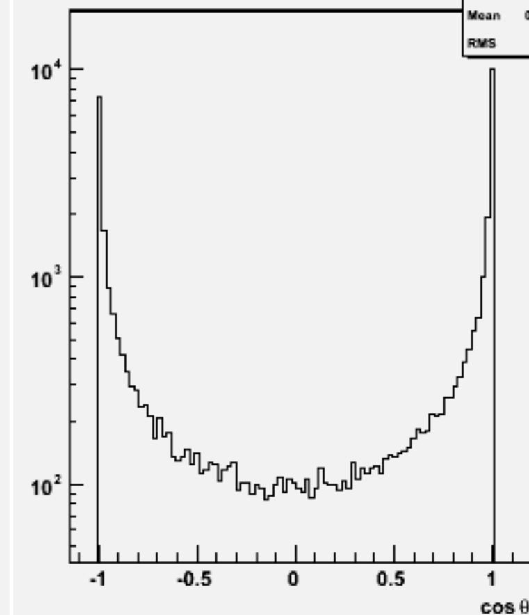
Jet cos \theta (All jets)w102403 cce1e1e3e3_o
