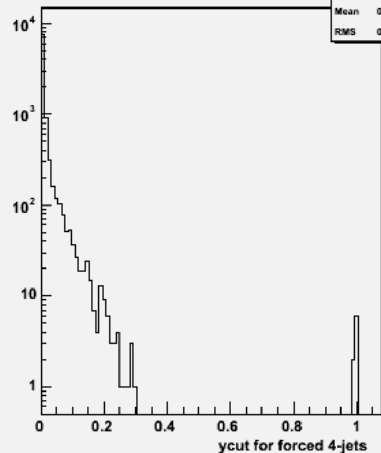
Ycut for 4-jets :w102402 cce1e1e2e2_o
