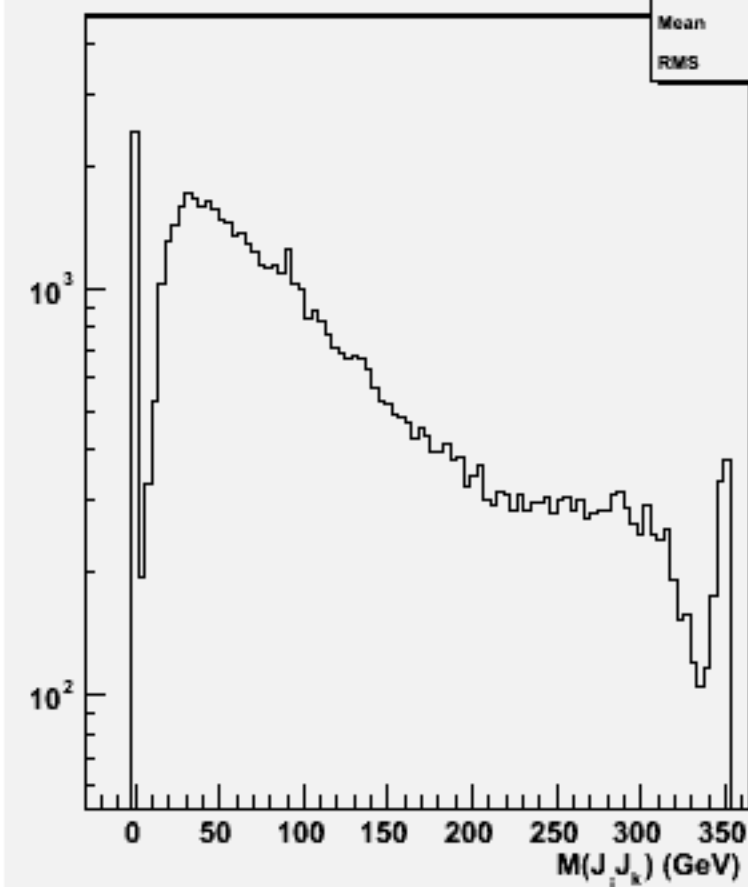
2jets mass(All comb)w102402 cce1e1e2e2_o
