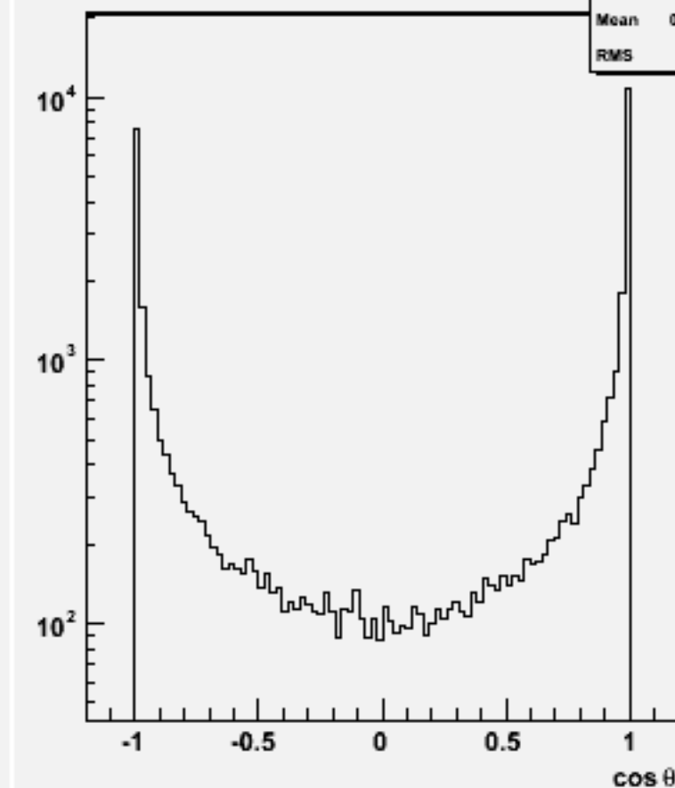
Jet cos \theta (All jets)w102402 cce1e1e2e2_o
