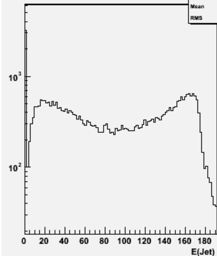
Jet energies(All jets)w102402 cce1e1e2e2_o
