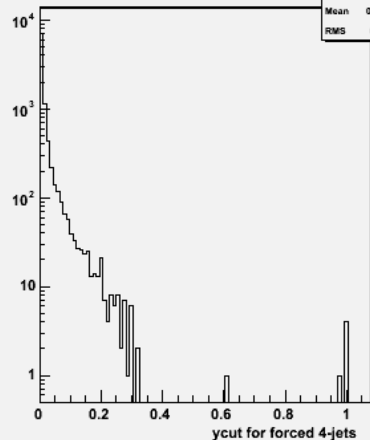
Ycut for 4-jets :w102401 cce1e1e2e2_o
