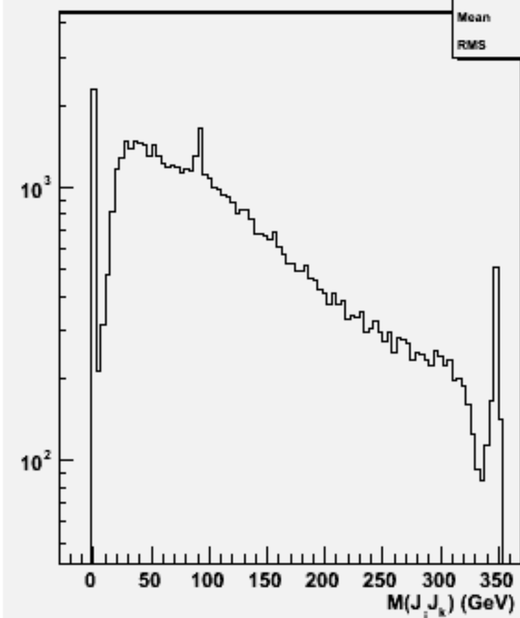
2jets mass(All comb)w102401 cce1e1e2e2_o
