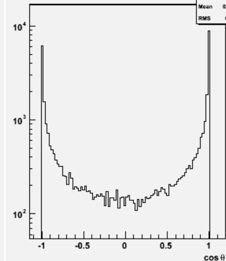
Jet cos \theta (All jets)w102401 cce1e1e2e2_o
