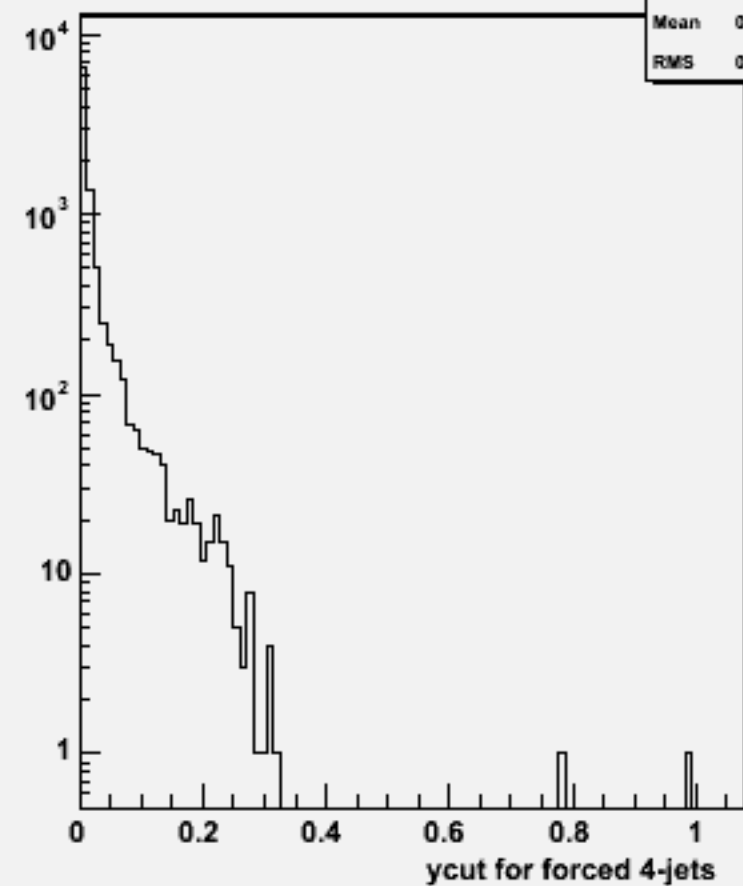
Ycut for 4-jets :w102400 cce1e1e2e2_o
