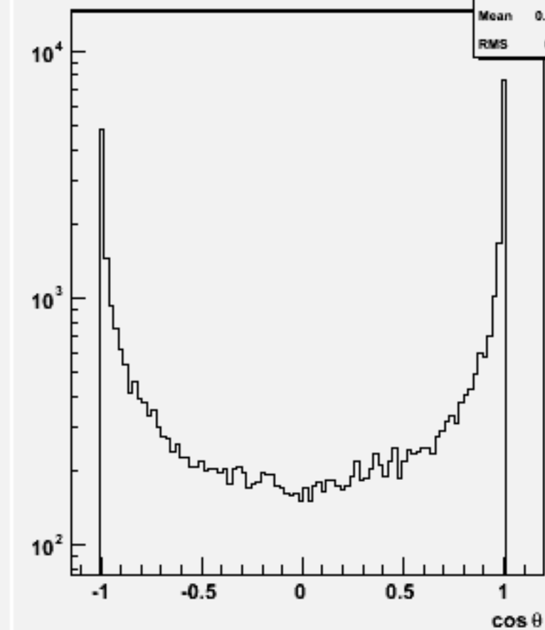
Jet cos \theta (All jets)w102400 cce1e1e2e2_o
