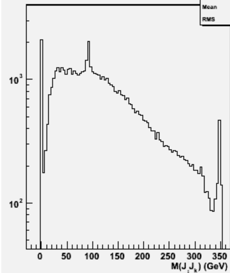
2jets mass(All comb)w102400 cce1e1e2e2_o
