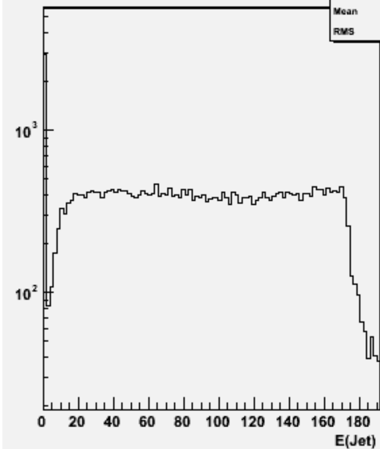
Jet energies(All jets)w102400 cce1e1e2e2_o
