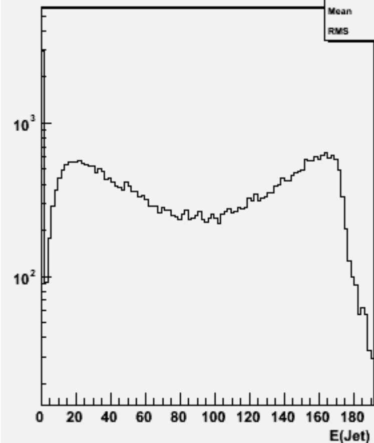
Jet energies(All jets)w102399 cce1e1e2e2_o
