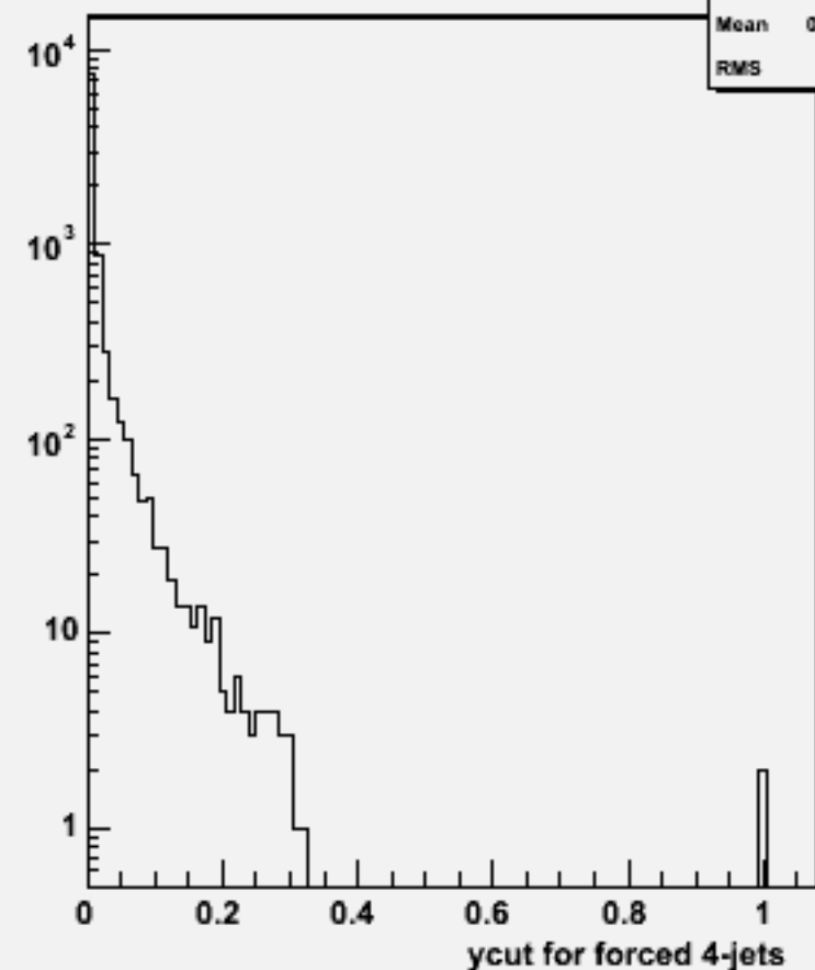
Ycut for 4-jets :w102399 cce1e1e2e2_o
