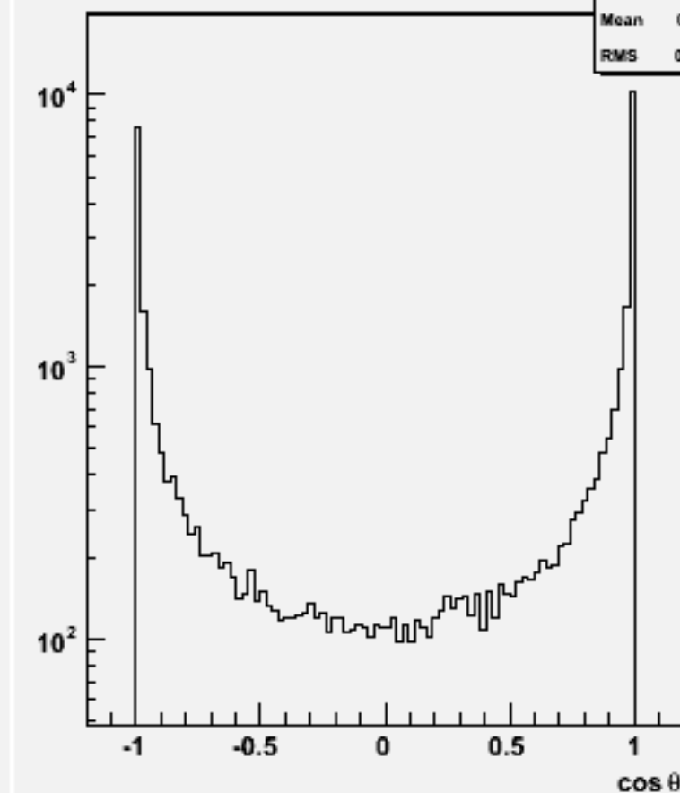
Jet cos \theta (All jets)w102399 cce1e1e2e2_o
