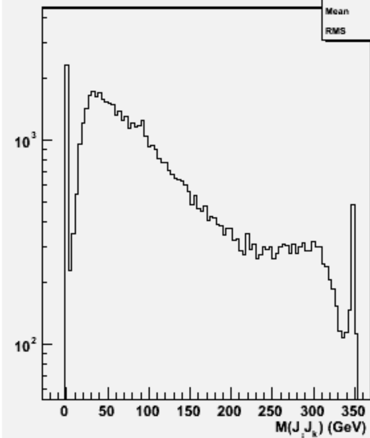
2jets mass(All comb)w102399 cce1e1e2e2_o
