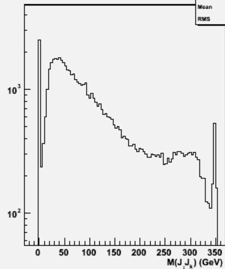
2jets mass(All comb)w102398 cce1e1e1e1_o
