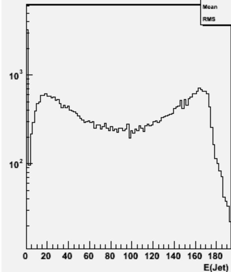
Jet energies(All jets)w102398 cce1e1e1e1_o
