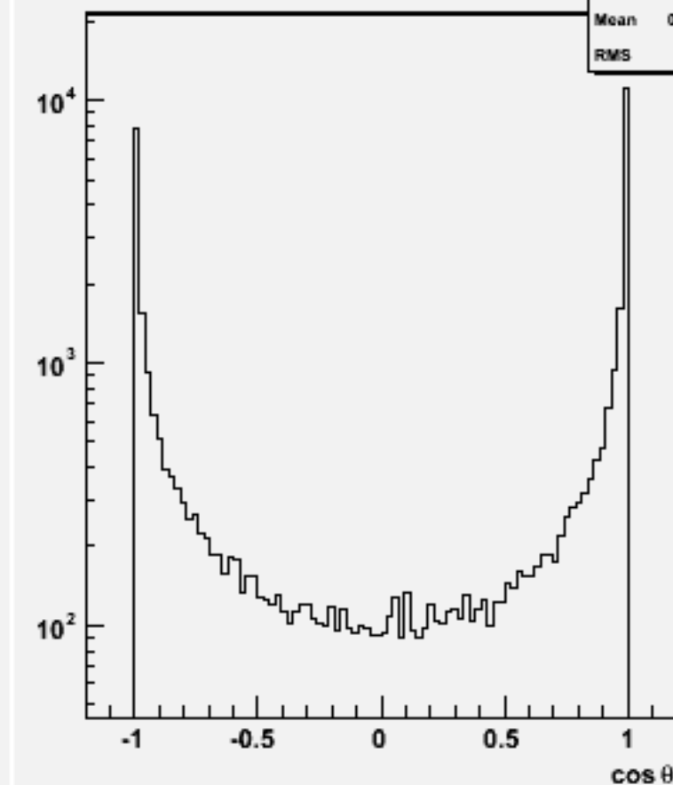
Jet cos \theta (All jets)w102398 cce1e1e1e1_o
