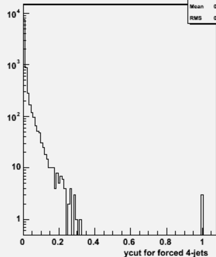
Ycut for 4-jets :w102398 cce1e1e1e1_o
