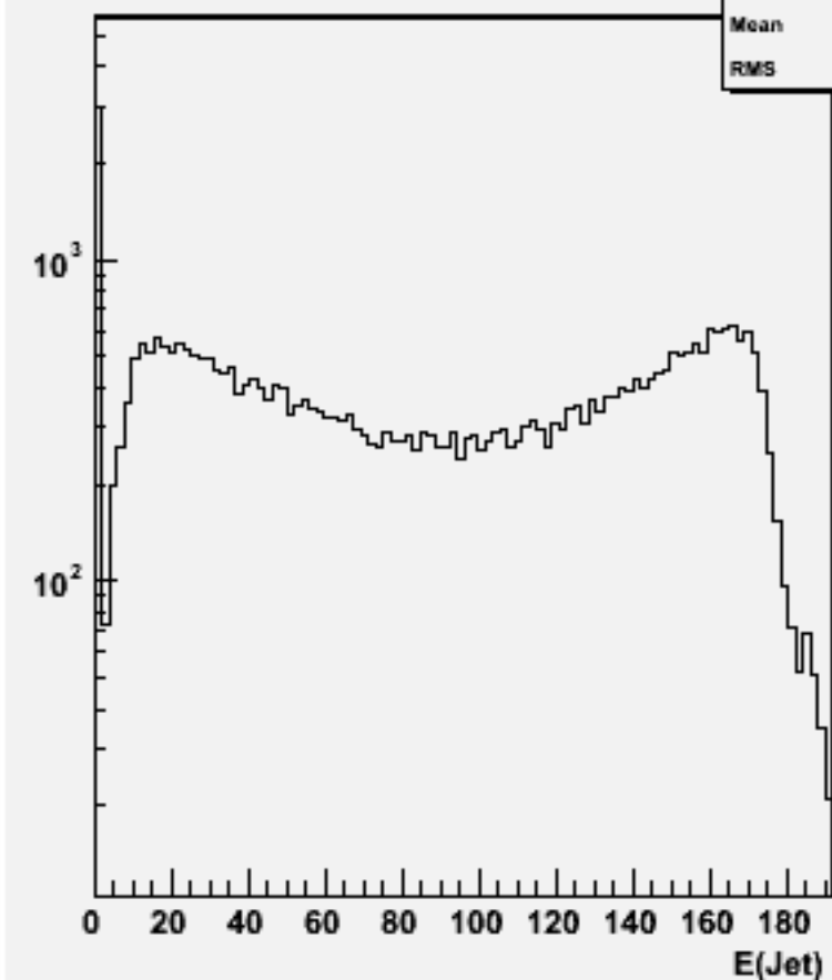
Jet energies(All jets)w102397 cce1e1e1e1_o
