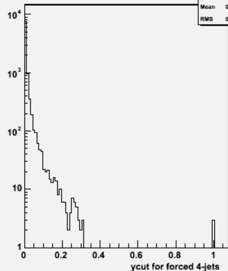
Ycut for 4-jets :w102397 cce1e1e1e1_o
