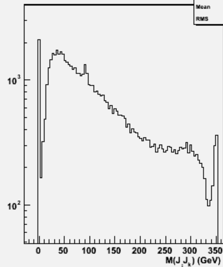
2jets mass(All comb)w102397 cce1e1e1e1_o
