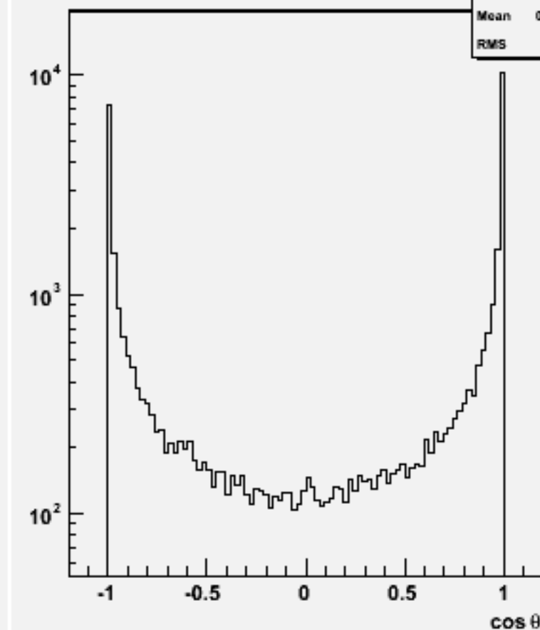
Jet cos \theta (All jets)w102397 cce1e1e1e1_o
