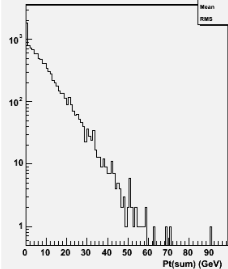
Pt Sum: w102393 uubbbb_o
