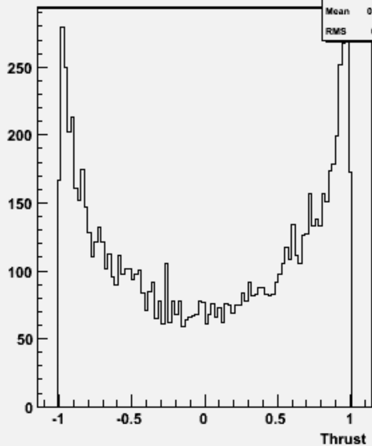
cos \Theta (thrust) w102393 uubbbb_o
