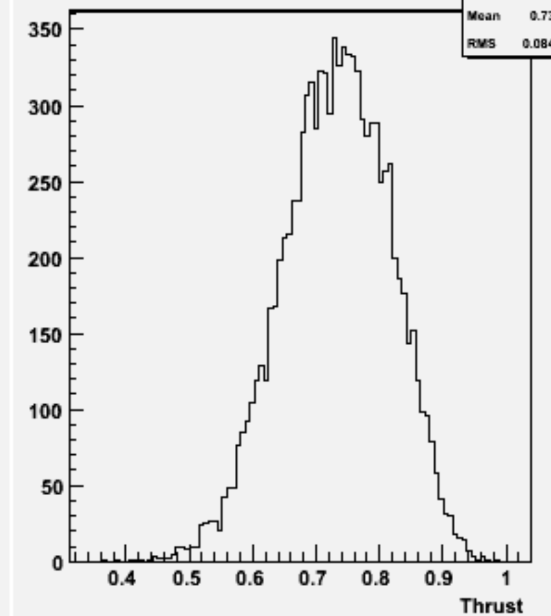
Thrust w102393 uubbbb_o
