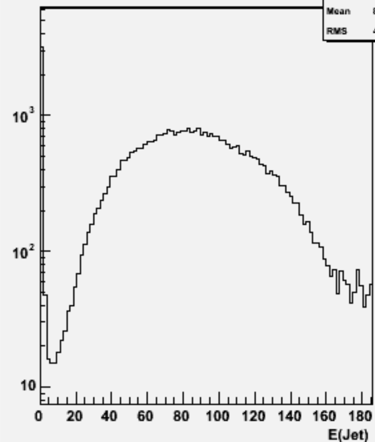
Jet energies(All jets)w102393 uubbbb_o
