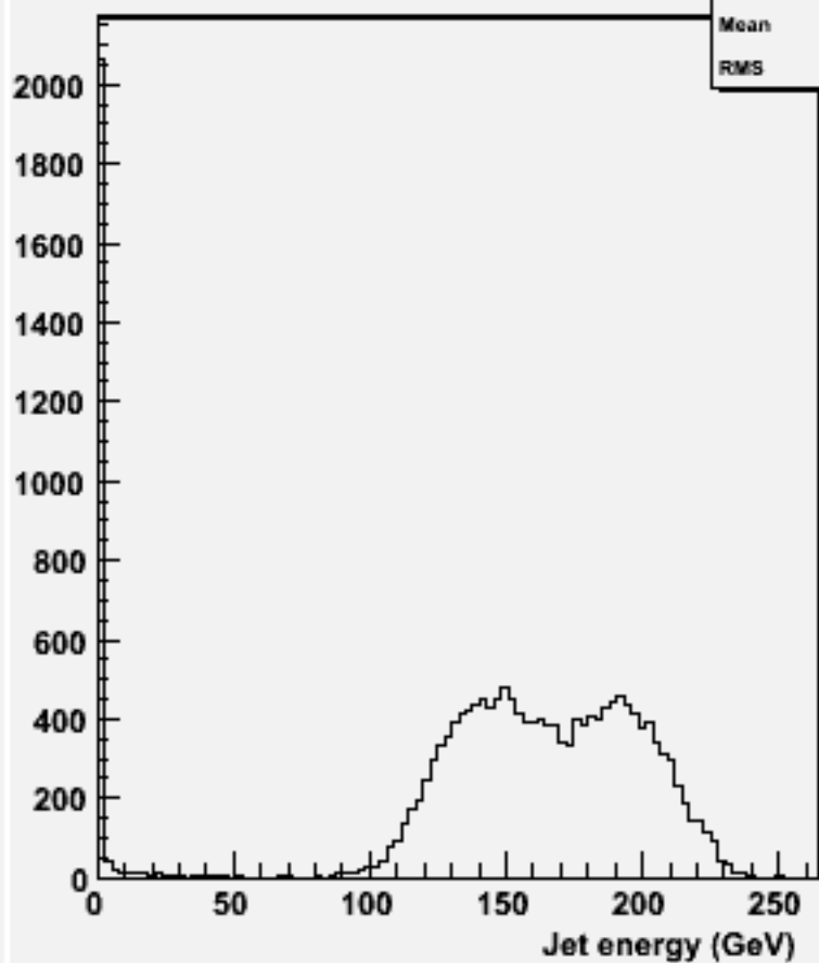
energy for 2-jets :w102393 uubbbb_o
