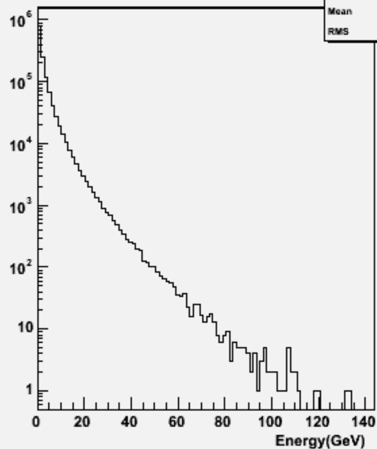
Particle Energy : w102393 uubbbb_o
