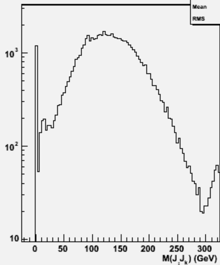
2jets mass(All comb)w102393 uubbbb_o
