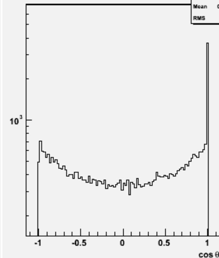
Jet cos \theta (All jets)w102393 uubbbb_o
