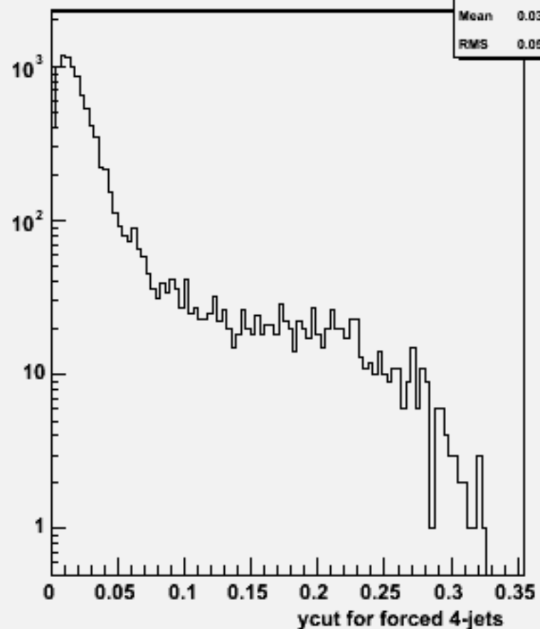
Ycut for 4-jets :w102393 uubbbb_o
