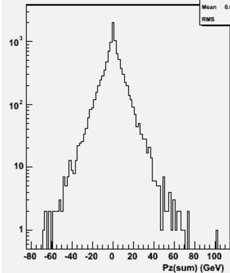
Pz Sum: w102393 uubbbb_o
