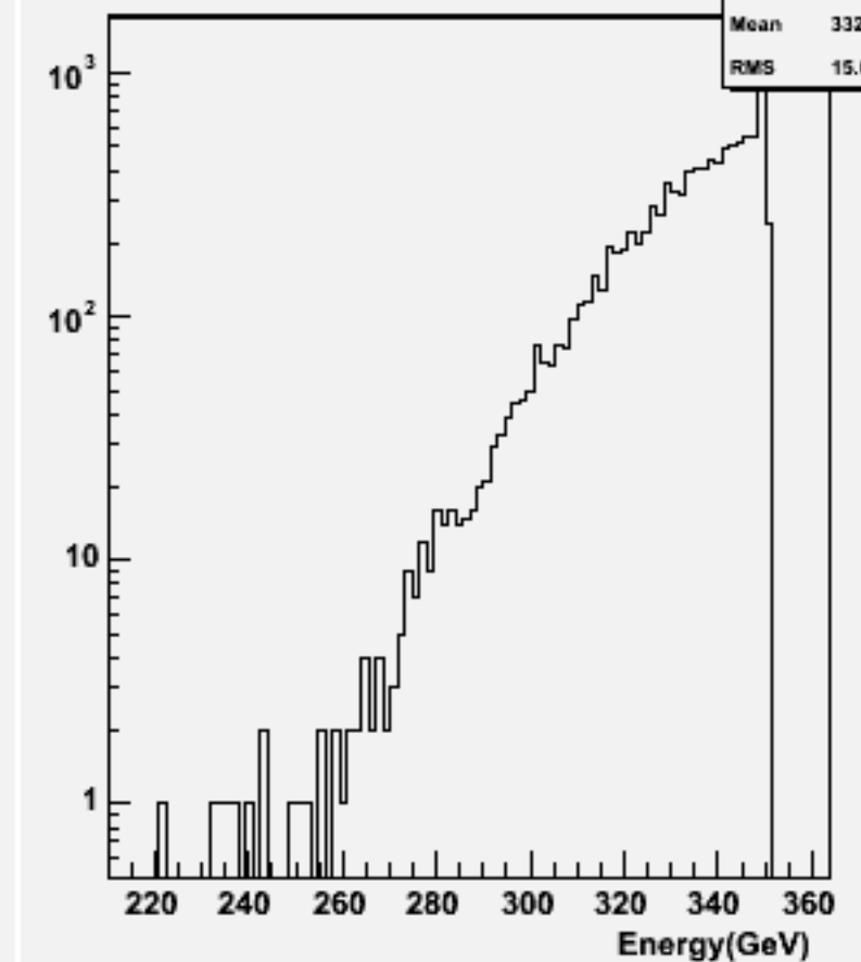
Total Energy (w/o \nu ): w102393 uubbbb_o
