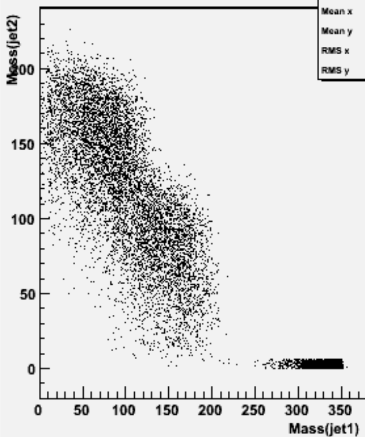
Jet mass for forced 2-jets : w102393 uubbbb_o
