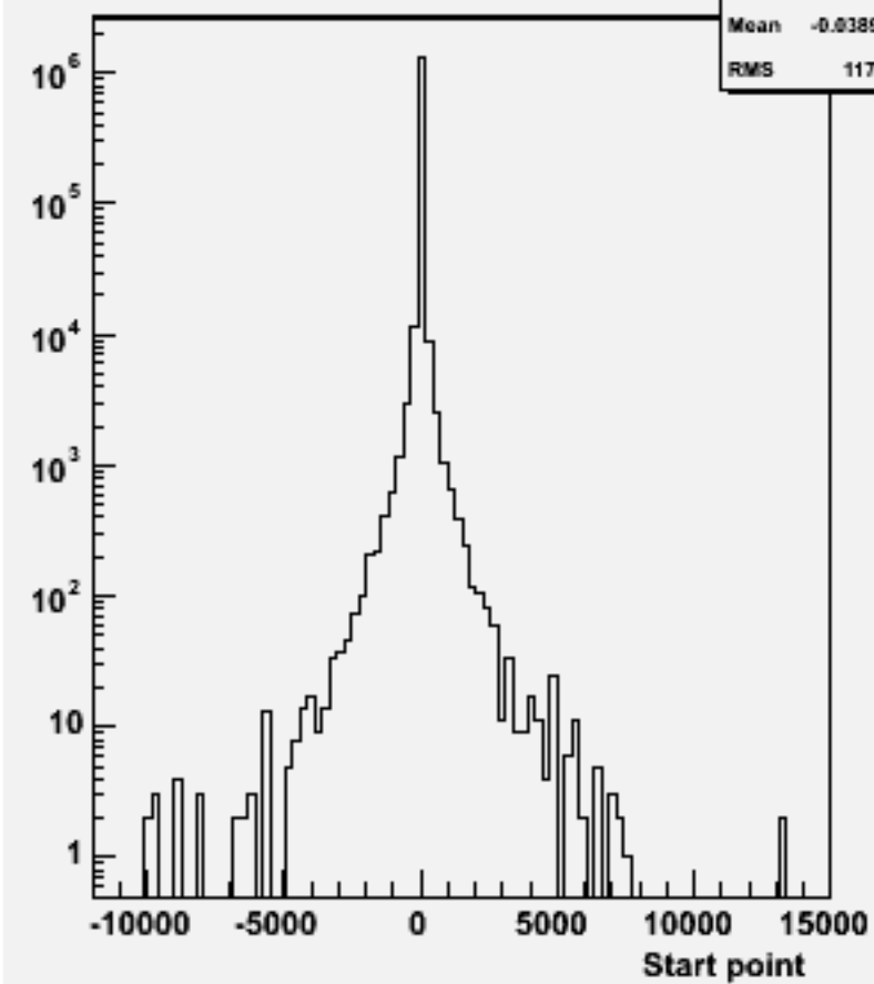
Start point Z : w102393 uubbbb_o
