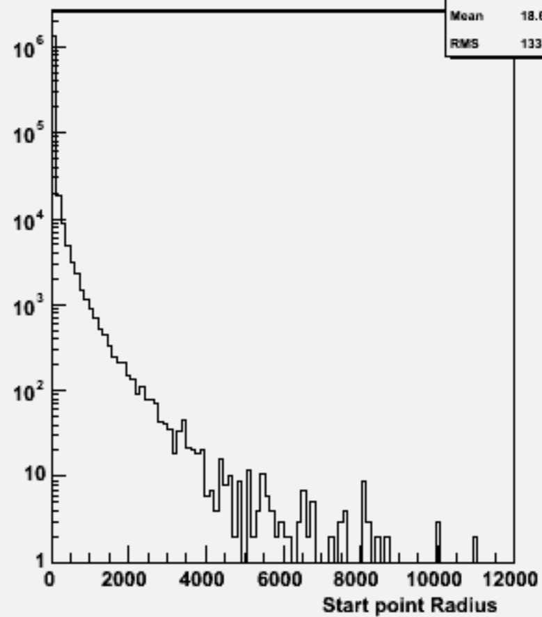
Start point R : w102393 uubbbb_o
