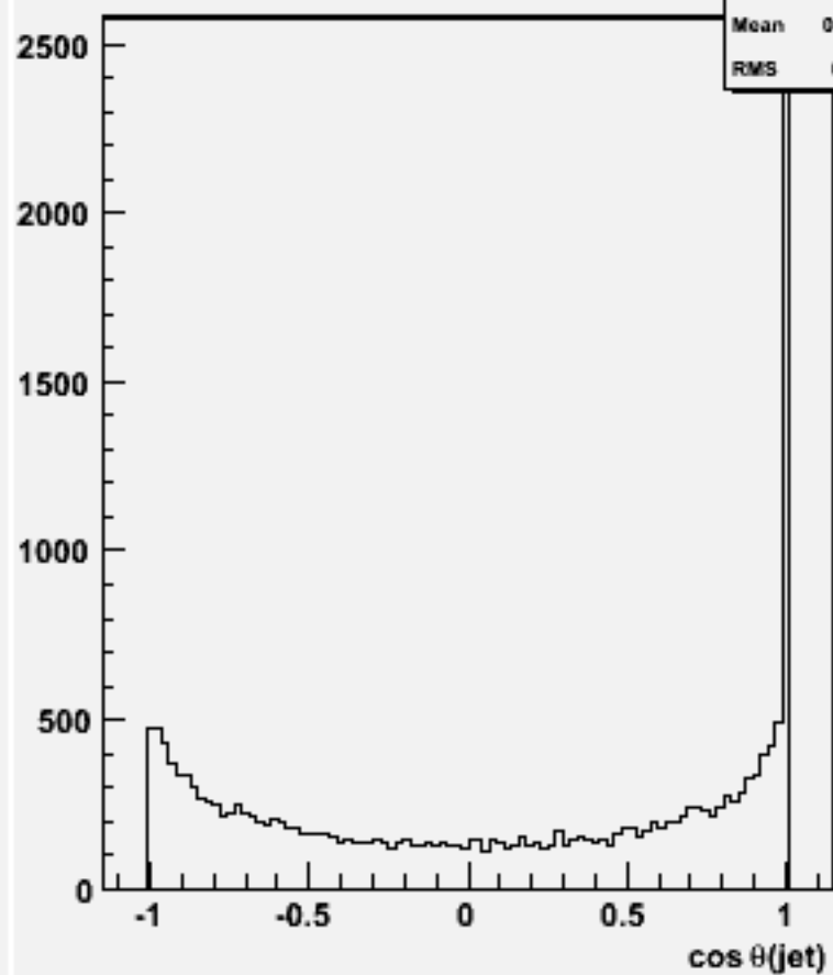
cos \Theta for 2-jets :w102393 uubbbb_o
