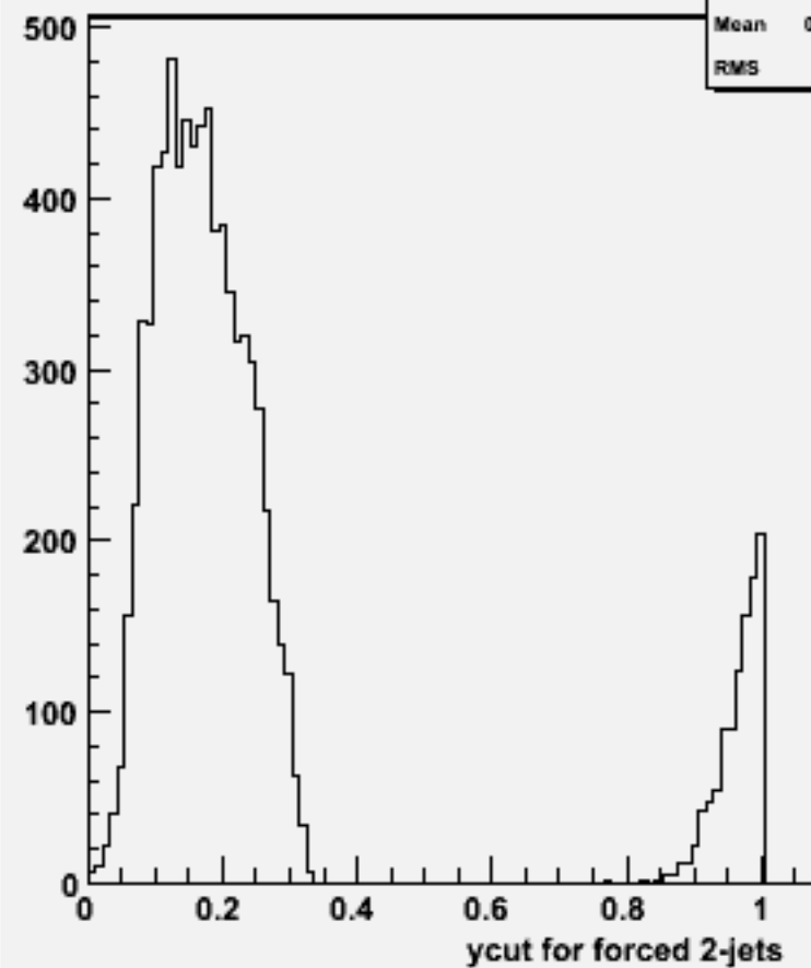
Ycut for 2-jets :w102393 uubbbb_o
