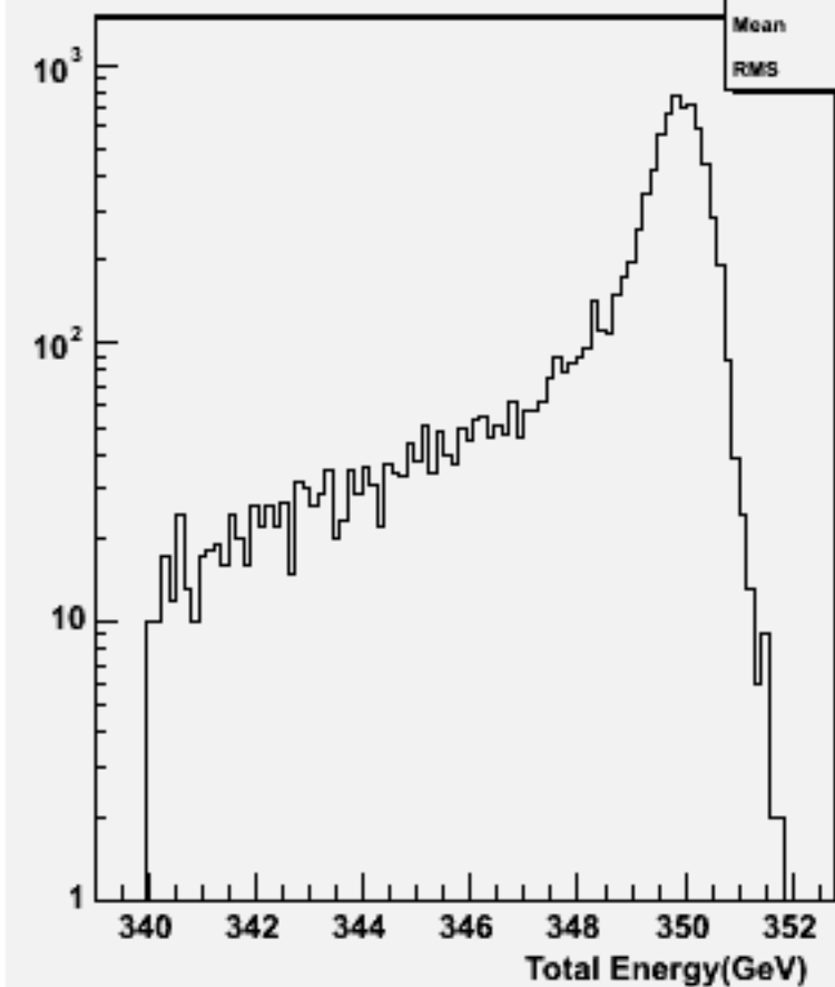
Total Energy (inc. \nu ): w102393 uubbbb_o
