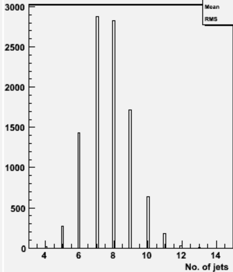
No. jets (ycut=0.001) : w102393 uubbbb_o
