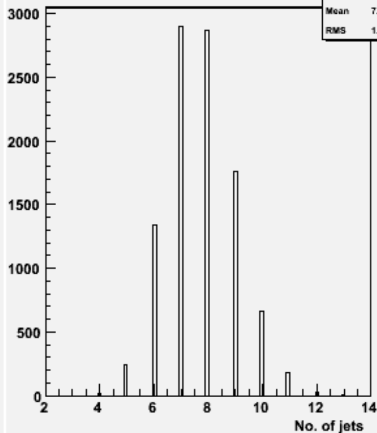
No. jets (ycut=0.001) : w102389 uussbb_o
