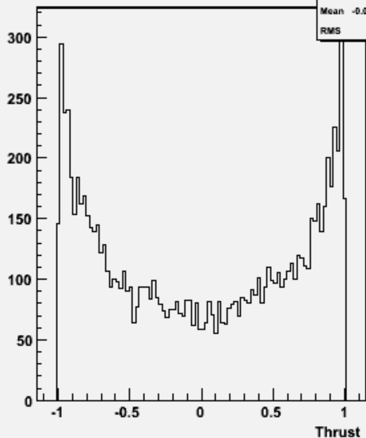
cos \Theta (thrust) w102389 uussbb_o
