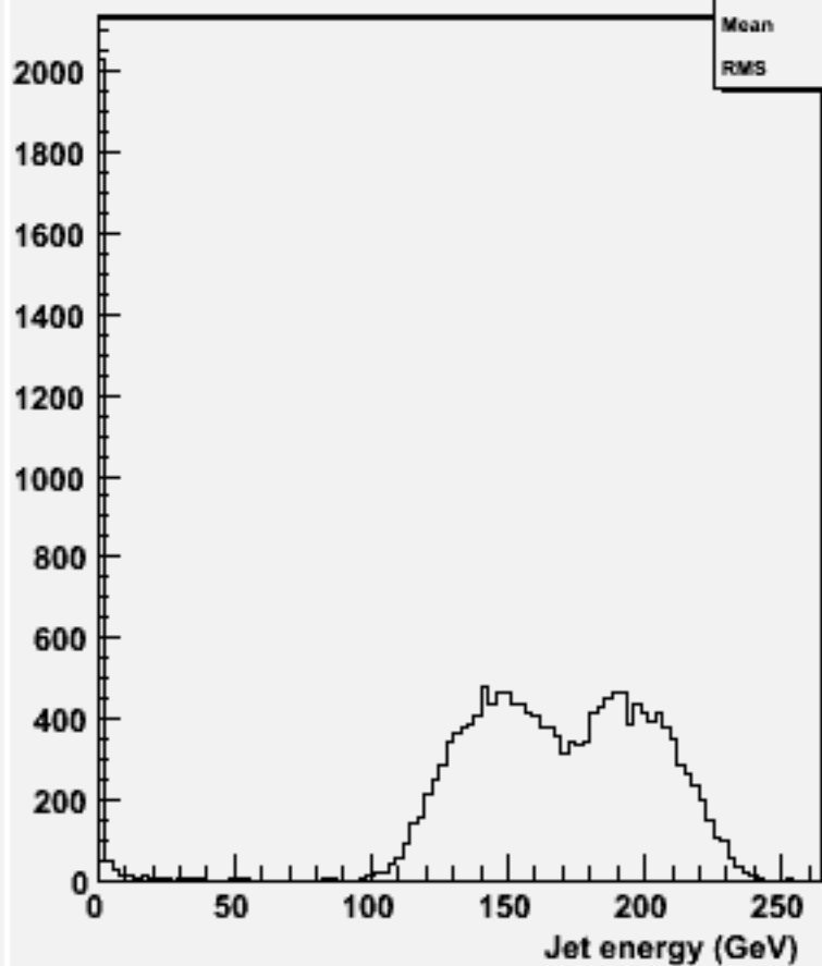
energy for 2-jets :w102389 uussbb_o
