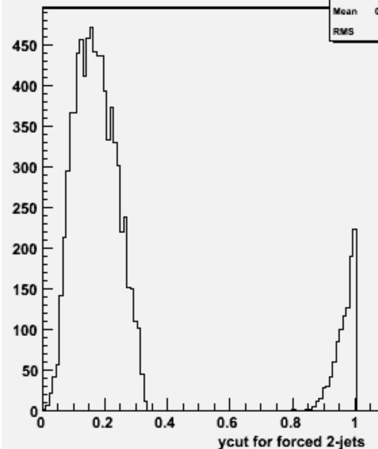
Ycut for 2-jets :w102389 uussbb_o
