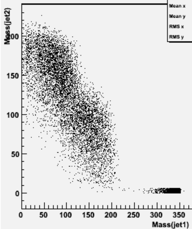
Jet mass for forced 2-jets : w102389 uussbb_o
