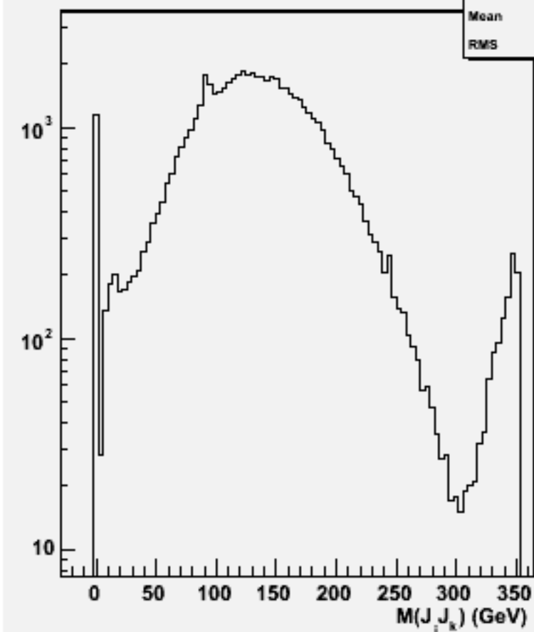
2jets mass(All comb)w102389 uussbb_o
