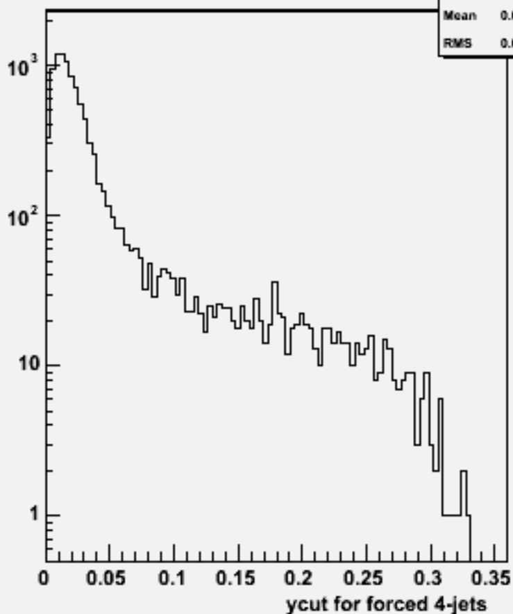
Ycut for 4-jets :w102389 uussbb_o
