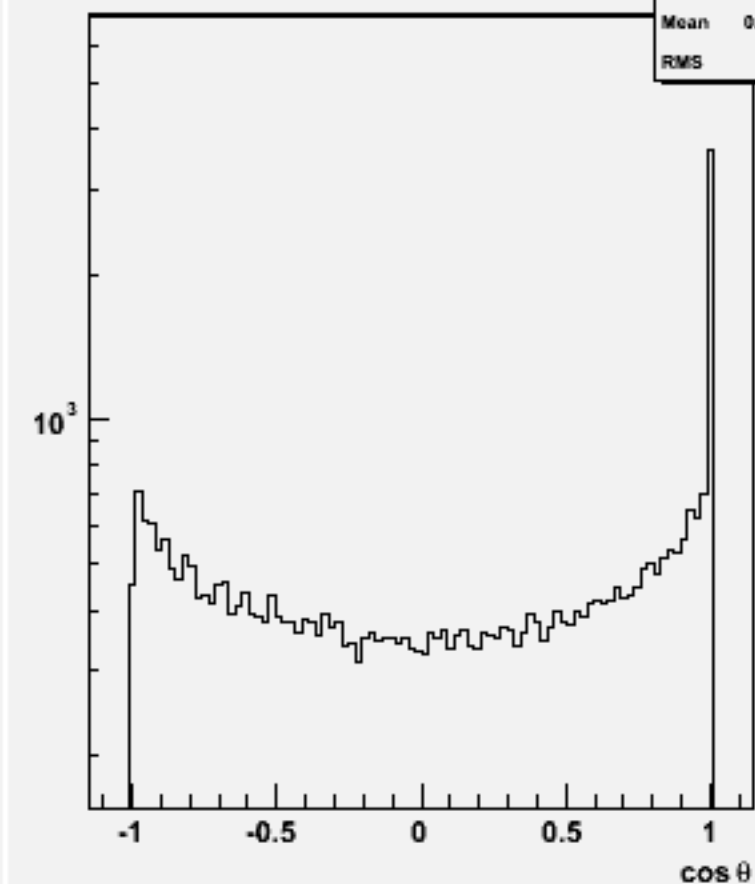
Jet cos \theta (All jets)w102389 uussbb_o
