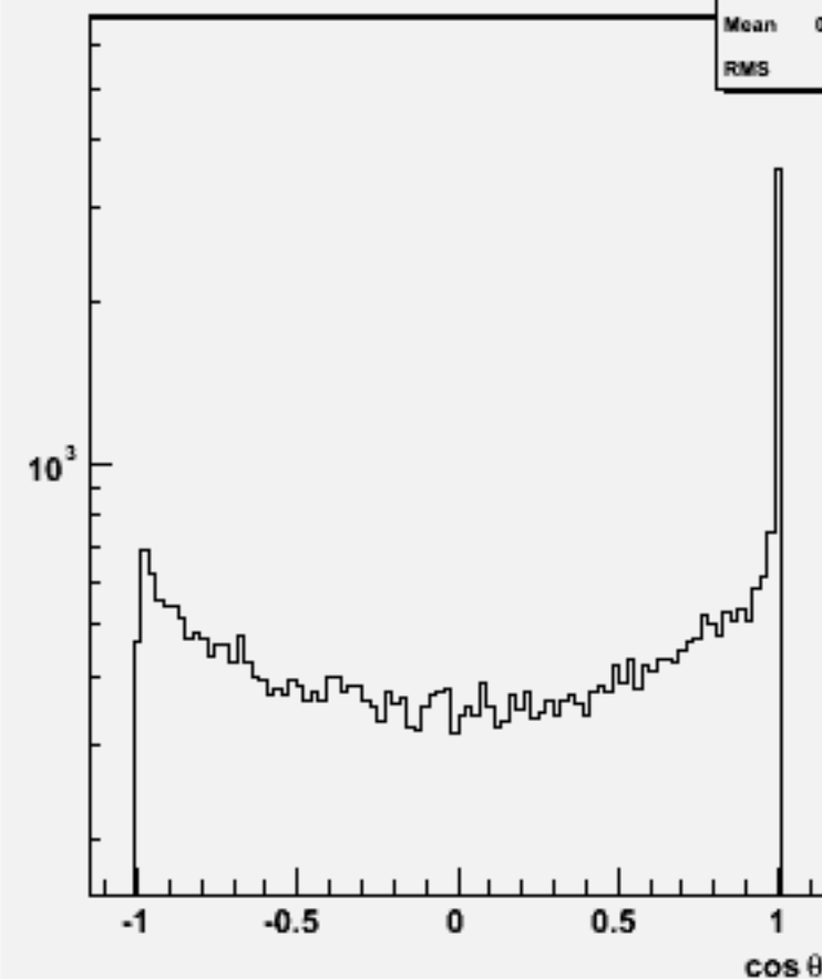
Jet cos \theta (All jets)w102385 uussss_o
