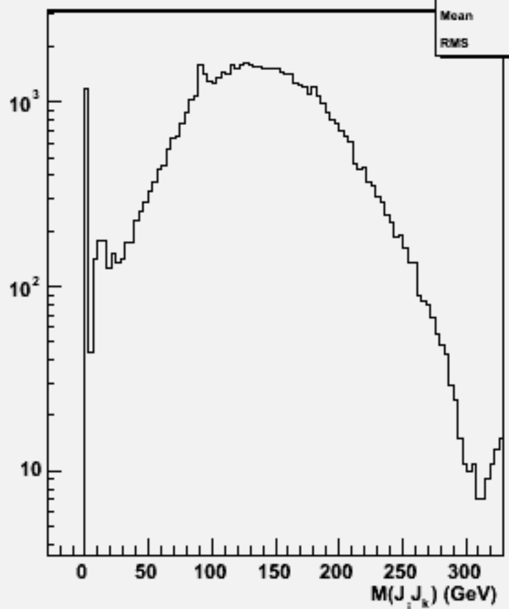
2jets mass(All comb)w102385 uussss_o
