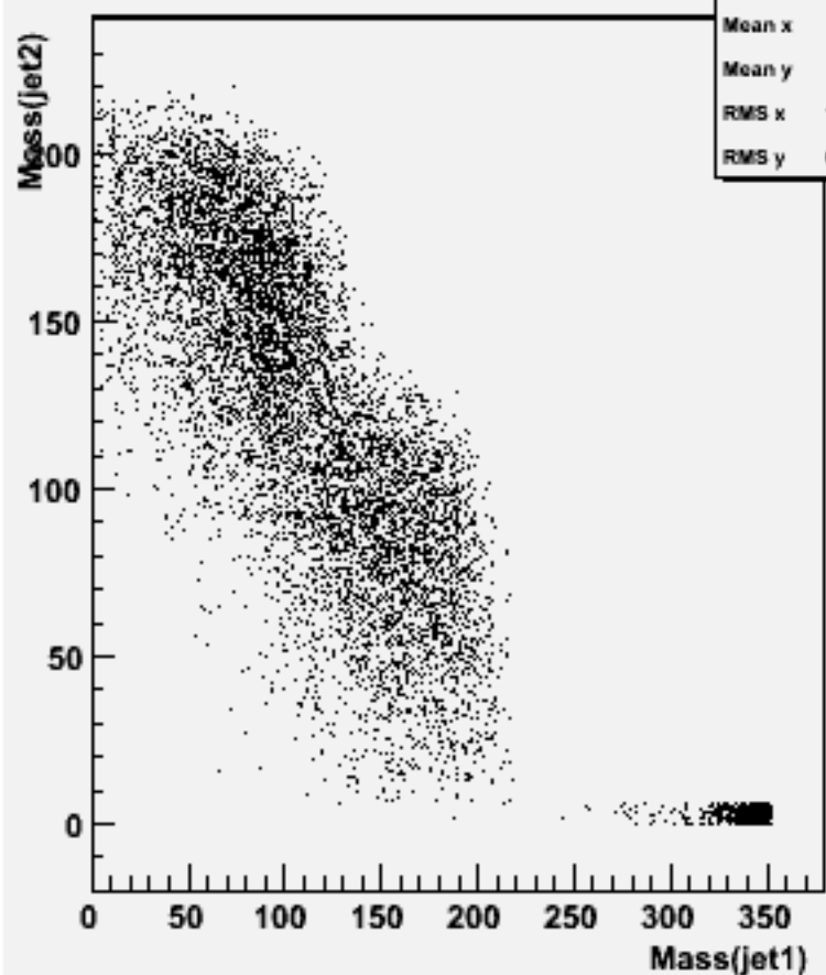
Jet mass for forced 2-jets : w102385 uussss_o
