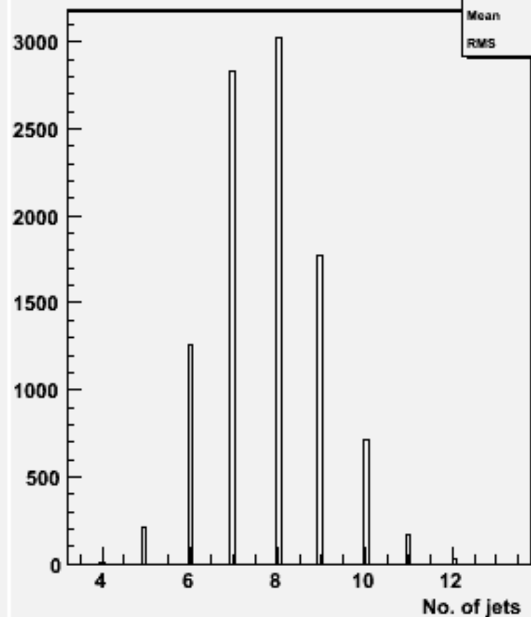
No. jets (ycut=0.001) : w102385 uussss_o
