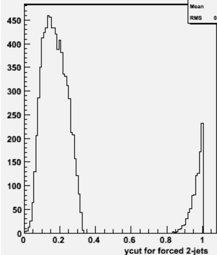
Ycut for 2-jets :w102385 uussss_o
