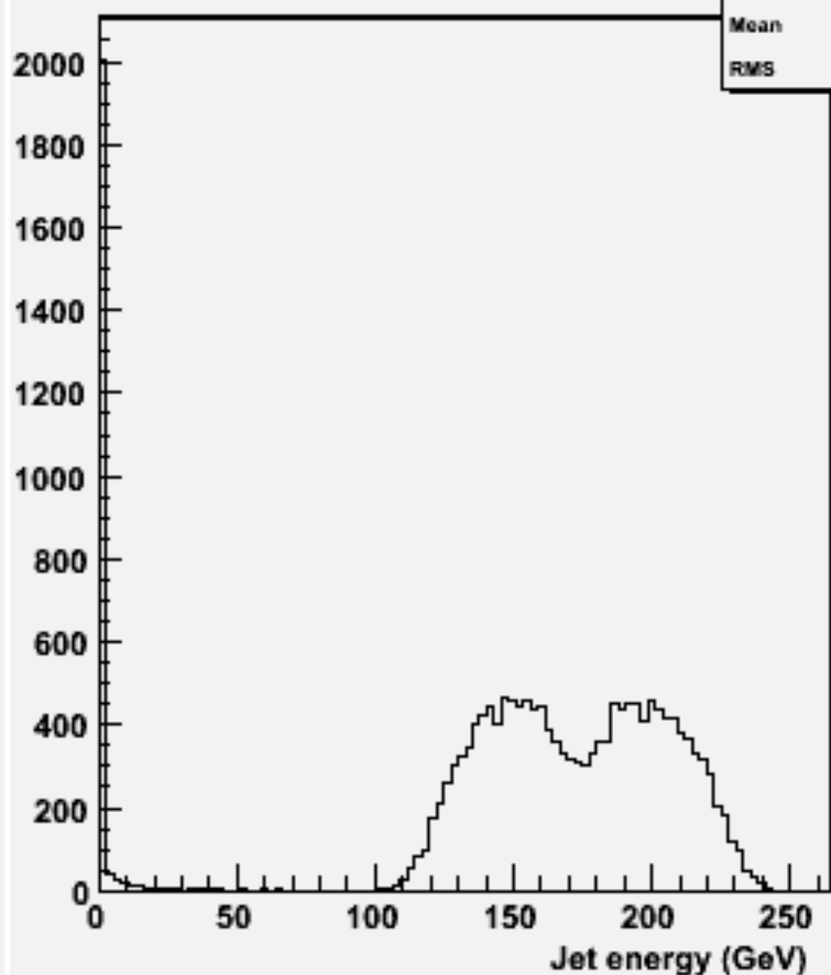
energy for 2-jets :w102385 uussss_o
