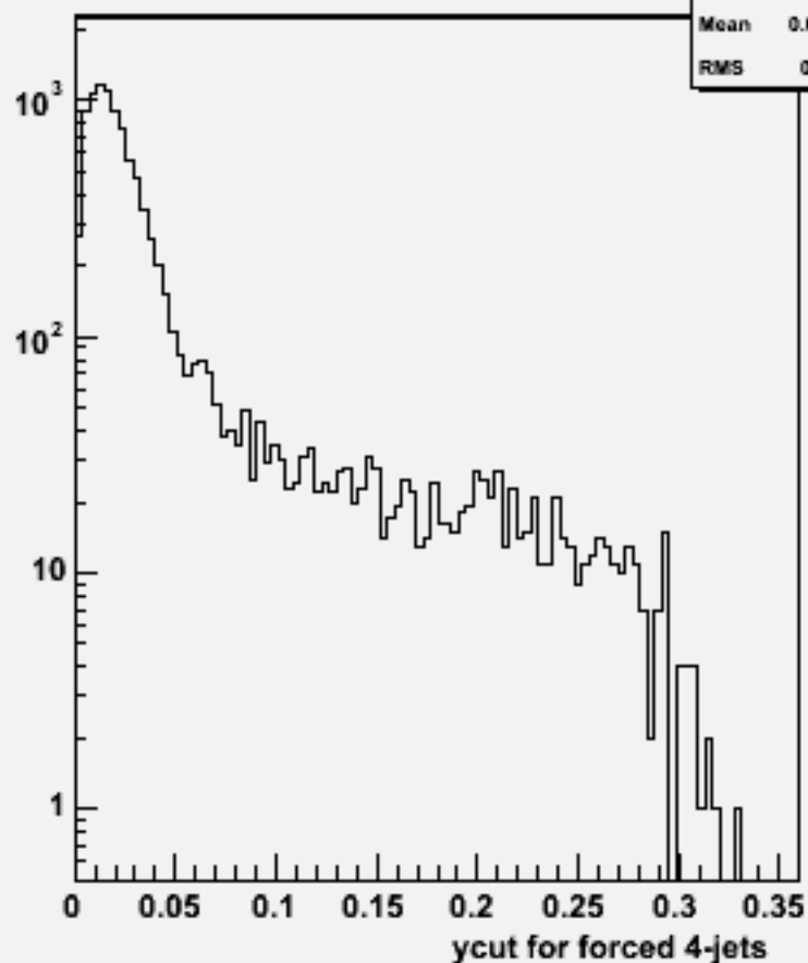
Ycut for 4-jets :w102385 uussss_o
