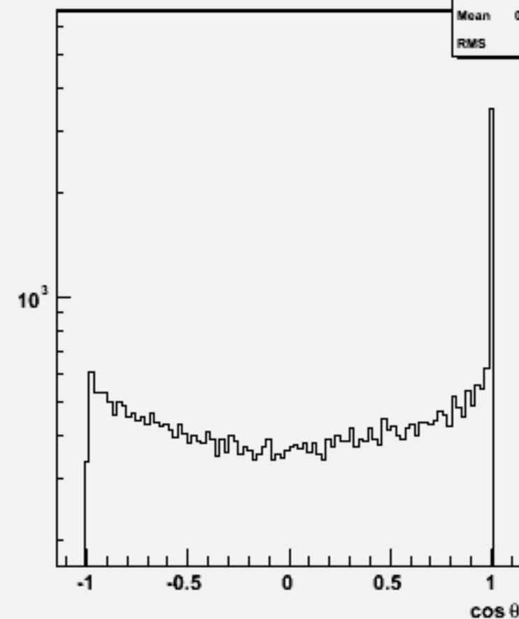
Jet cos \theta (All jets)w102384 uussss_o
