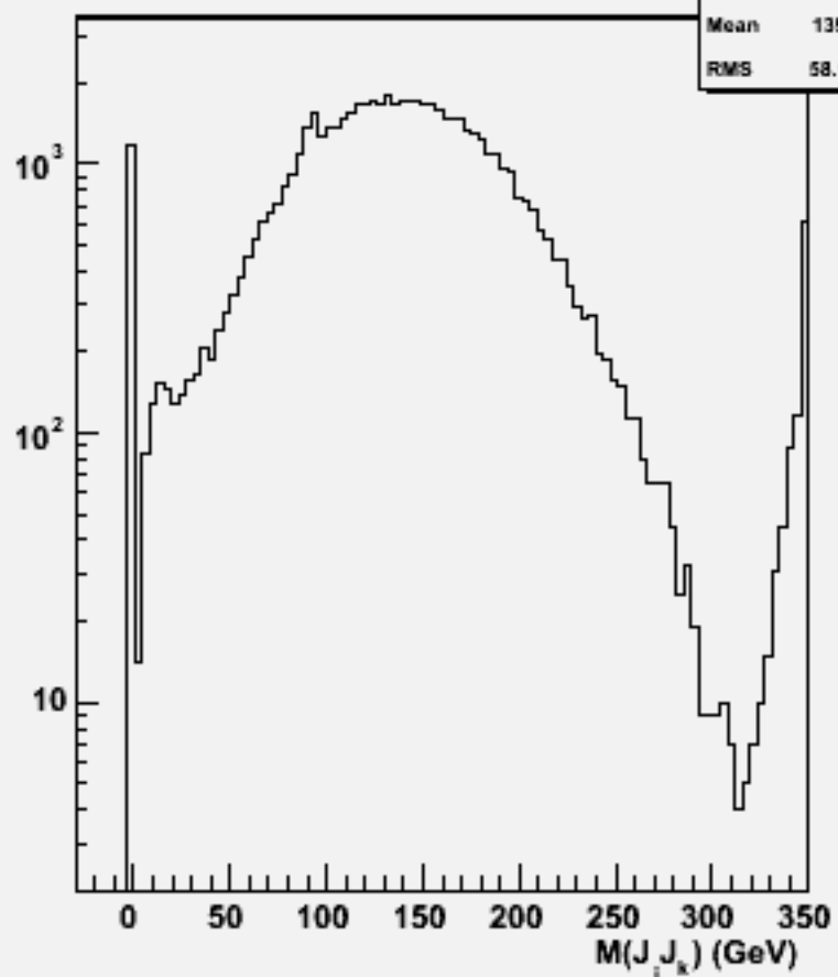
2jets mass(All comb)w102384 uussss_o
