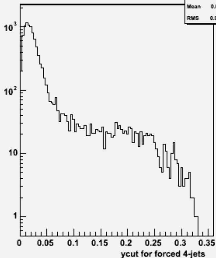
Ycut for 4-jets :w102384 uussss_o
