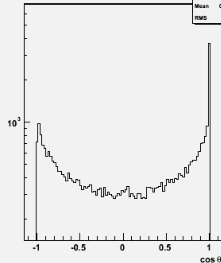
Jet cosθ (All jets)w102380 uue3e3bb_o
