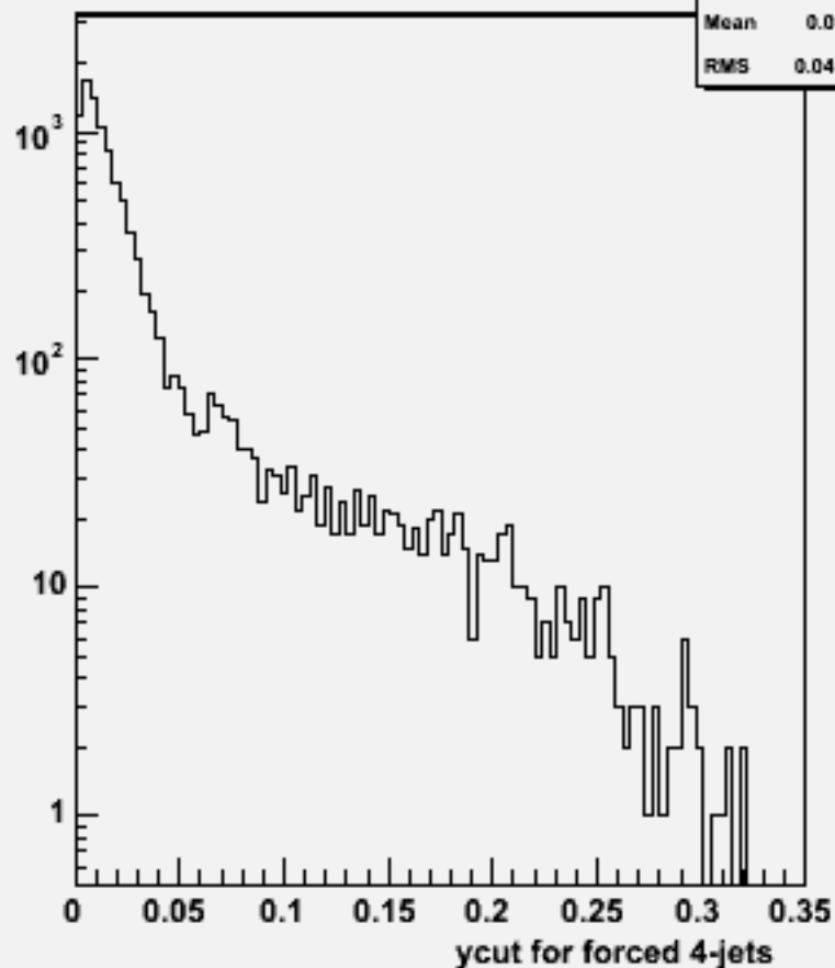
Ycut for 4-jets :w102380 uue3e3bb_o
