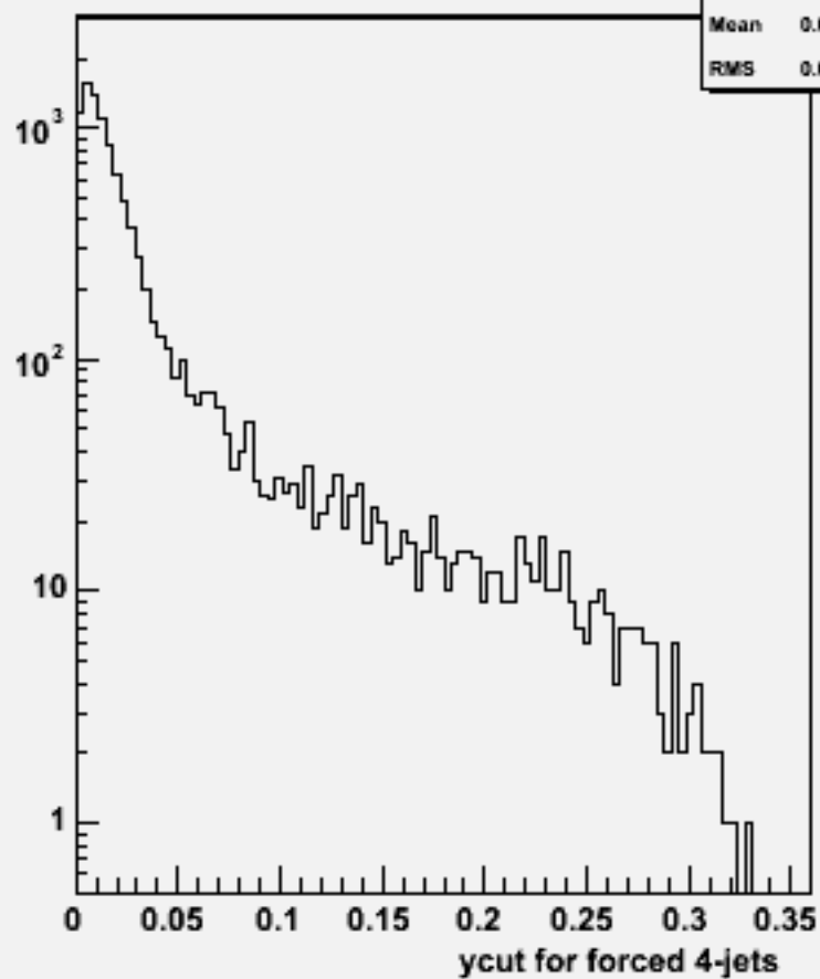
Ycut for 4-jets :w102369 uue2e2bb_o
