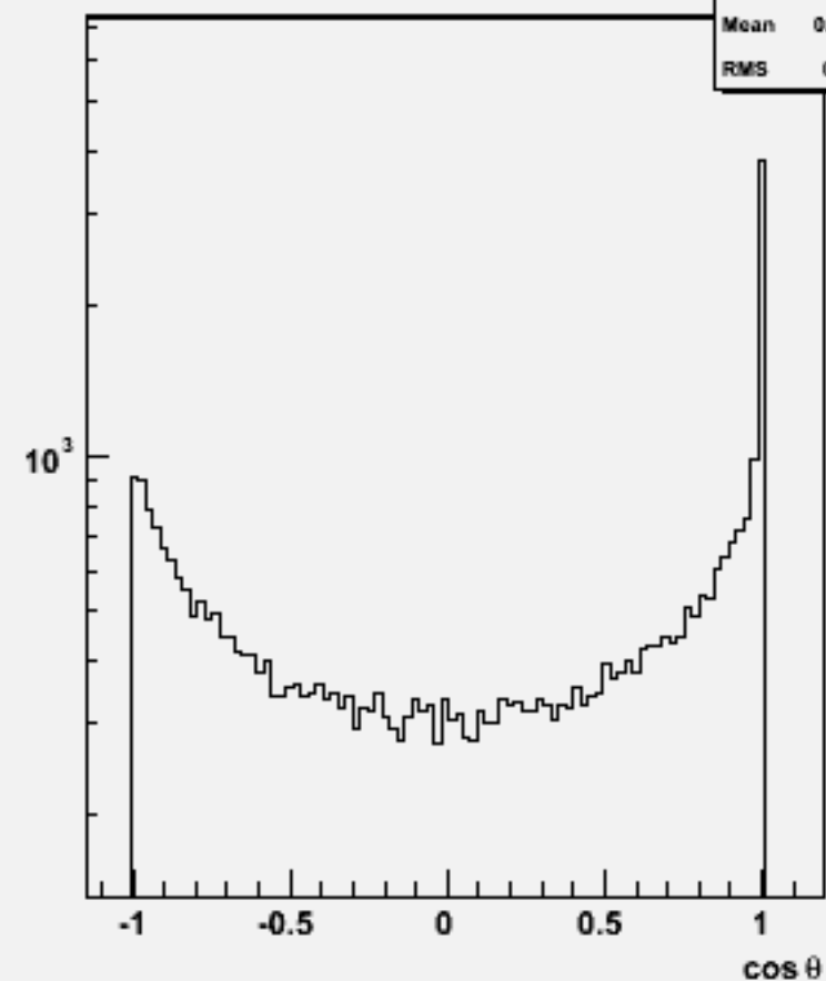
Jet cosθ (All jets)w102364 uue2e2ss_o
