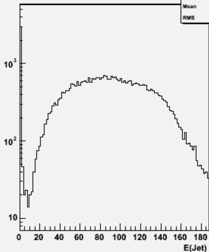
Jet energies(All jets)w102364 uue2e2ss_o
