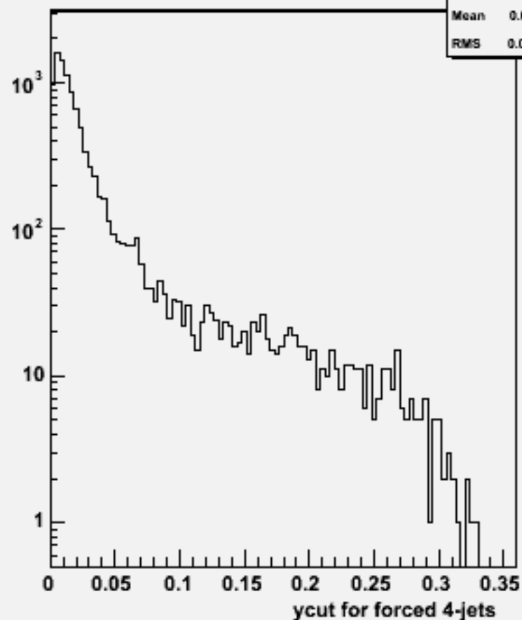
Ycut for 4-jets :w102364 uue2e2ss_o
