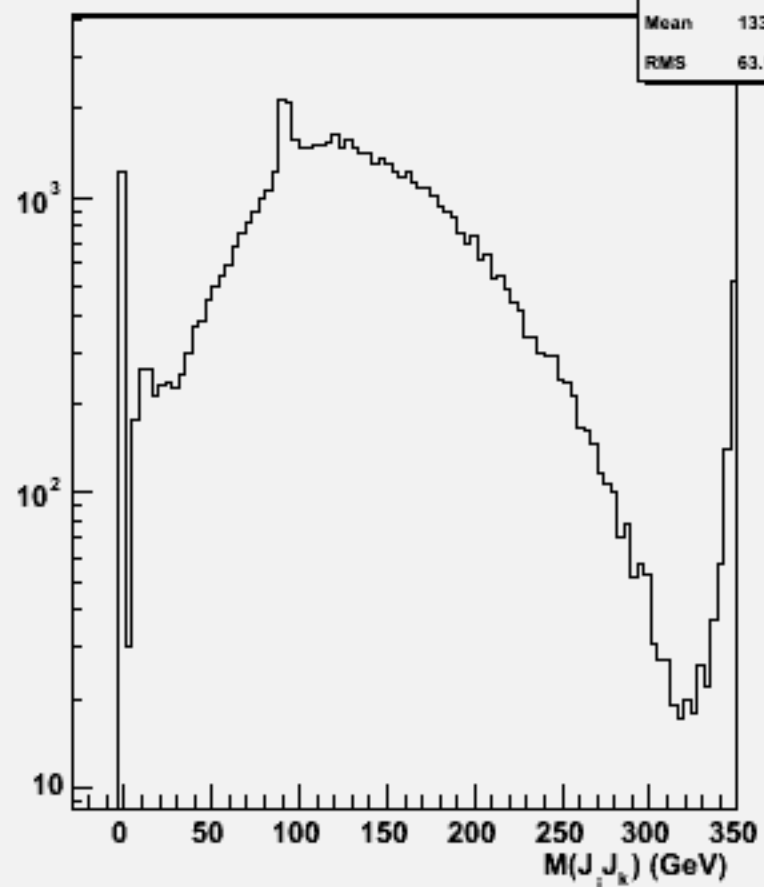
2jets mass(All comb)w102364 uue2e2ss_o
