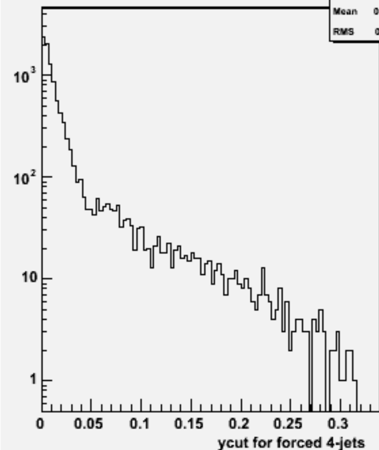
Ycut for 4-jets :w102361 uue2e2e3e3_o
