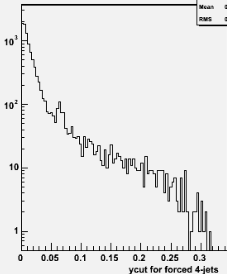
Ycut for 4-jets :w102356 uue2e2e2e2_o
