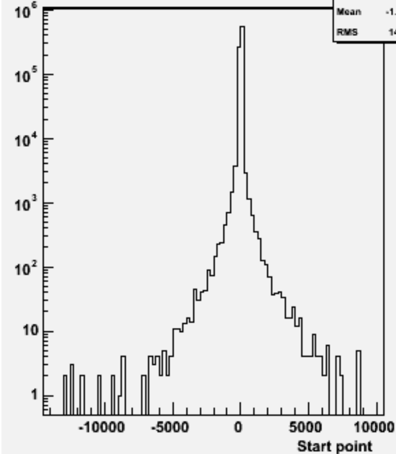
Start point Z : w102354 uue1e1bb_o
