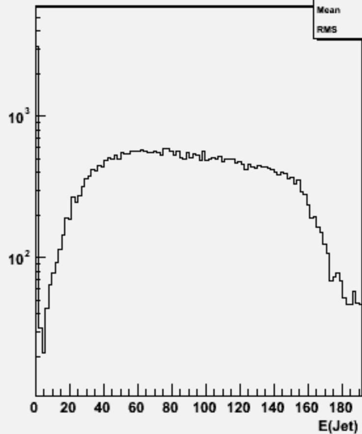
Jet energies(All jets)w102354 uue1e1bb_o
