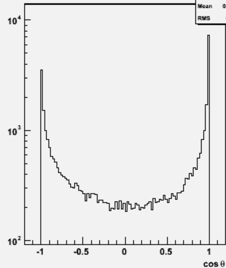
Jet cos \theta (All jets)w102354 uue1e1bb_o
