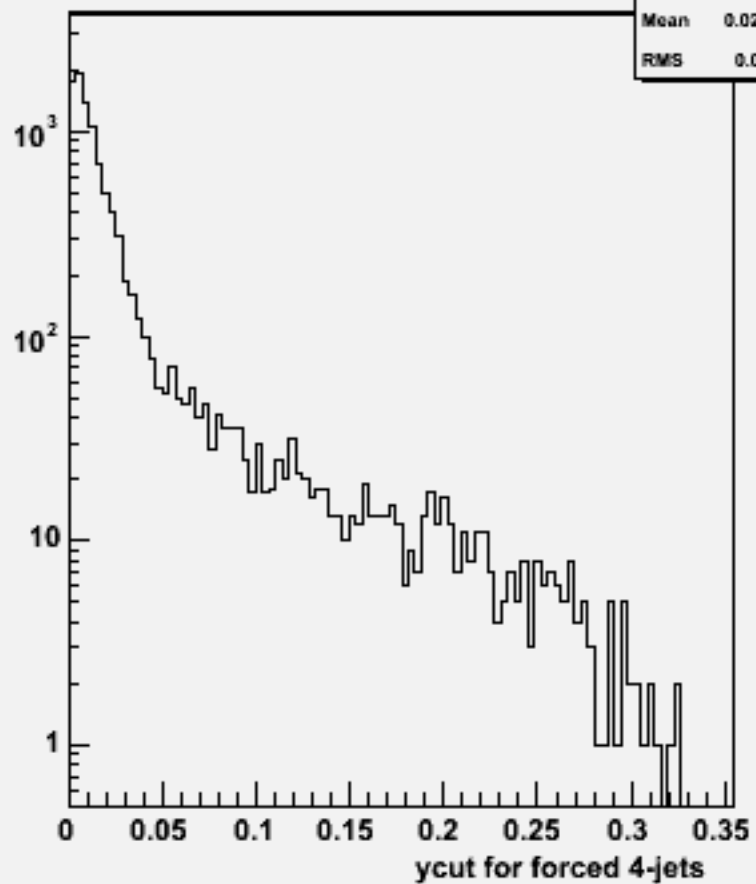
Ycut for 4-jets :w102354 uue1e1bb_o
