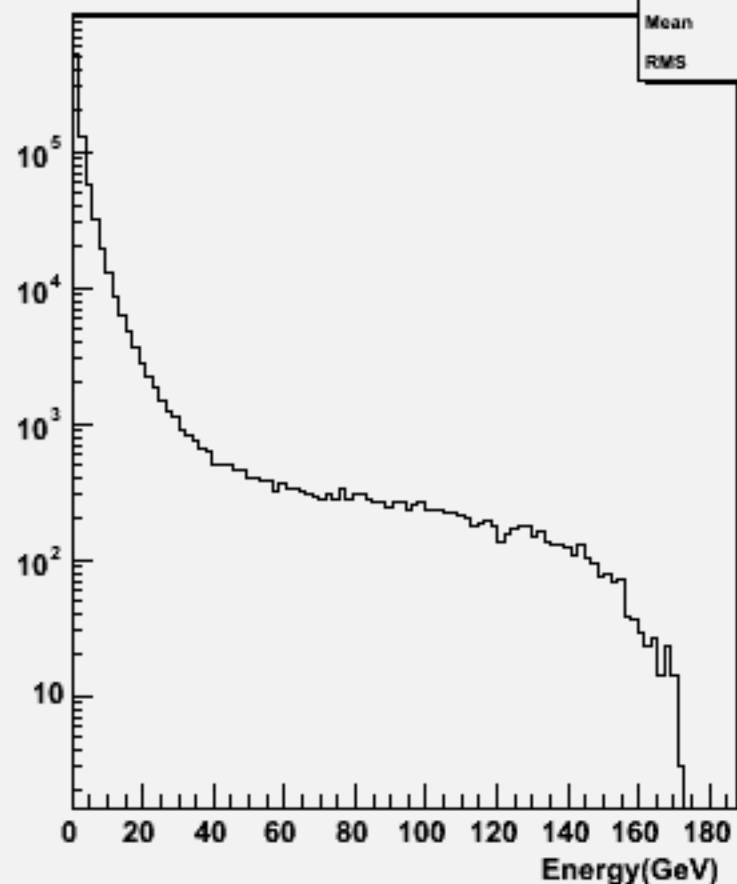
Particle Energy : w102354 uue1e1bb_o
