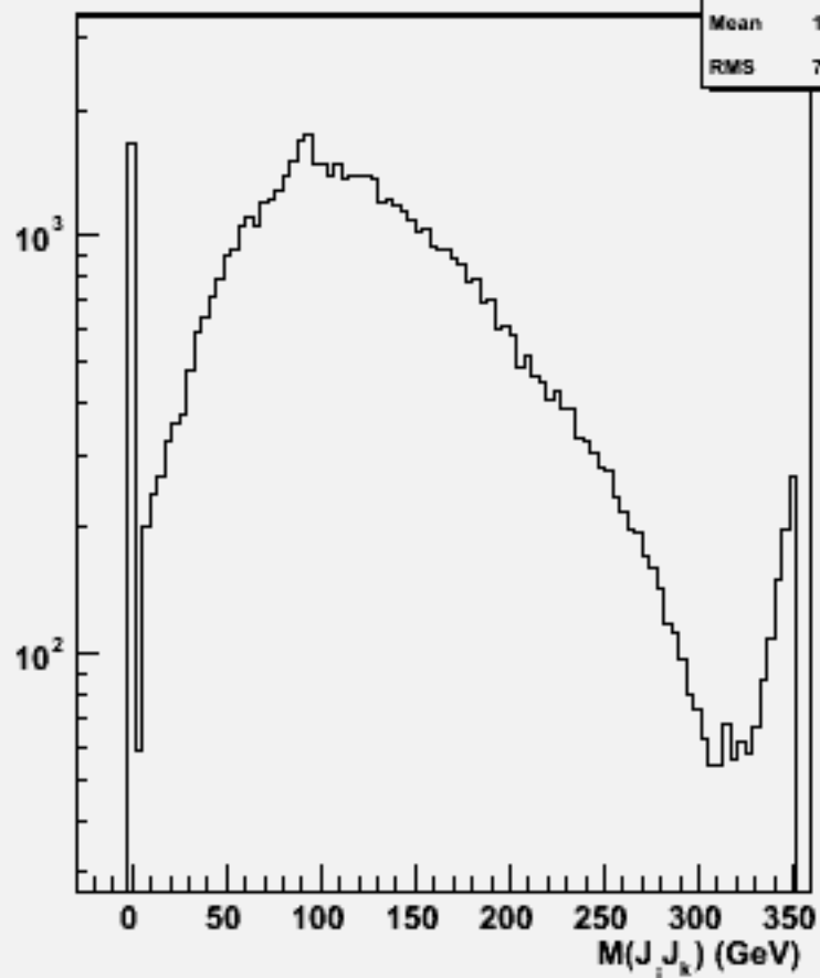
2jets mass(All comb)w102354 uue1e1bb_o
