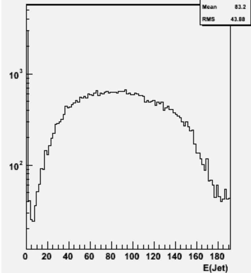
Jet energies(All jets)w102353 uue1e1bb_o
