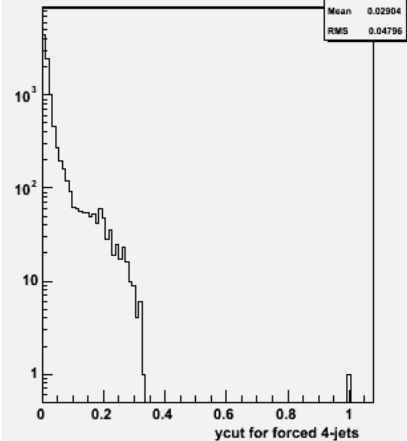
Ycut for 4-jets :w102353 uue1e1bb_o
