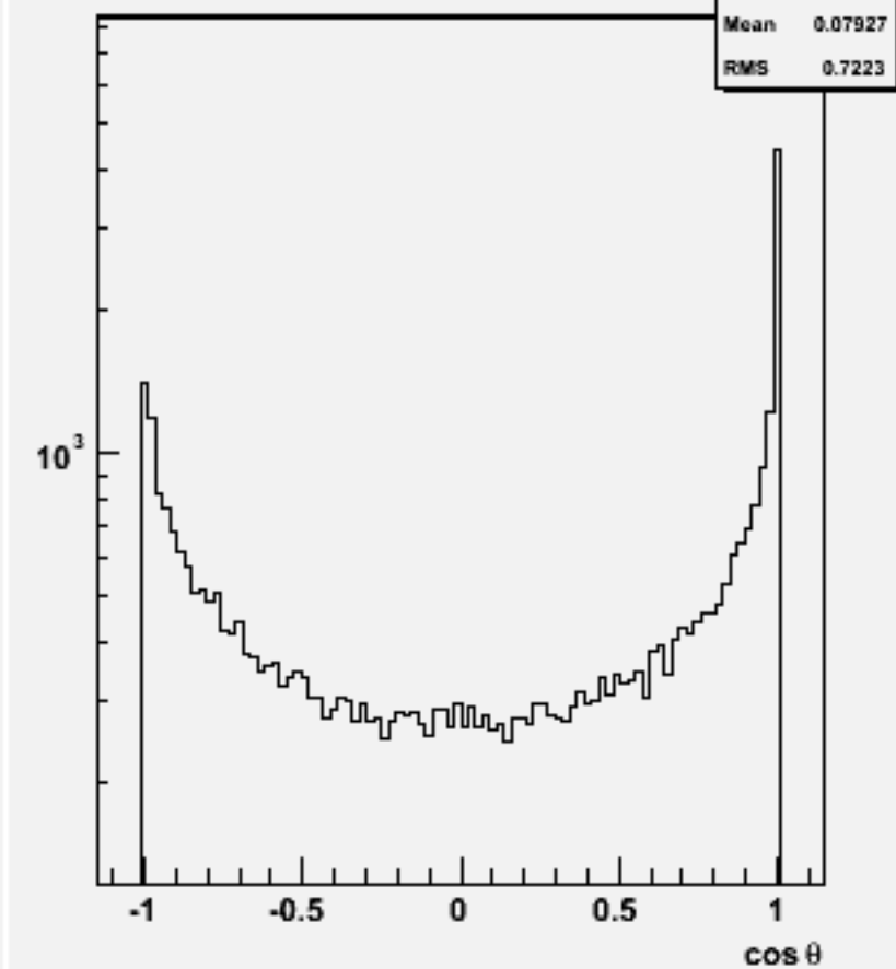
Jet cosθ (All jets)w102353 uue1e1bb_o
