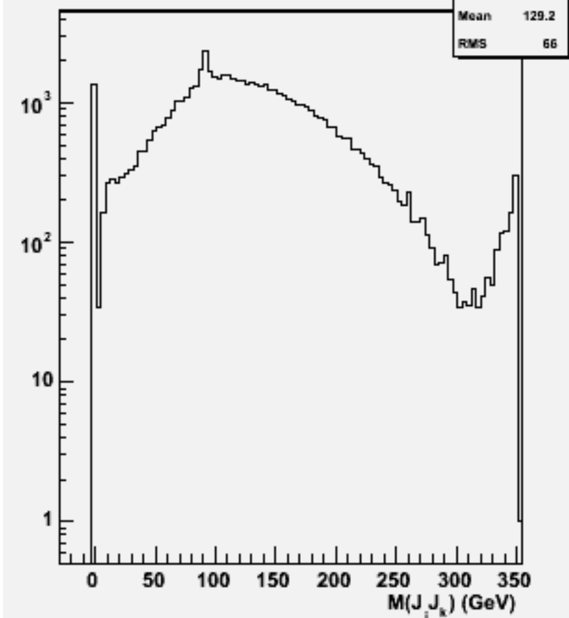
2jets mass(All comb)w102353 uue1e1bb_o
