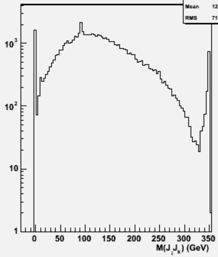
2jets mass(All comb)w102350 uue1e1ss_o
