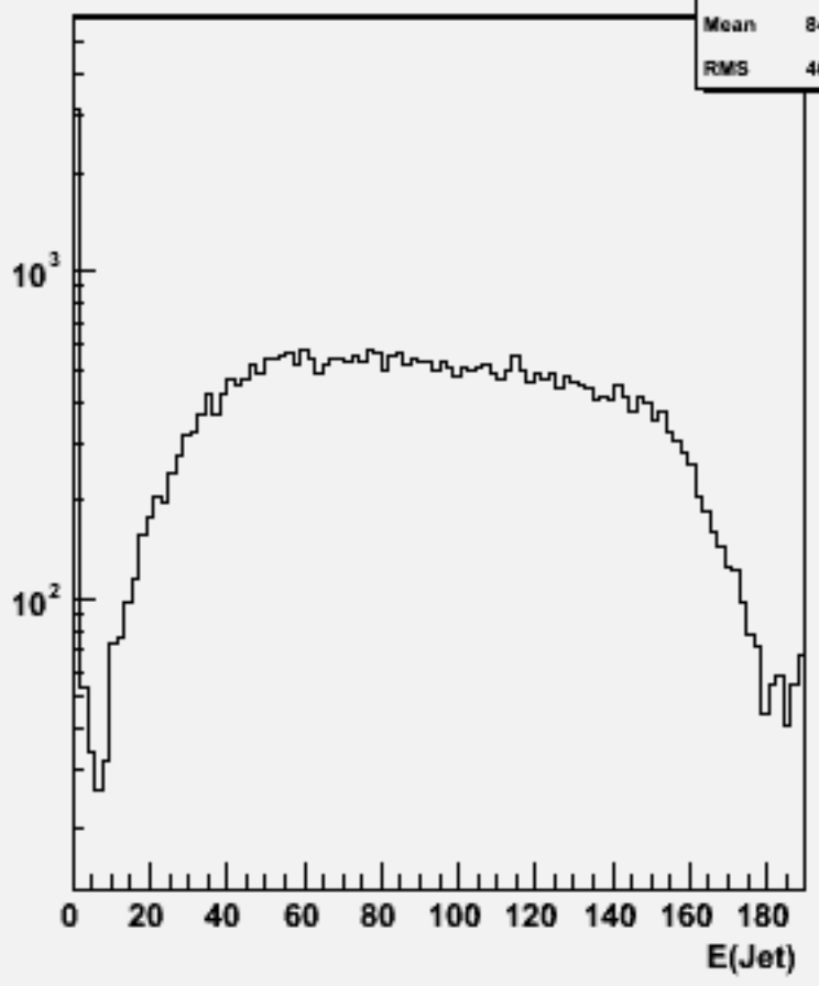
Jet energies(All jets)w102350 uue1e1ss_o
