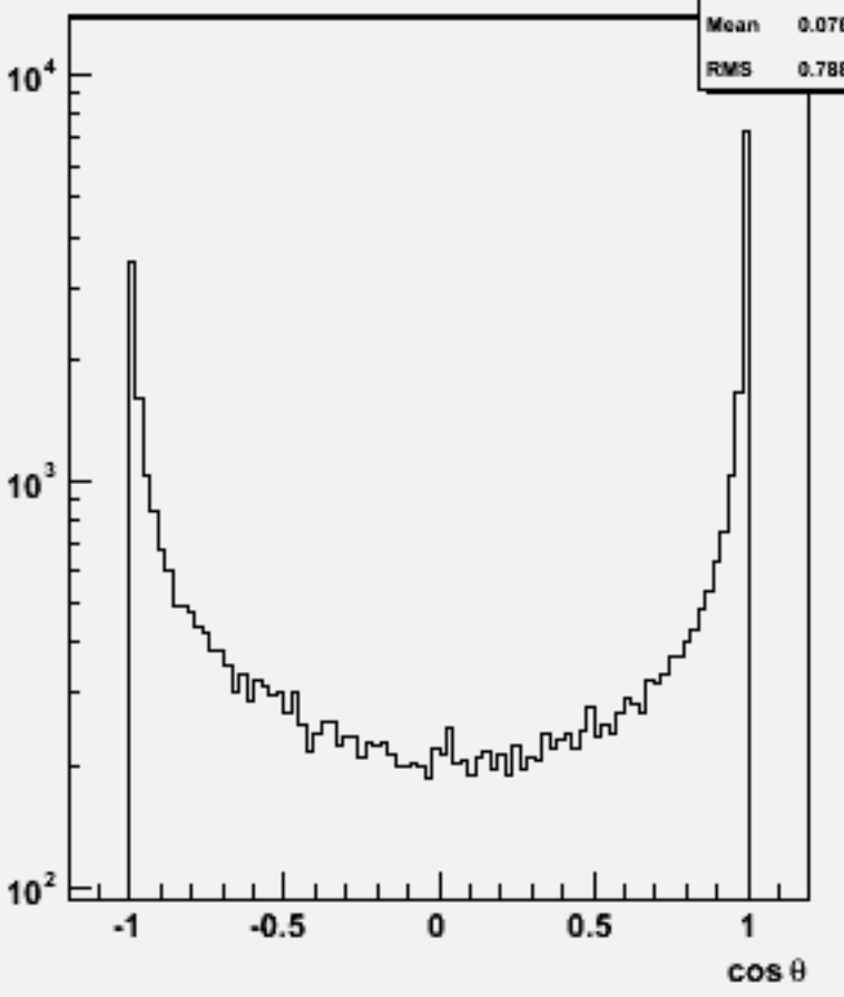
Jet cosθ (All jets)w102350 uue1e1ss_o
