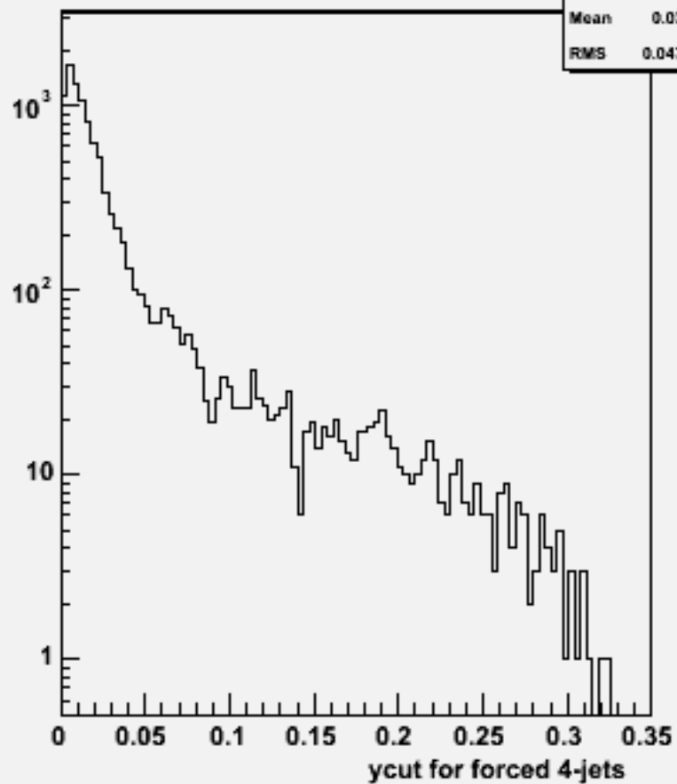
Ycut for 4-jets :w102349 uue1e1ss_o
