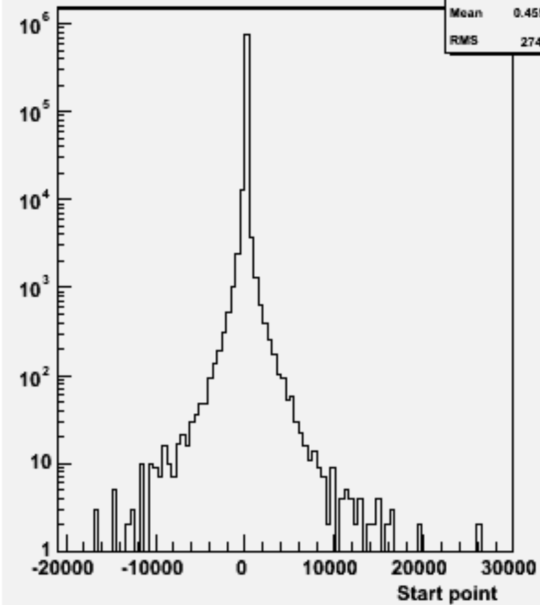
Start point Z : w102349 uue1e1ss_o
