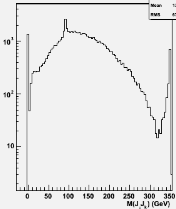
2jets mass(All comb)w102349 uue1e1ss_o
