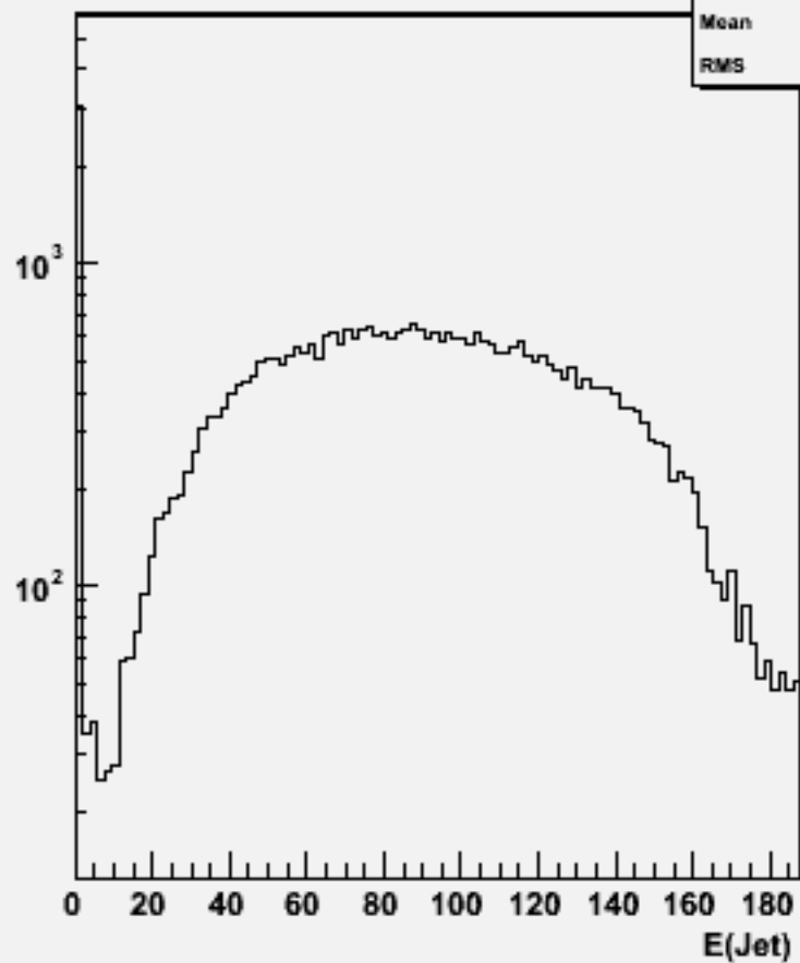
Jet energies(All jets)w102349 uue1e1ss_o
