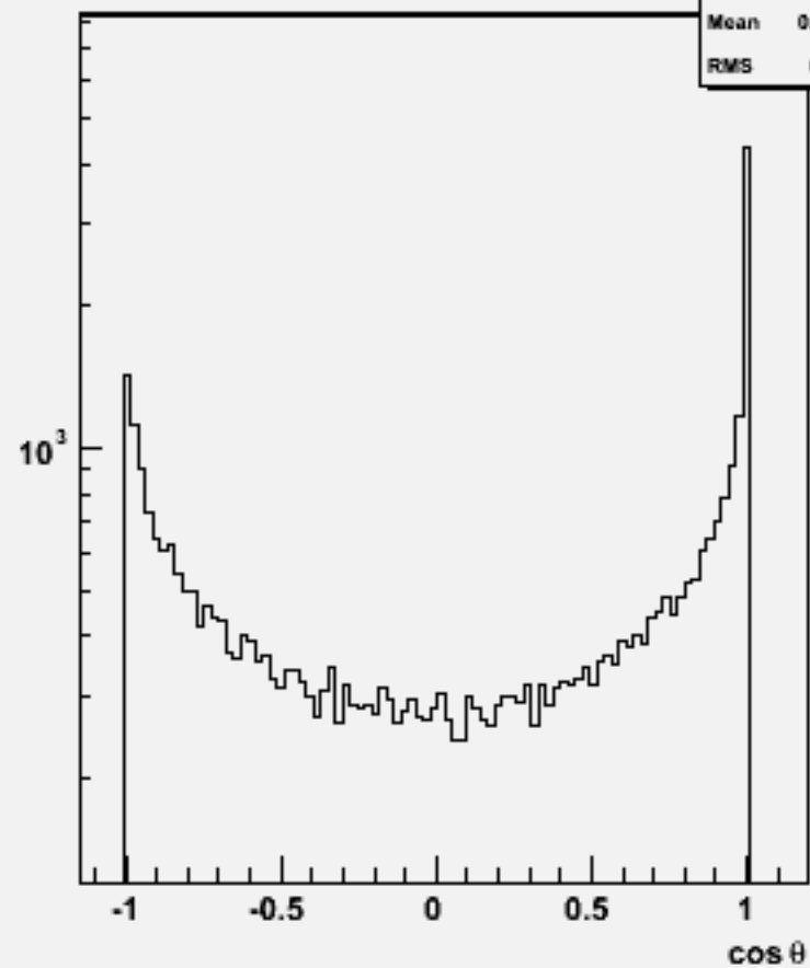
Jet cosθ (All jets)w102349 uue1e1ss_o
