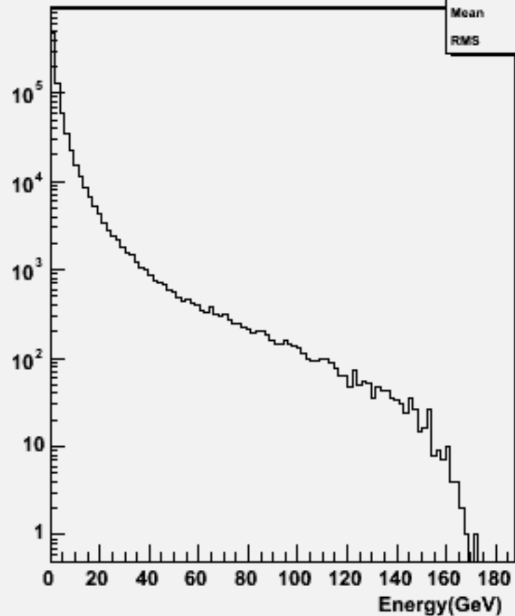
Particle Energy : w102349 uue1e1ss_o
